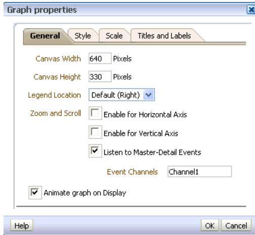
Figure 3–20 Setting up to Listen to Master -Detail Events
