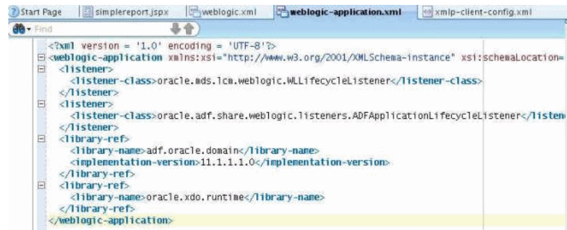
Figure 9–13 Example weblogic-application.xml
