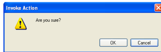
Figure 8–13 Confirmation Dialog
