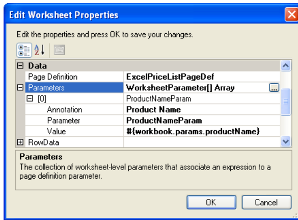
Figure 14–4 Worksheet Parameters
