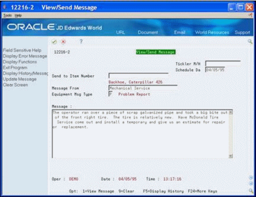
Figure 6-4 View/Send Message screen
