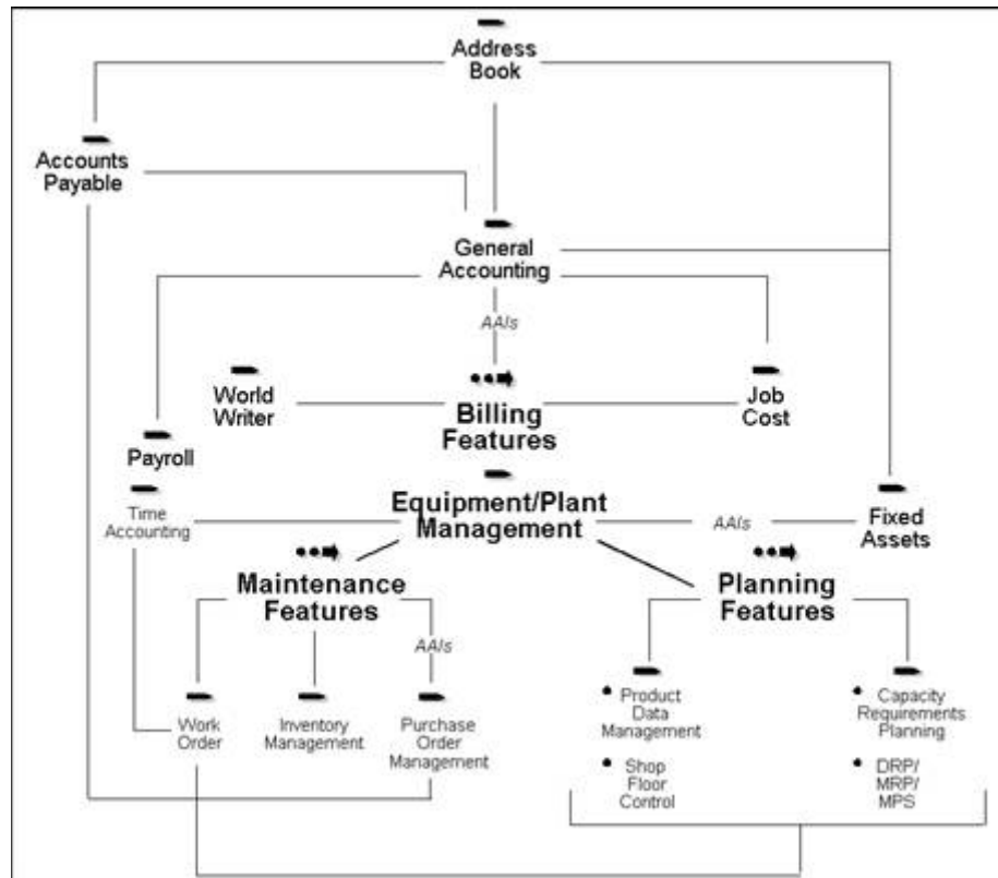
Figure 1–1 Integration Between Equipment Billing and other JD Edwards World systems
