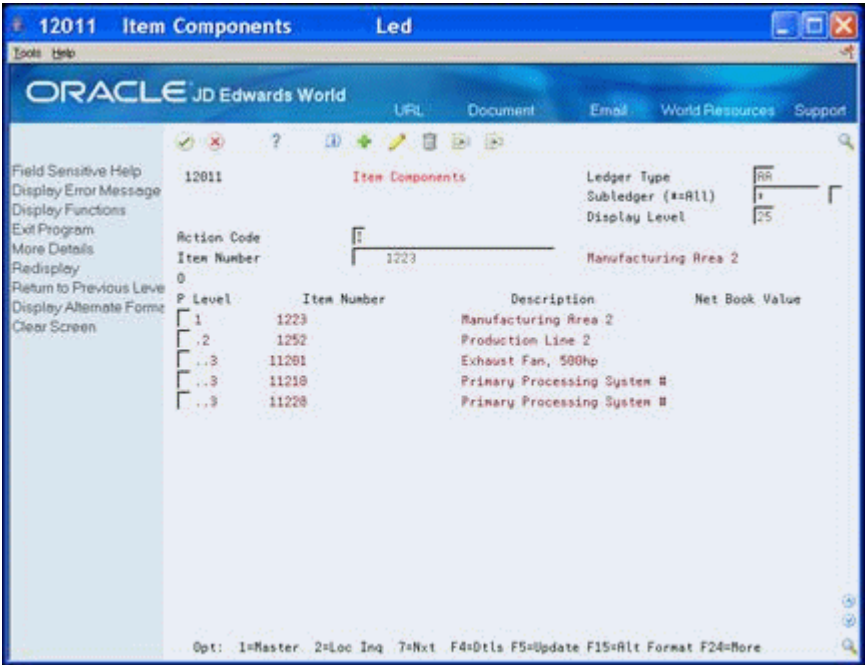
Figure 7-3 Item Components screen
