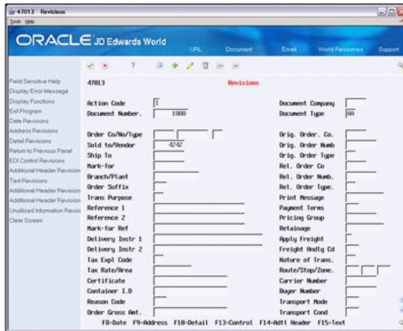
Figure 19–1 Revisions screen
