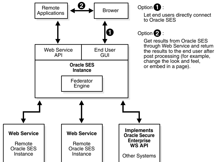
Figure 1-4 Federation Architecture
