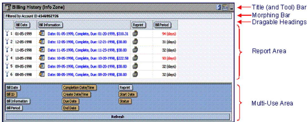
Figure 13: Info Zone Common Areas
