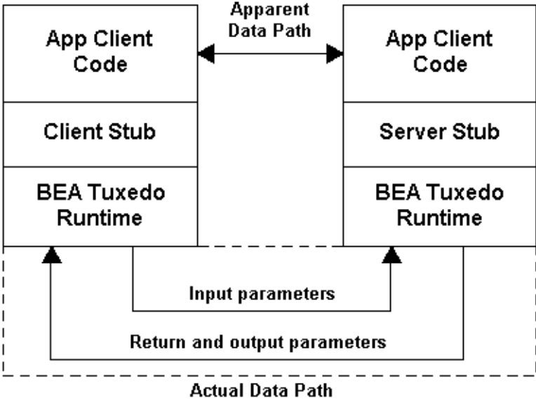
Figure 1-1 RPC Communication
