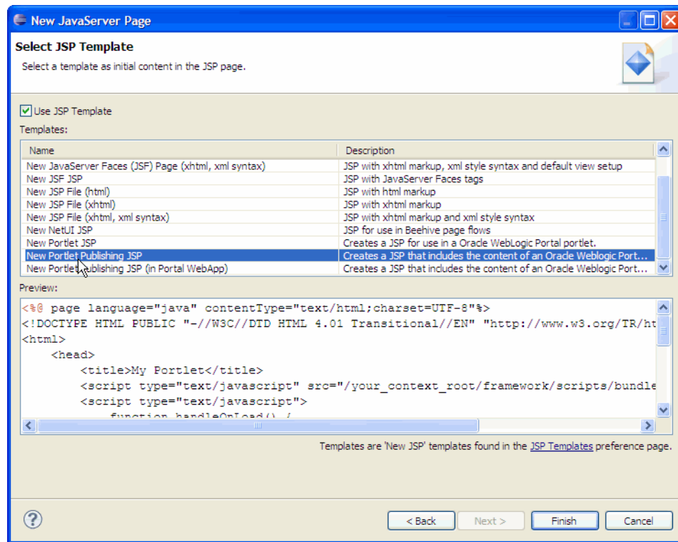
Figure 5–4 Select JSP Template Page Dialog in the New JavaServer Page Wizard
