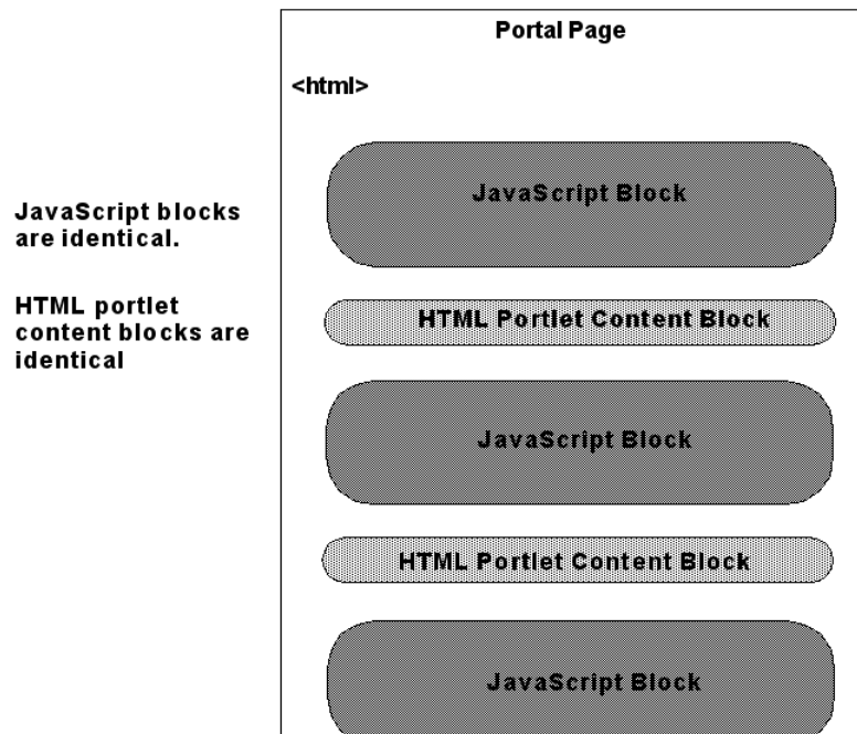
Figure 5–3 Portlet Publishing and WSRP
