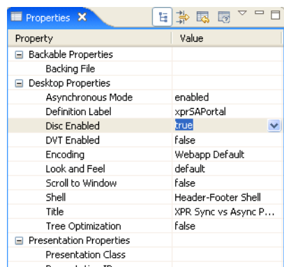
Figure 3–2 Enabling Disc in Oracle Enterprise Pack for Eclipse
