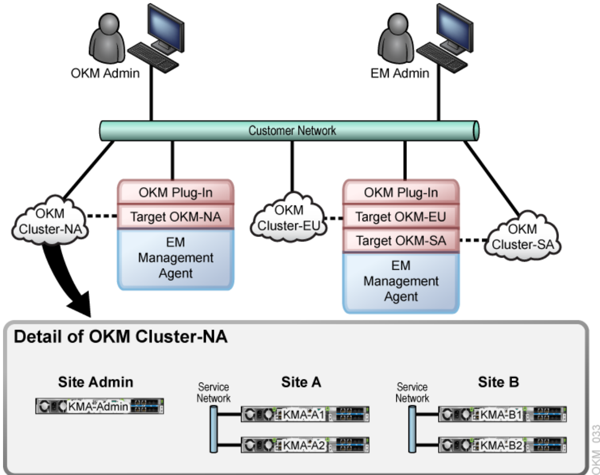
Figure 1–1 Large Enterprise Plug-in Deployment Example
