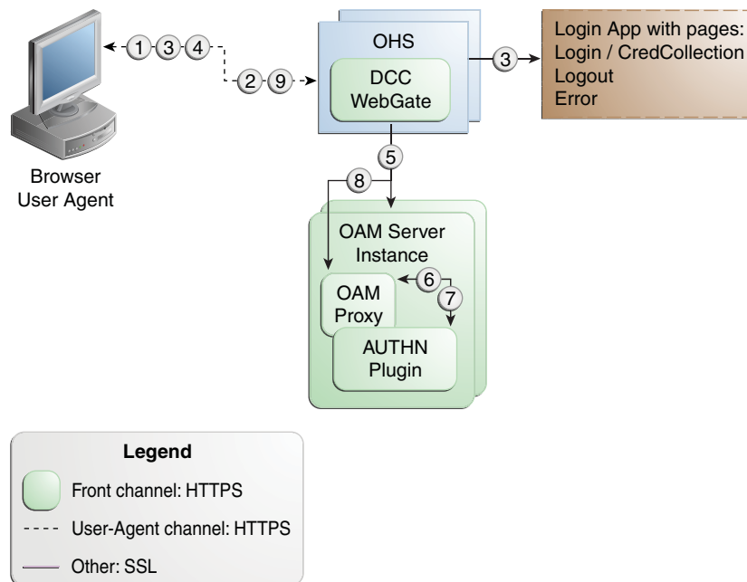
Figure 15–6 Combined DCC and Webgate Configuration
