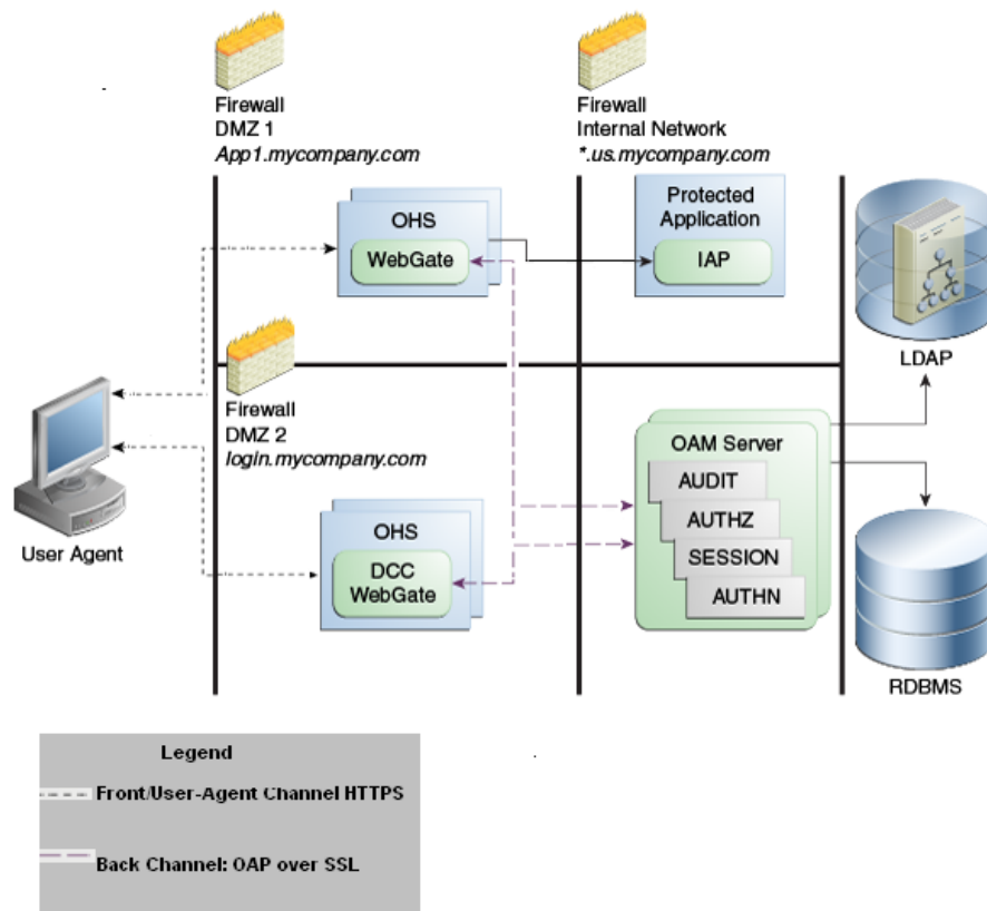
Figure 15-5 Example: Separate Resource Webgate and DCC Webgate Deployment
