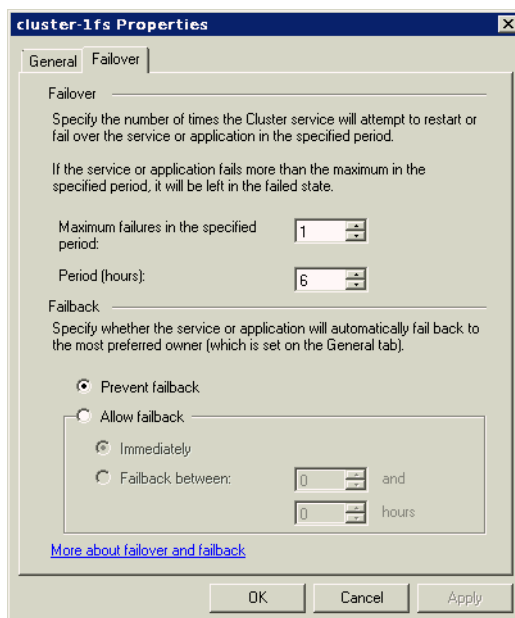
Figure 2–14 Group Failback Policy Property Page
