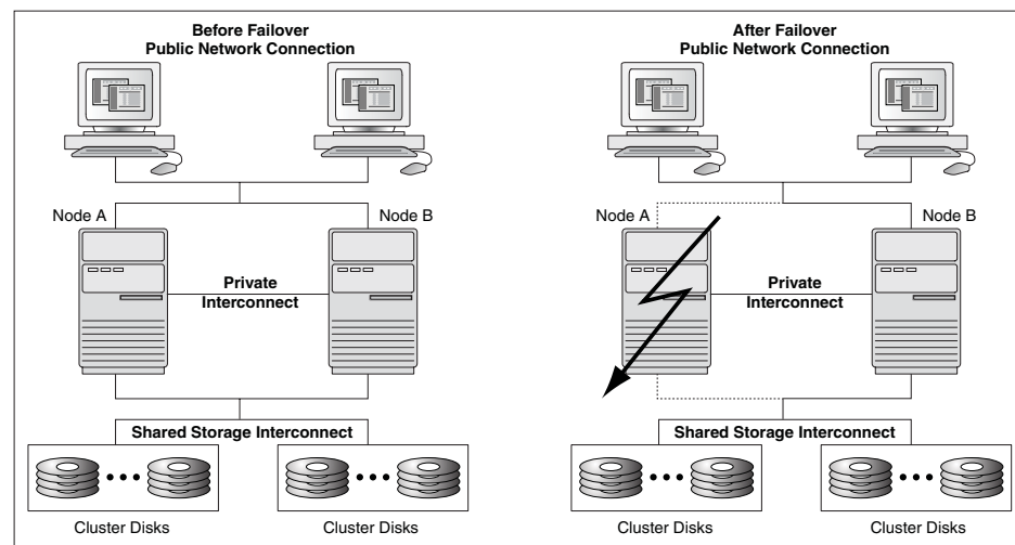
Figure 2–2 Shared-Nothing Configuration
