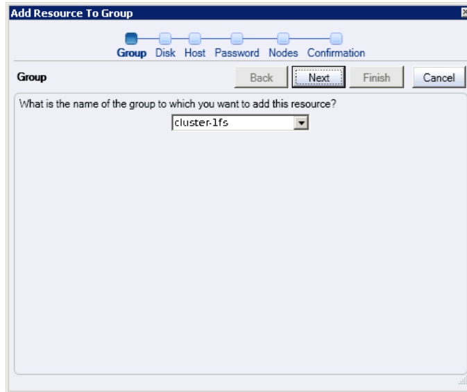
Figure 9–1 Add Resource to Group Wizard - Group Page
