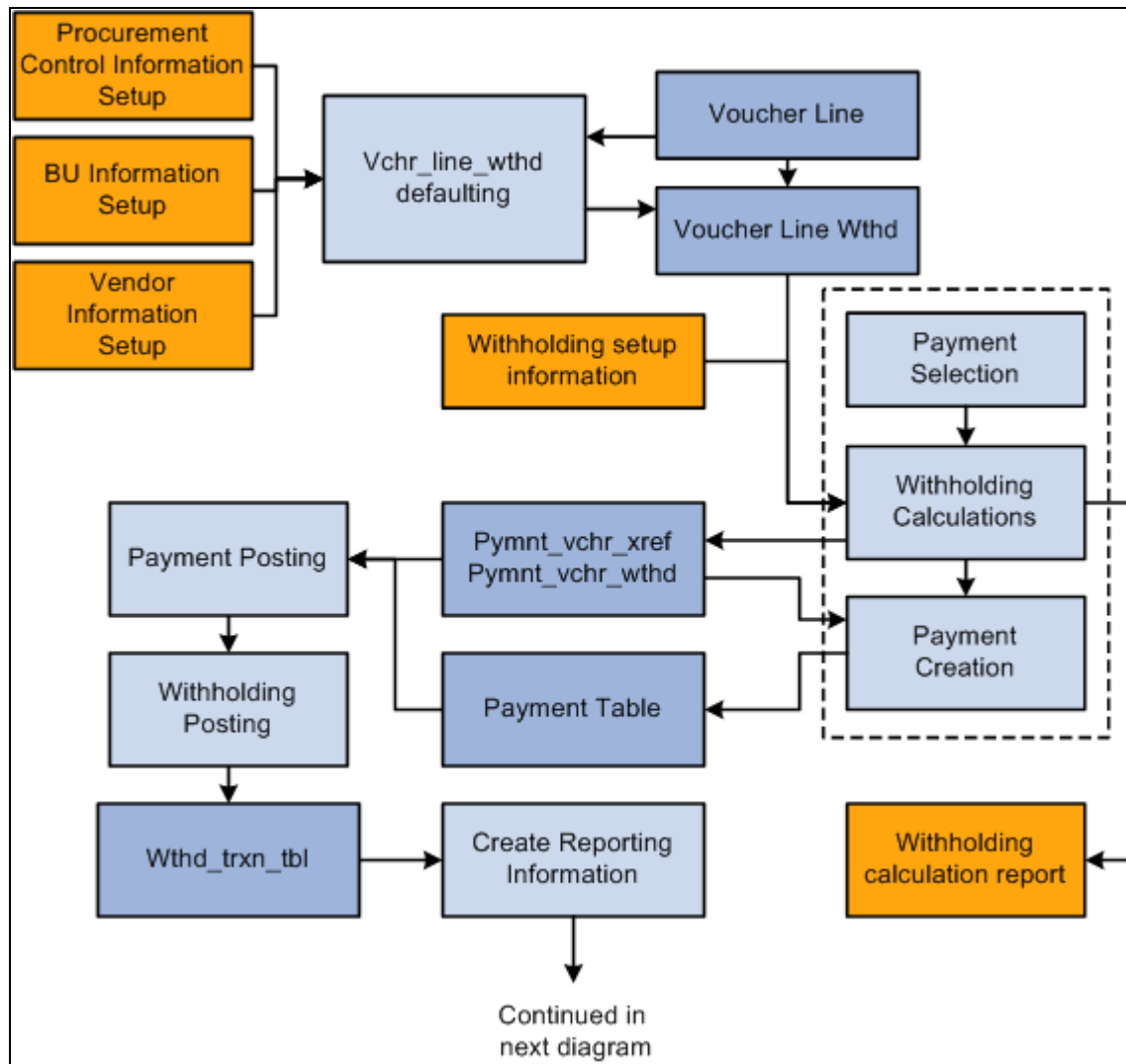
Withholding process flow (part 1)
