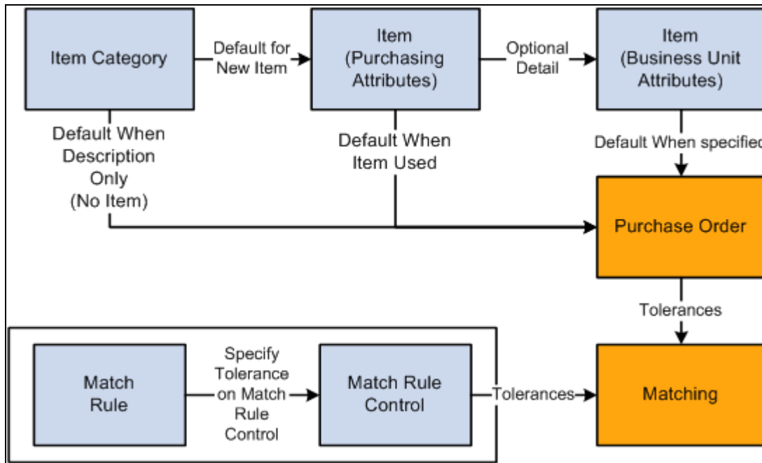
Matching tolerance defaults diagram
