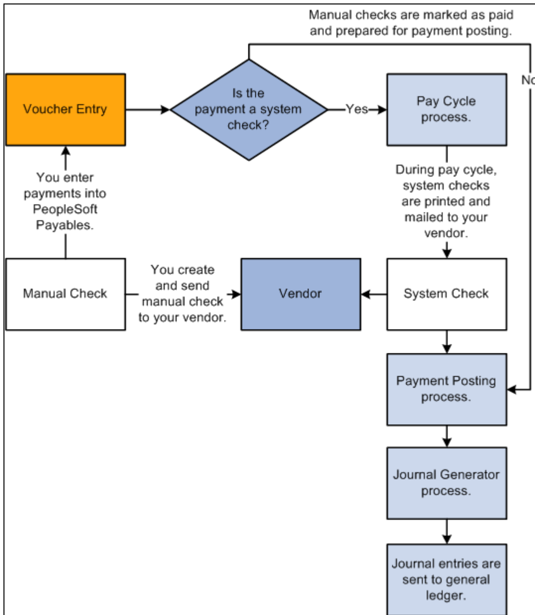
System and Manual Checks process flow
