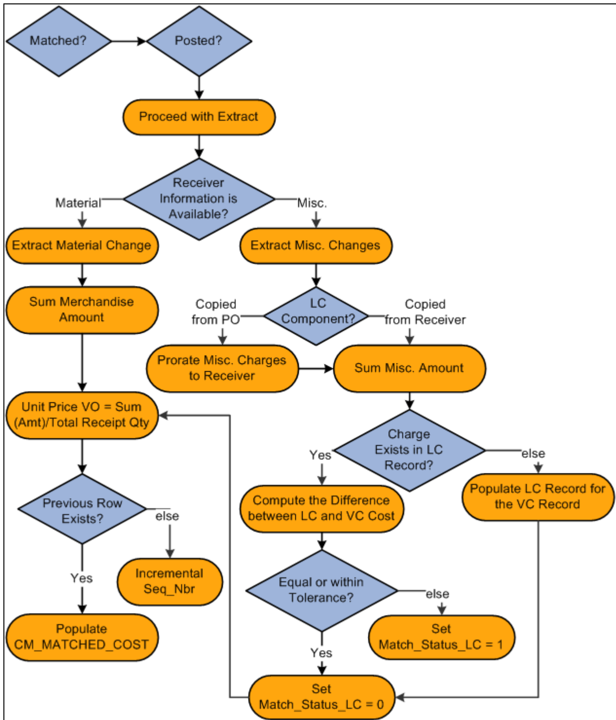
Landed Cost Extraction process
