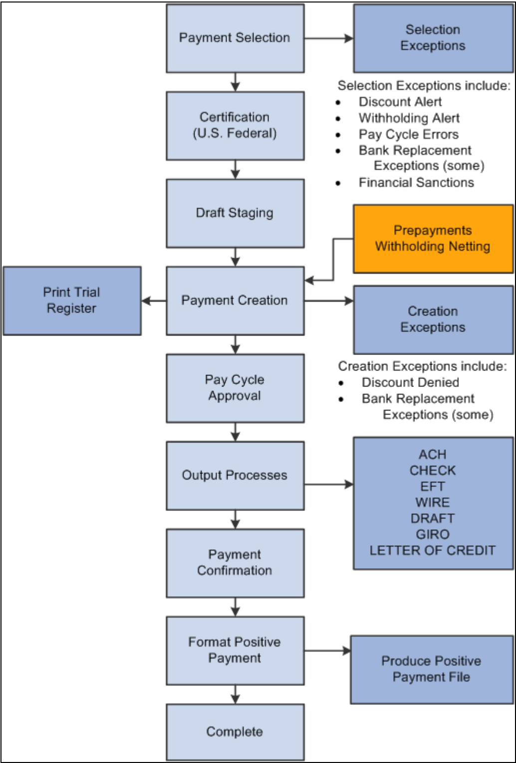
Pay cycle process flow
