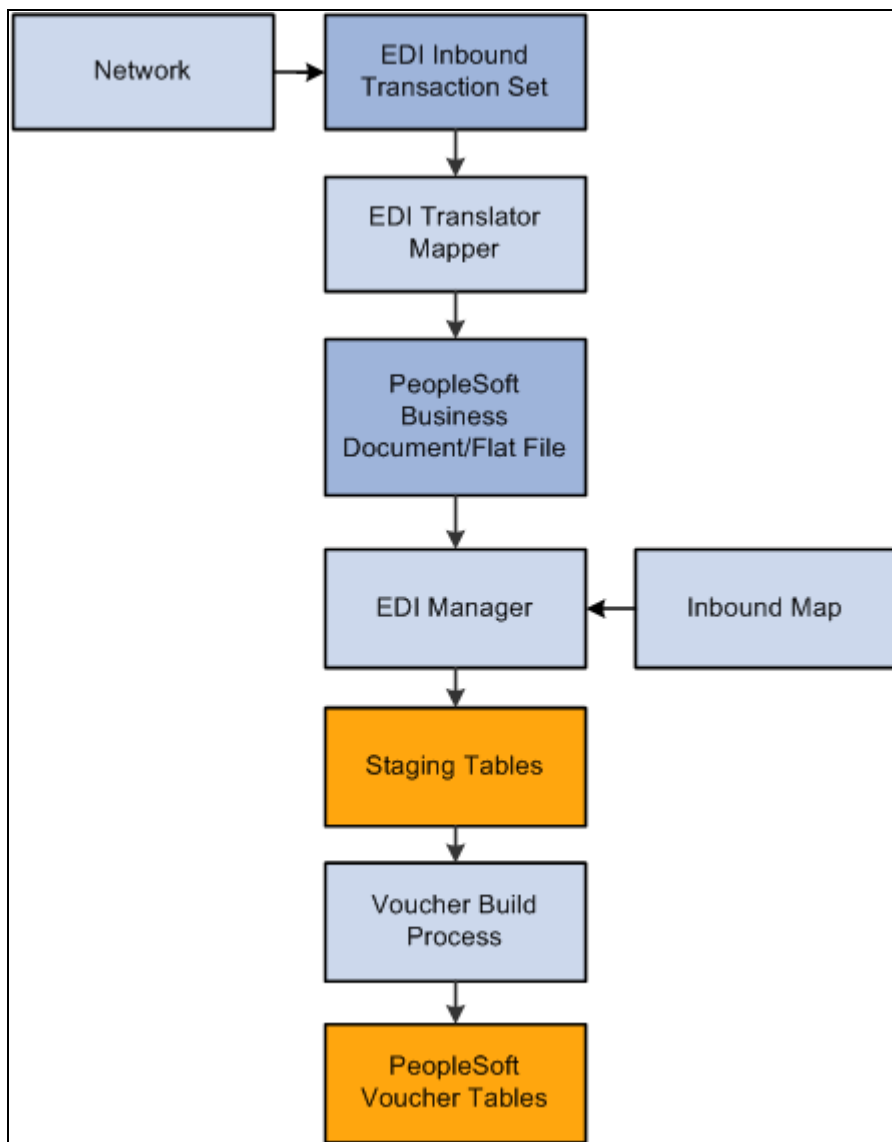
EDI Manager and Voucher Build process flow
