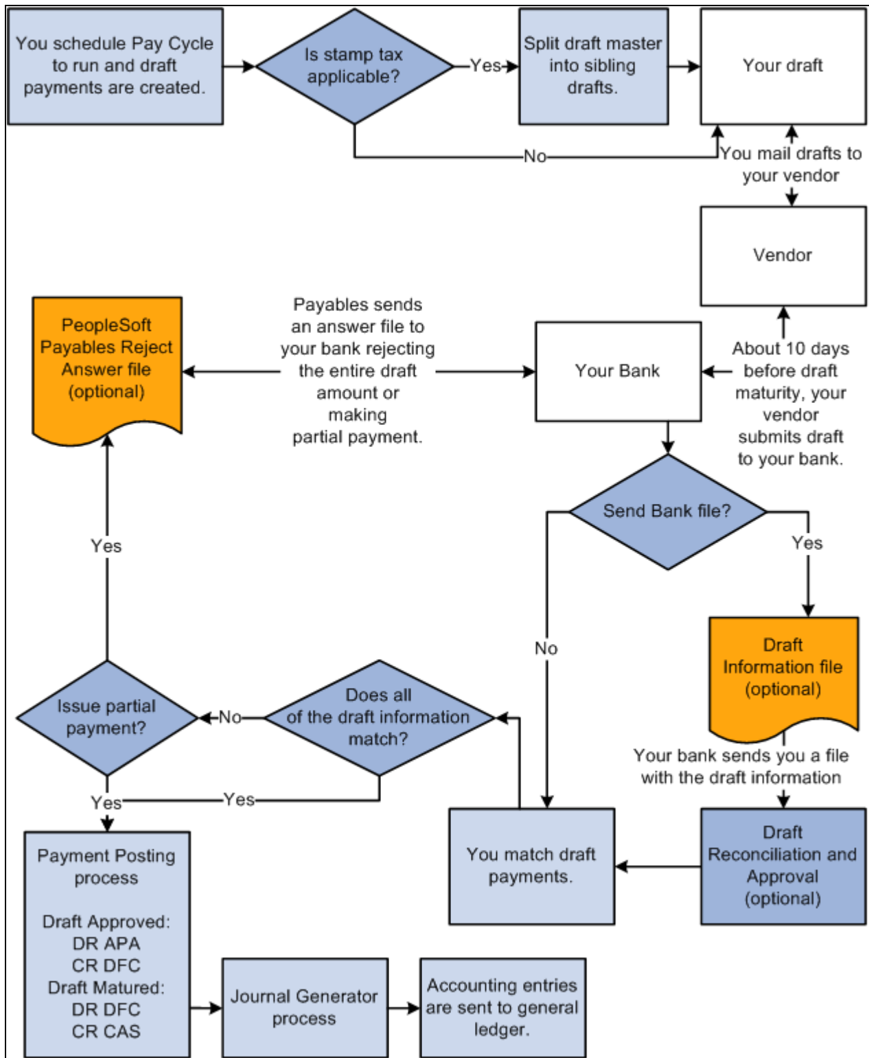
Customer-initiated Draft Payment process flow
