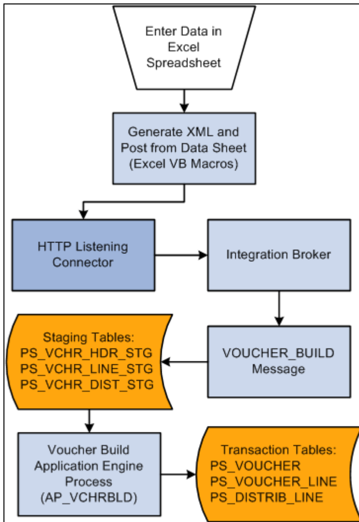
Spreadsheet voucher process flow
