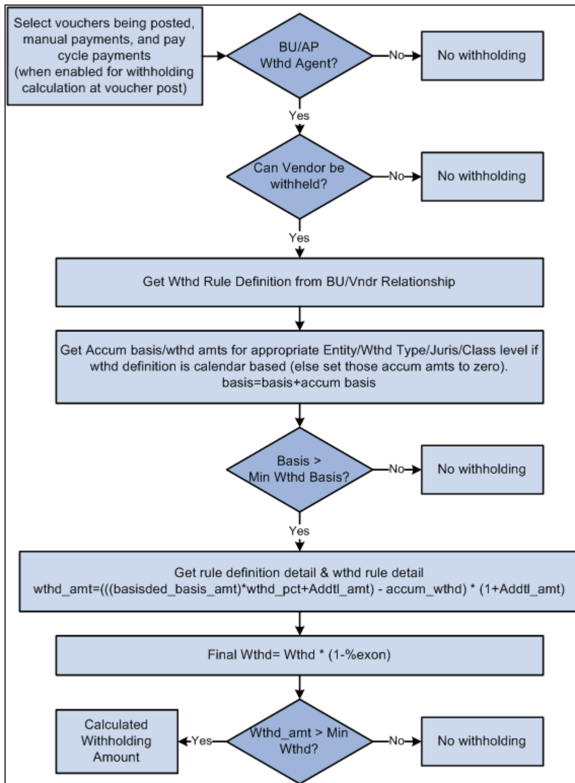
Withholding calculation process flow
