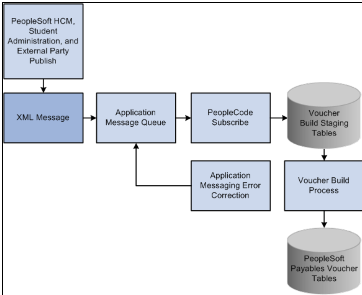
VOUCHER_BUILD message subscription inbound process flow
