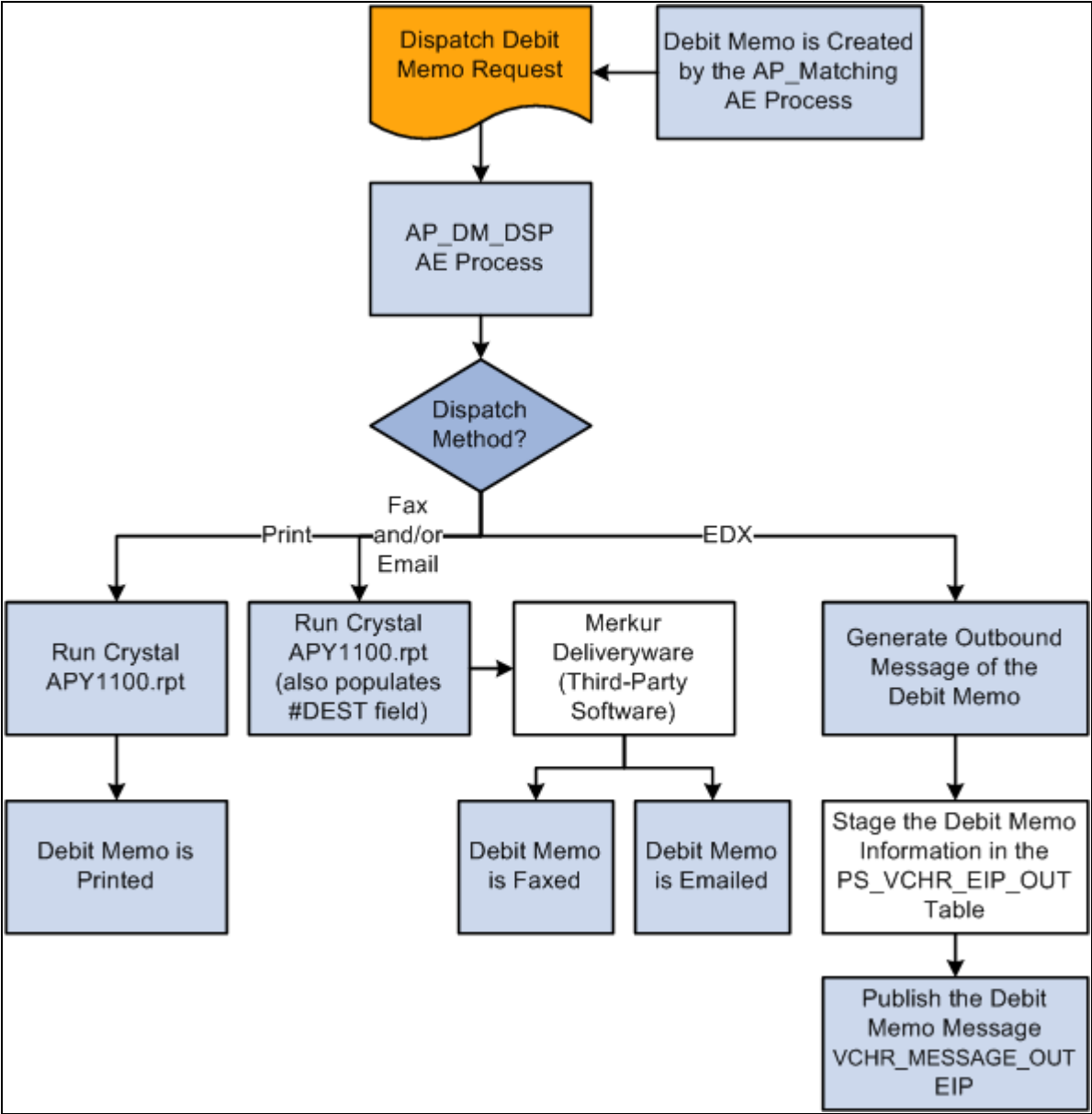
Debit memo notification process
