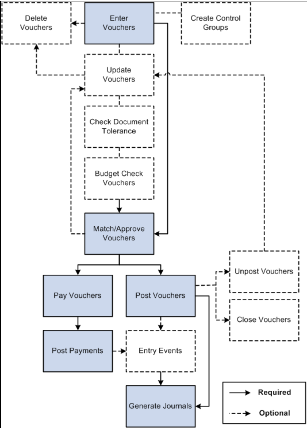
Voucher processing flow
