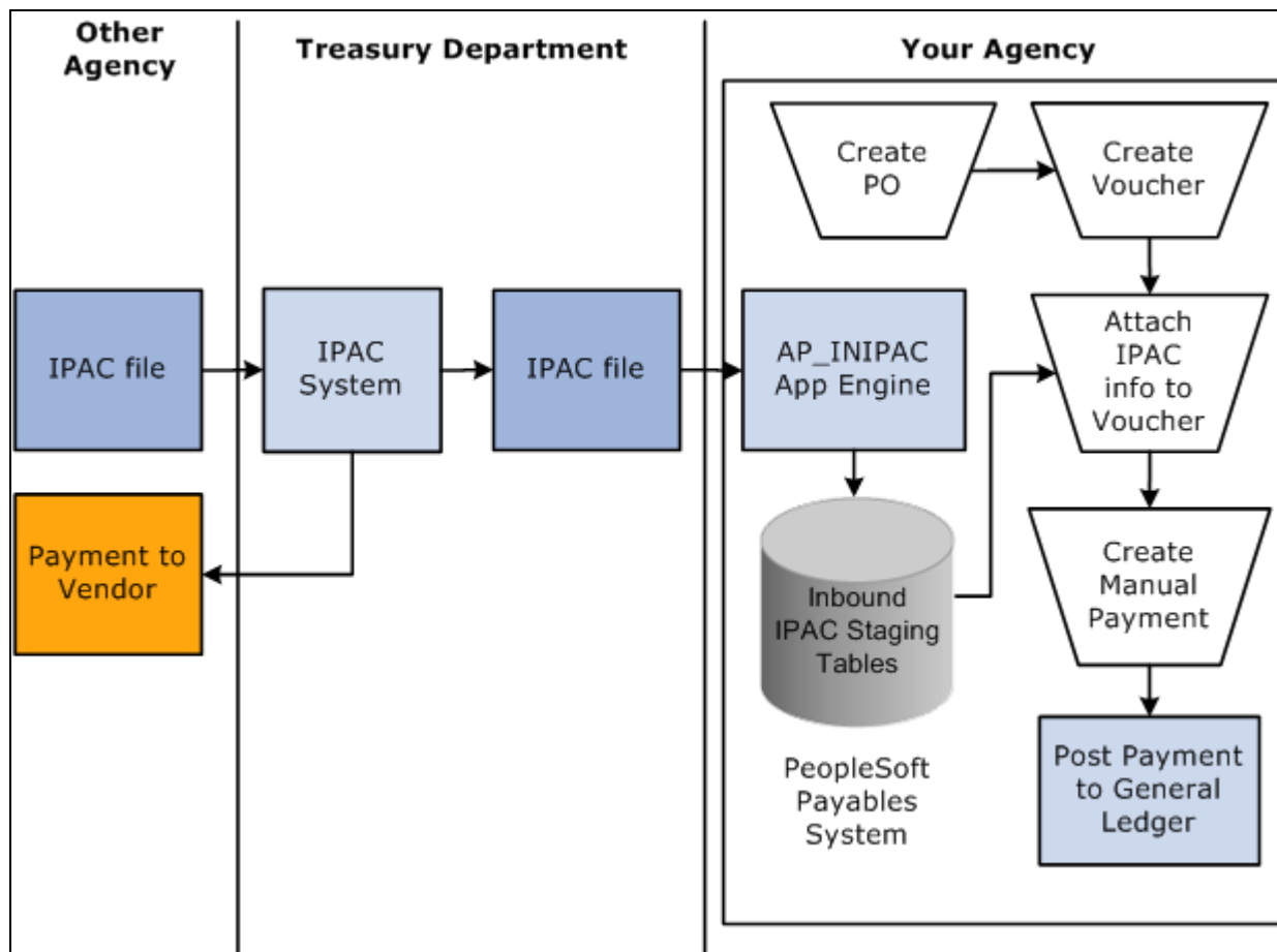
Inbound IPAC processing in PeopleSoft Payables
