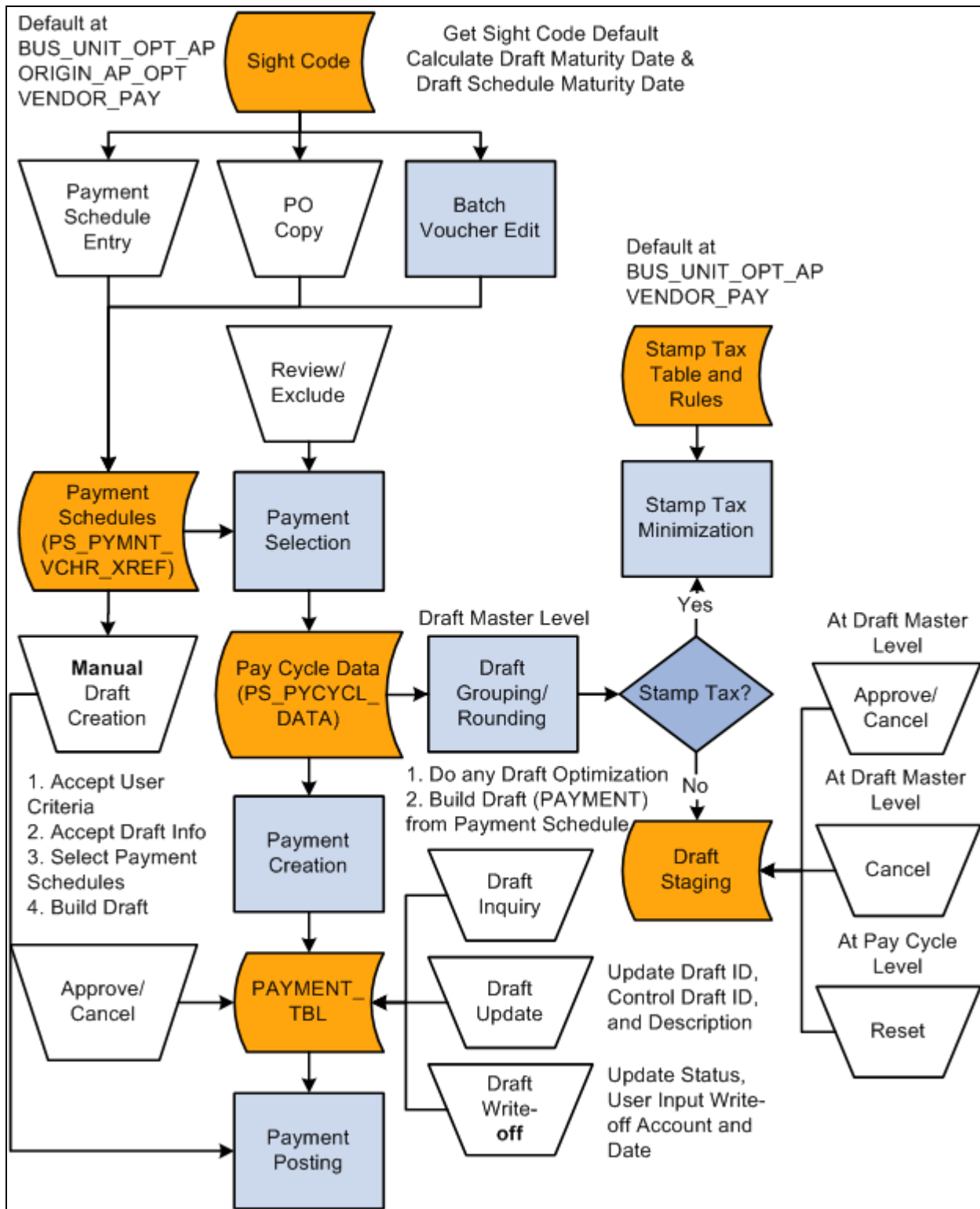
Draft Payment process
