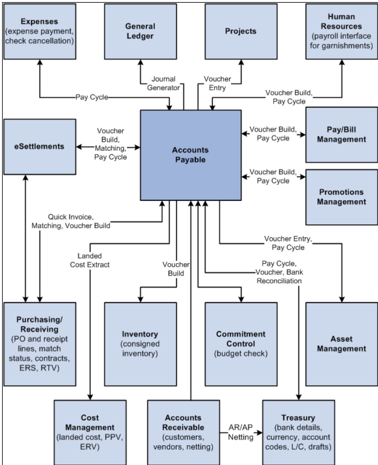
PeopleSoft Payables integrations with other PeopleSoft products
