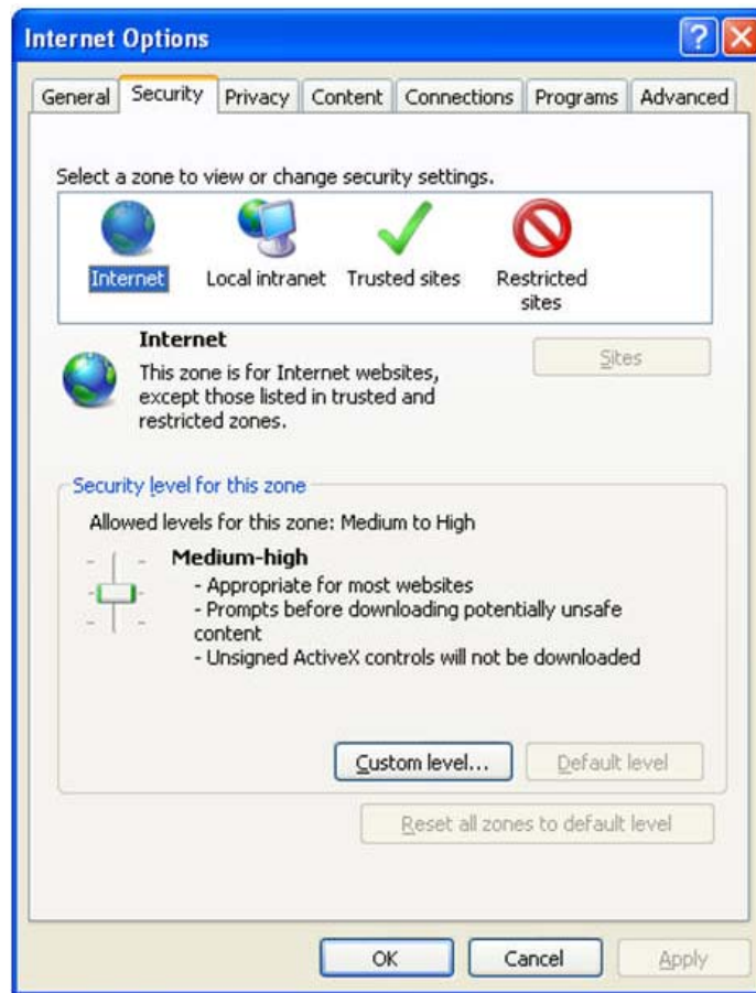
Figure 1: Internet Options
