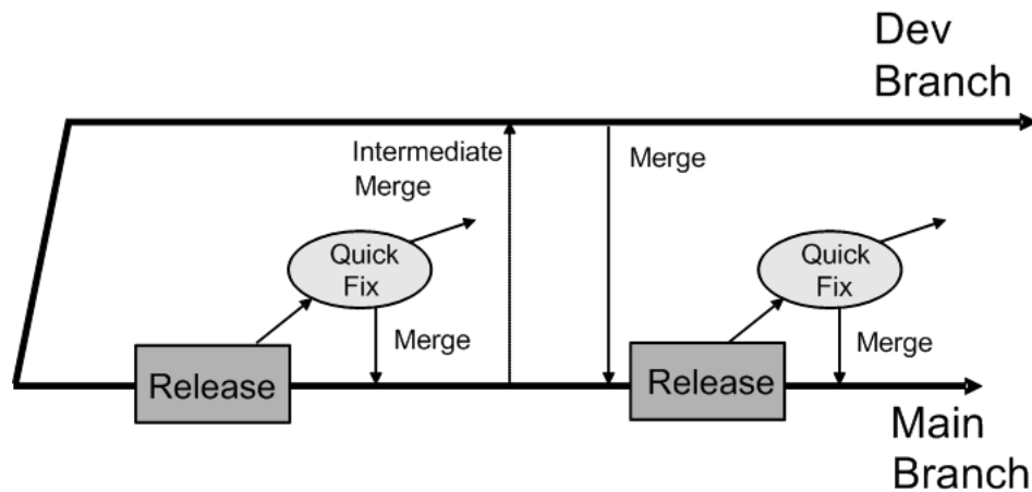
Figure 3–5 Small Team Development Model
