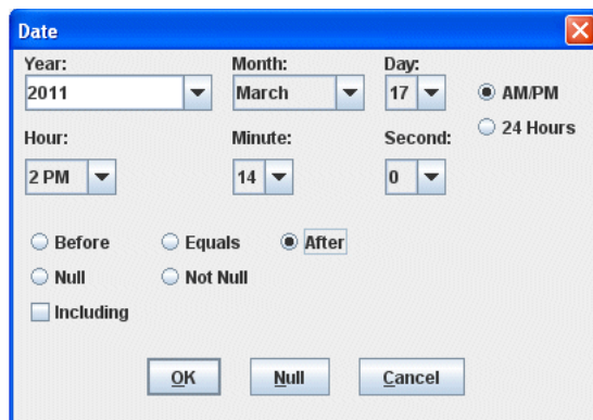
Figure 6-6 Setting a Date Filter in DAC
