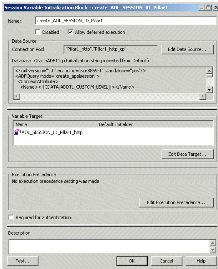
Figure 6–9 Session Variable Initialization Block Dialog for Pillar-Specific Initialization Block
