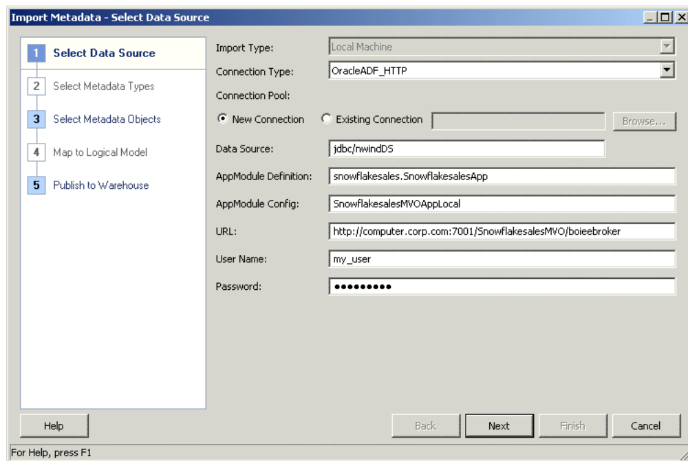
Figure 6–1 Import Metadata Wizard: ADF Data Source
