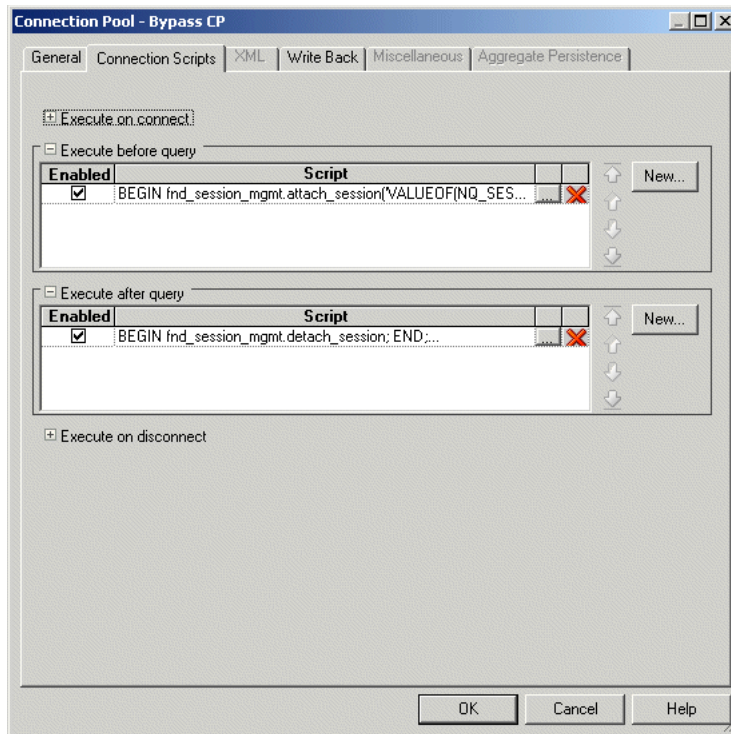
Figure 6–8 Pre-query and Post-query Scripts for the SQL Bypass Connection Pool
