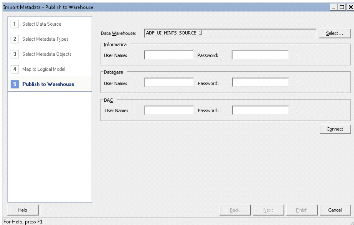
Figure 6–5 Publish to Warehouse Screen of Import Metadata Wizard
