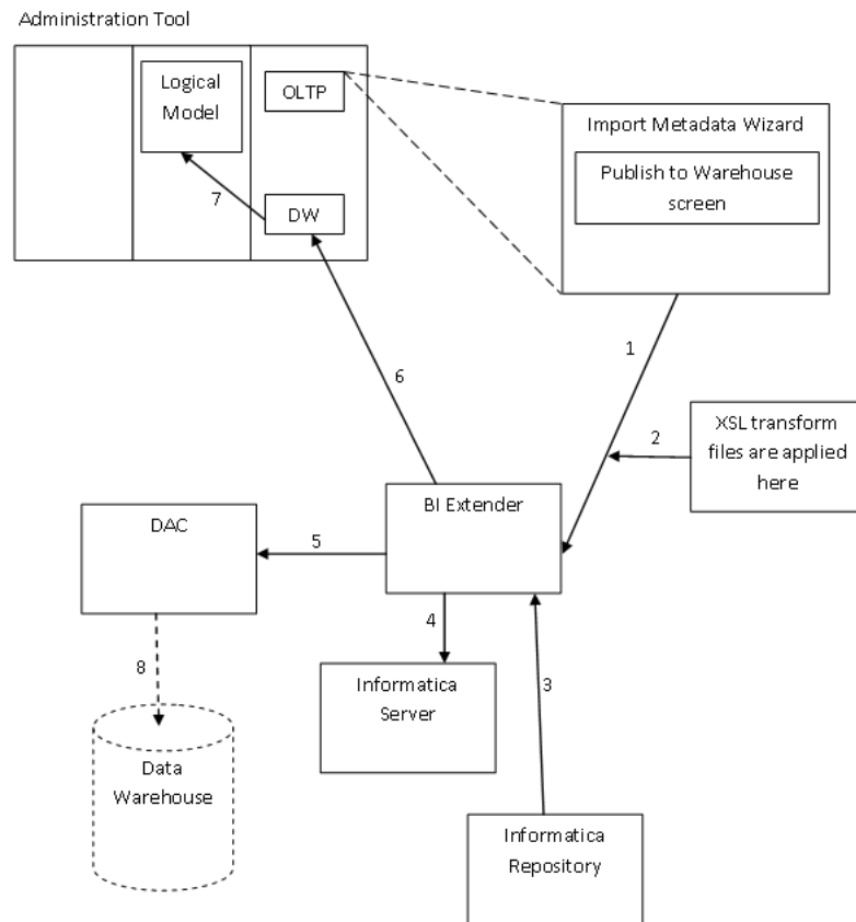
Figure 6–4 BI Extender Orchestration of Flexfield Object Changes
