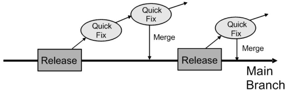
Figure 3–4 Simple Development Model
