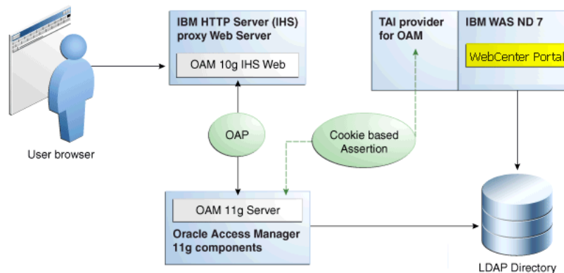
Figure 5–19 Configuring OAM Single Sign-On for WebCenter Portal Installations on IBM WebSphere
