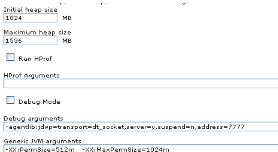
Figure 6–7 JVM Startup Parameters
