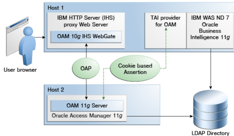
Figure 11–2 Components and Process Flow with OAM 11g and the IAP
