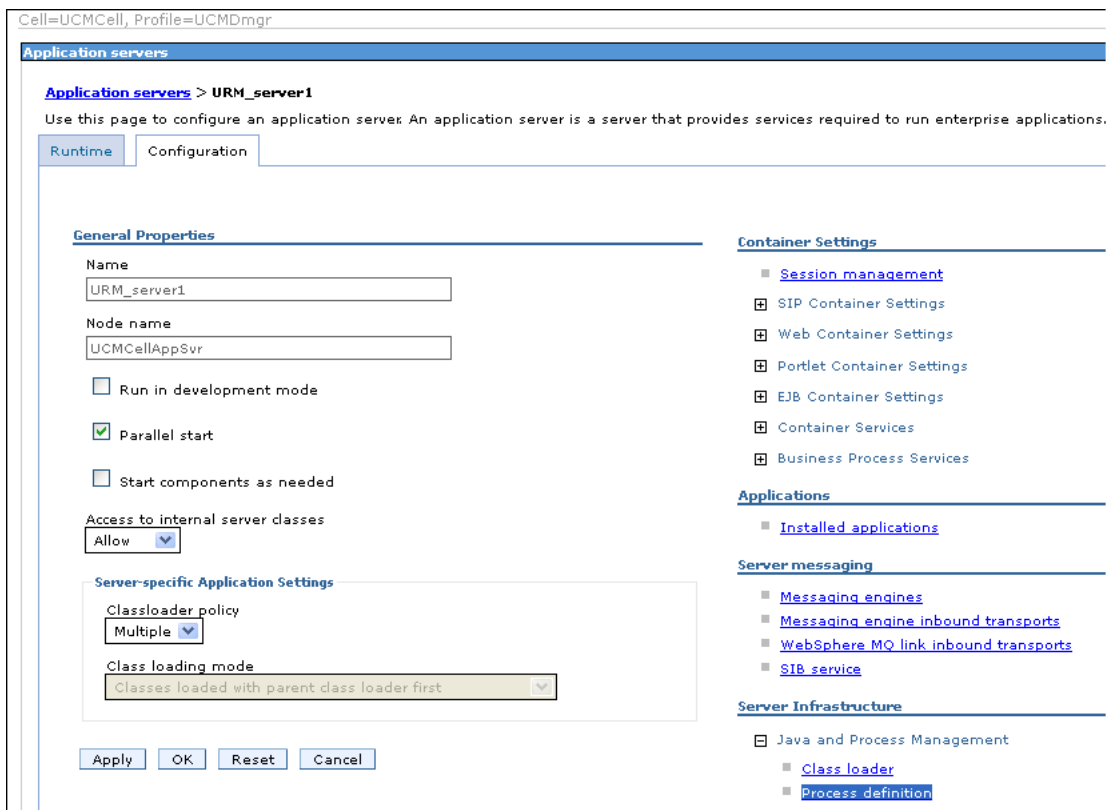
Figure 6-5 General Properties Page
