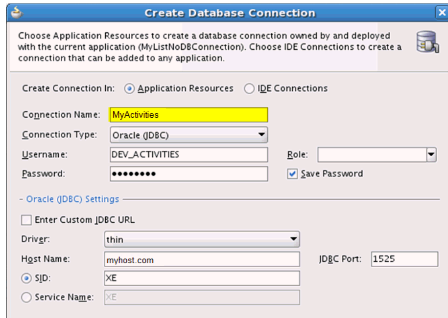
Figure 5–33 Database Connection Name - MyActivities
