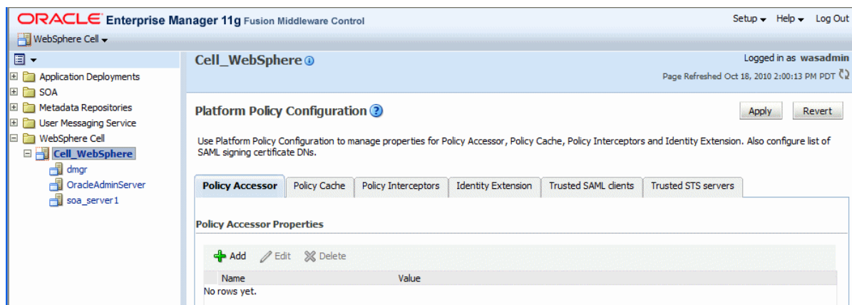
Figure 8–1 Platform Policy Configuration
