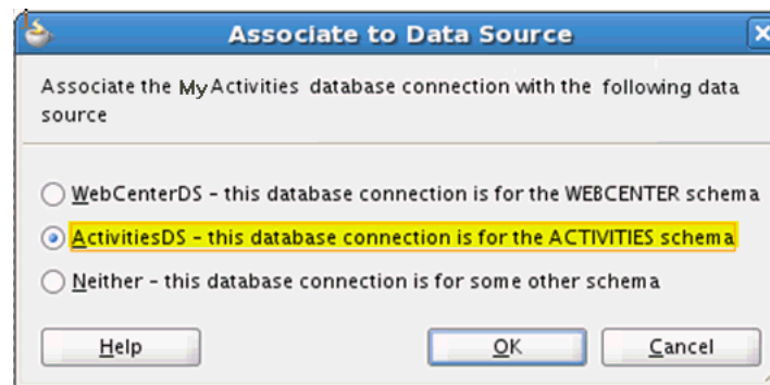
Figure 5–34 Associate MyActivities Connection to ActivitiesDS
