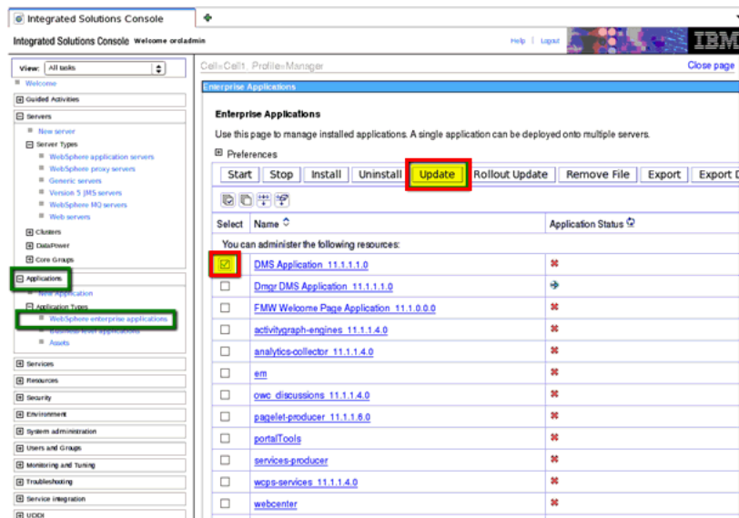
Figure 5-56 Update Enterprise Application Deployment
