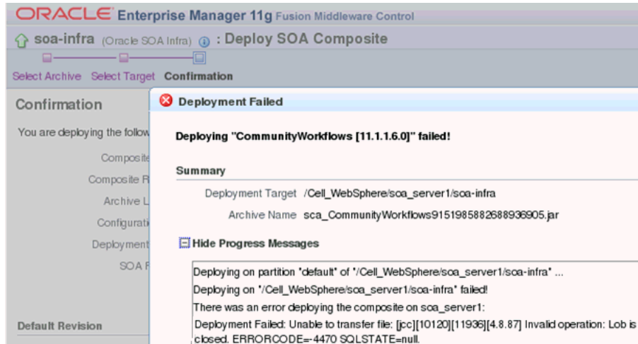
Figure 5–65 scs_CommunityWorkflows Fails to Deploy
