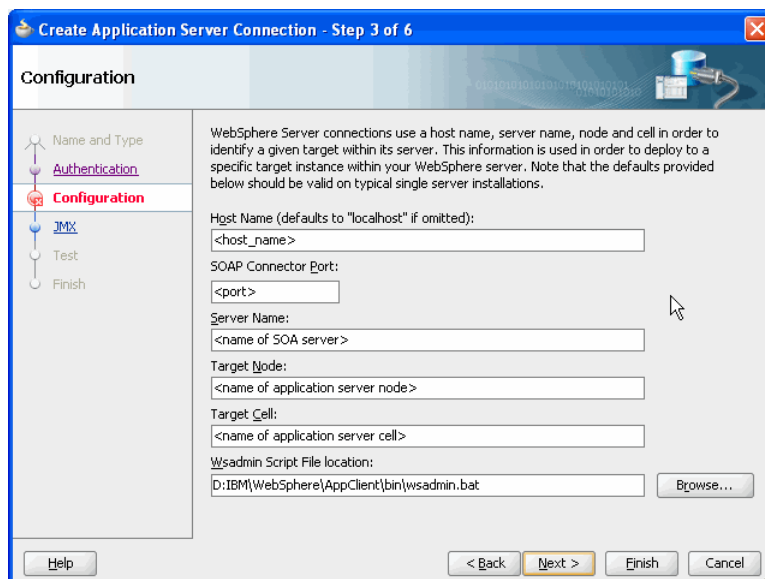
Figure 4-1 Configuring Server Details for an Application Server Connection
