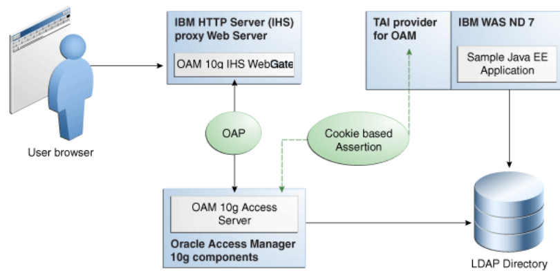
Figure 11–1 Components and Process Flow with OAM 10g (10.1.4.3) and the IAP
