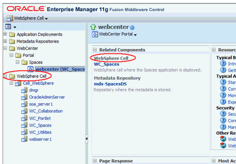
Figure 5–54 Fusion Middleware Control Home Page for Spaces Deployment on IBM WebSphere
