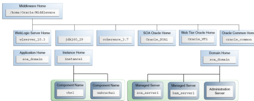
Figure 2–8 Directory Structure with an Oracle Instance and a WebLogic Server Domain
