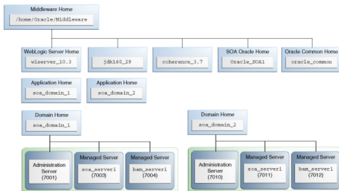
Figure 2–5 Directory Structure with Multiple Instances of a Single Product
