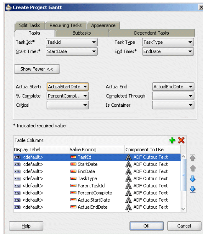
Figure 26–41 Create Project Gantt Dialog for Orders Shipped
