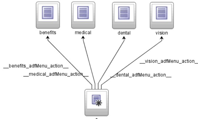
Figure 18–21 Updated Unbounded Task Flow
