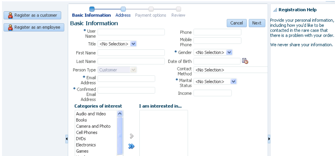
Figure 17–11 Customer Registration Task Flow in an ADF Dynamic Region
