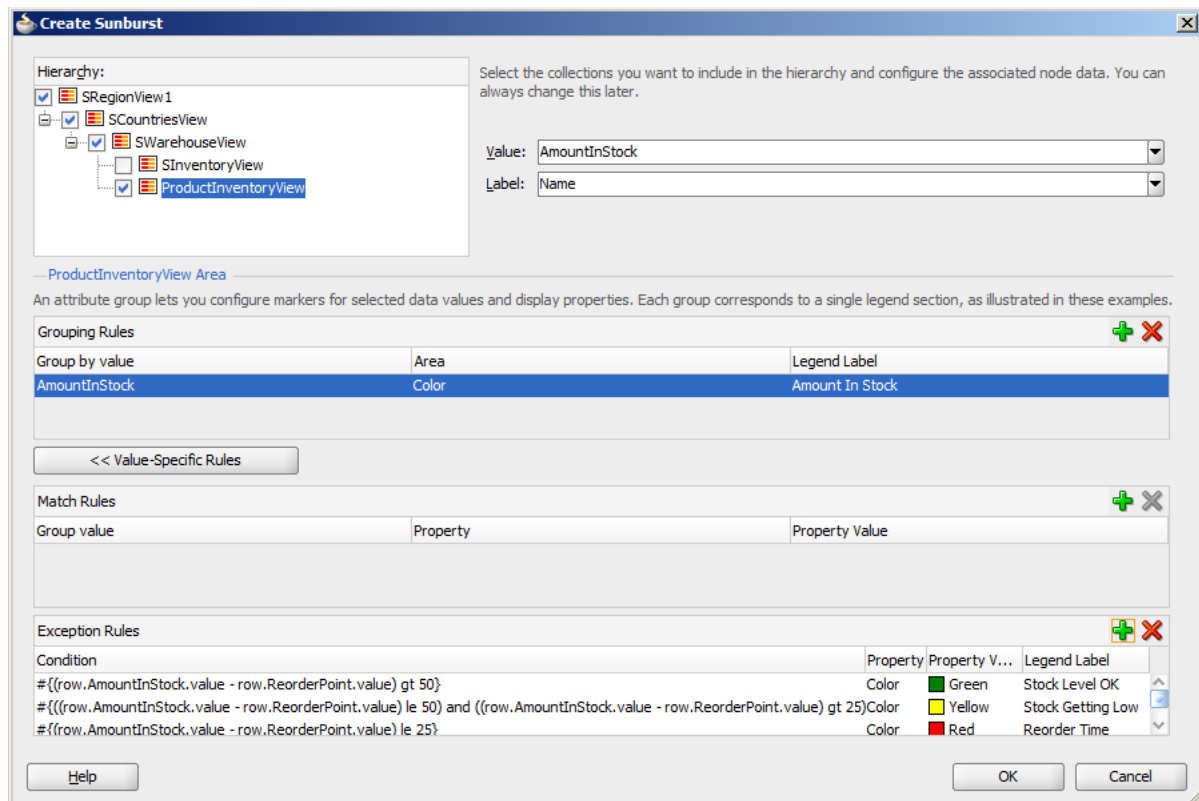
Figure 26–68 Sunburst Showing Exception Rules Creation Dialog
