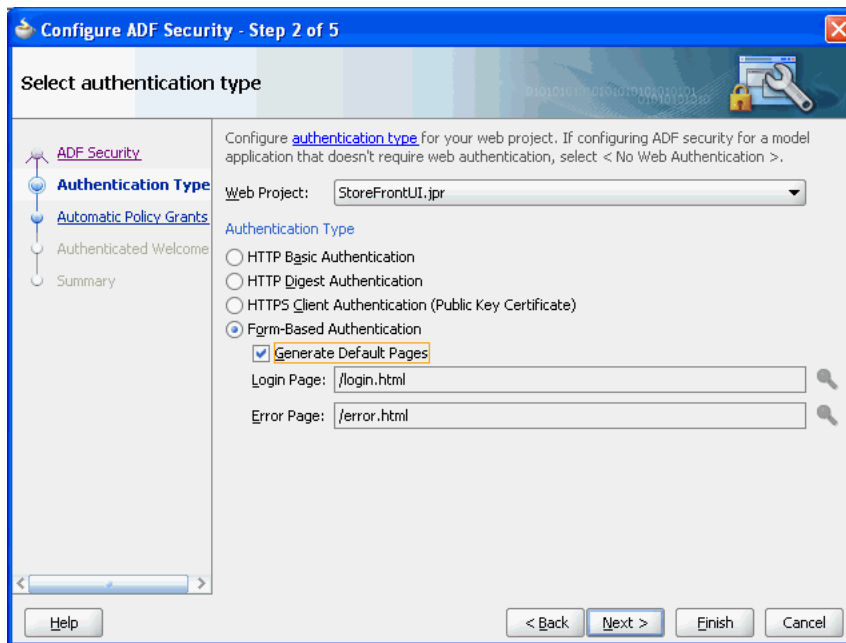
Figure 30-3 Using the Configure ADF Security Wizard to Generate a Simple Login Page
