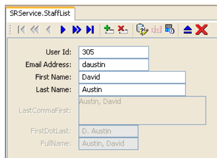
Figure 5–49 View Object with Three Kinds of Calculated Attributes
