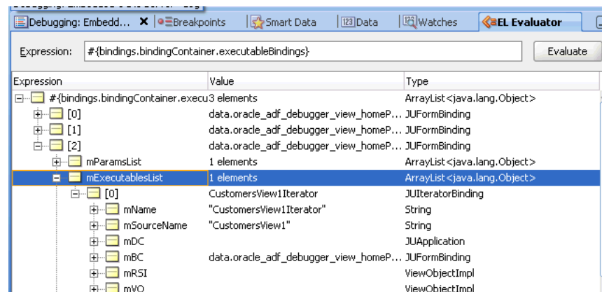
Figure 31–13 EL Expression Evaluated
