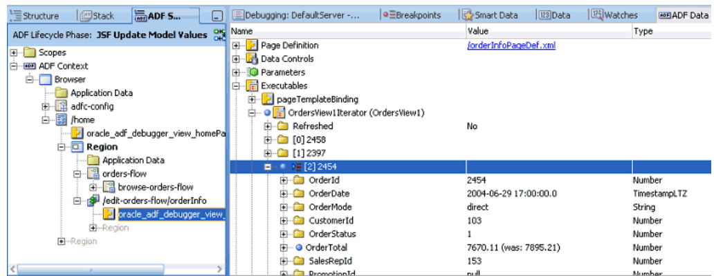
Figure 31–42 A Value Change Is Indicated by a Blue Dot in the ADF Data Window
