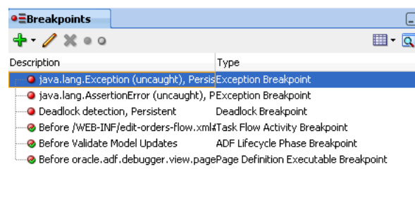
Figure 31–19 Breakpoints window Showing ADF Declarative and Java Code Breakpoints
