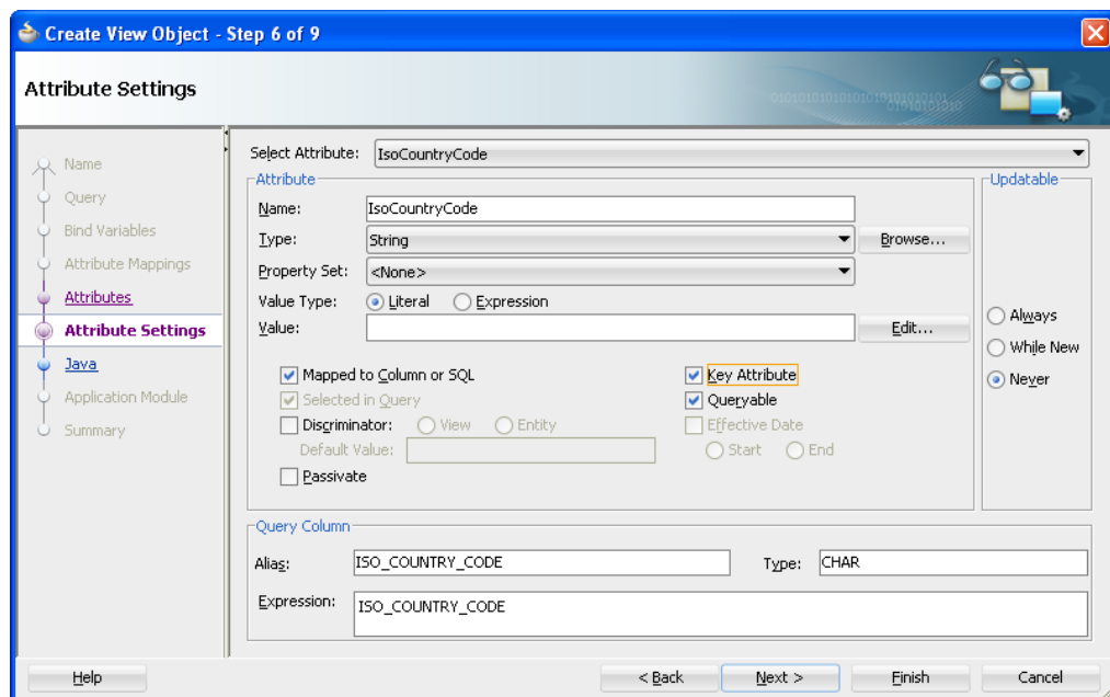
Figure 5–9 Create View Object Wizard, Attribute Settings Page
