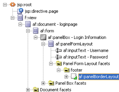
Figure 30–22 Login Page Structure with Panel Border Layout
