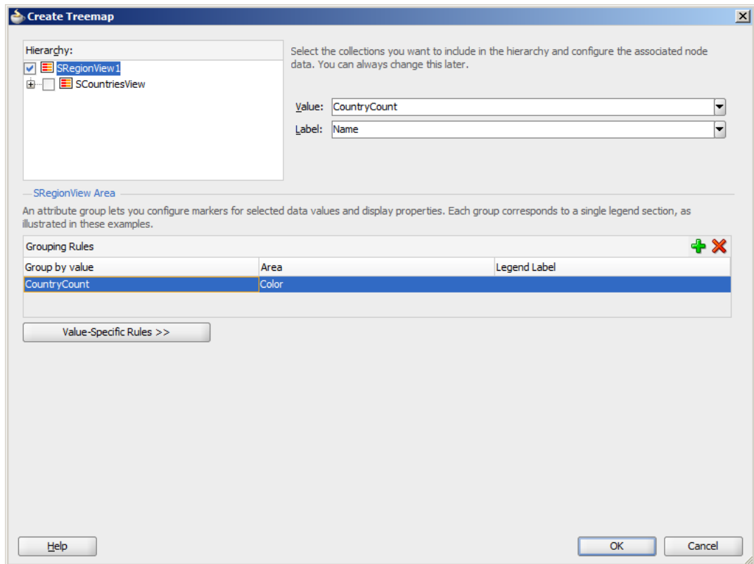
Figure 26–65 Create Treemap Dialog for a Region Node
