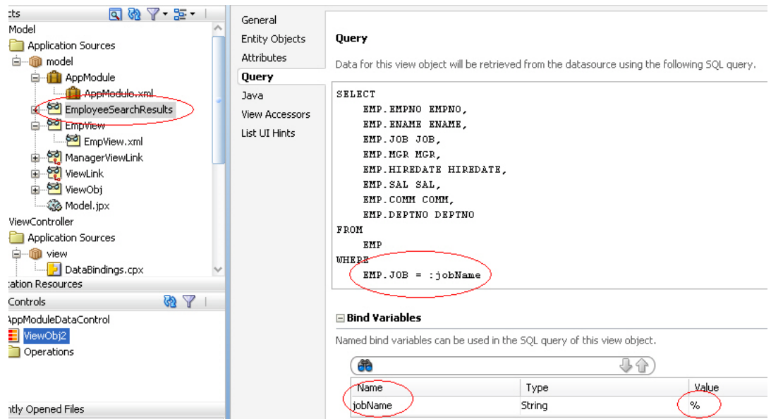
Figure 26–59 EmployeeSearchResults View Object
