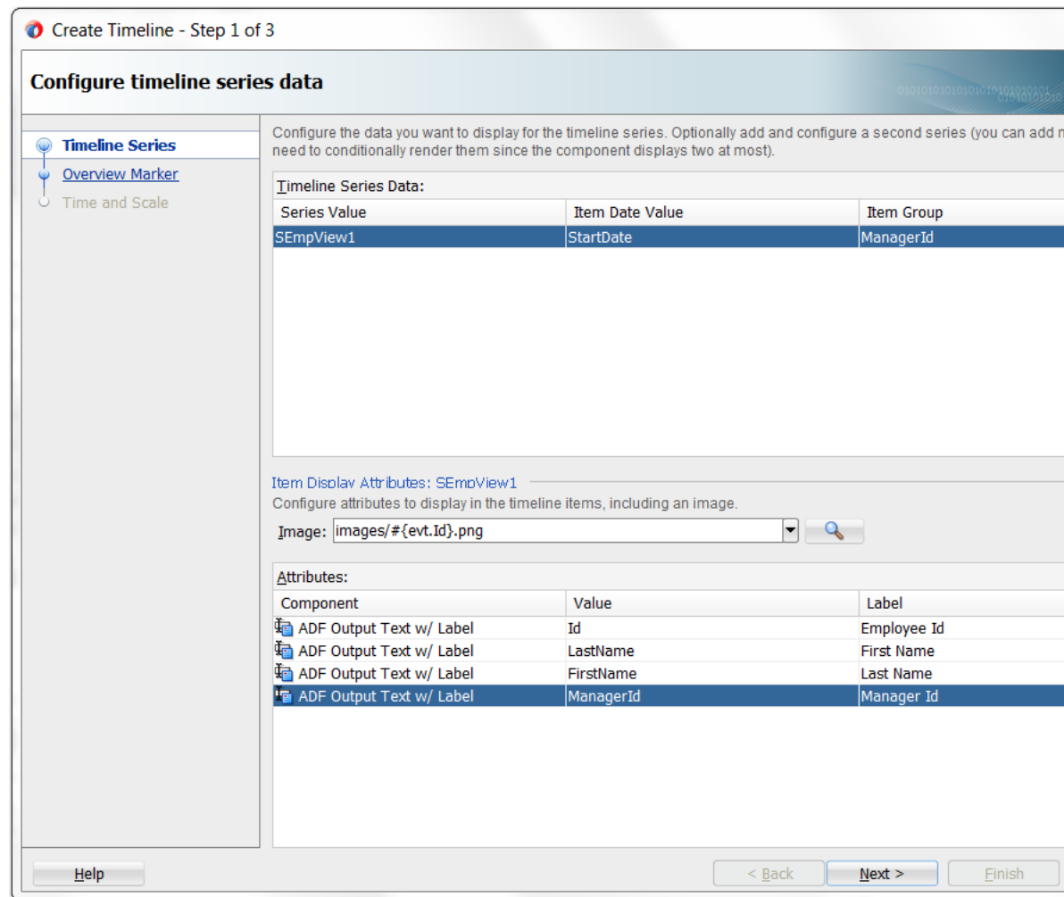
Figure 26–51 Configure Timeline Series Data Page of Create Timeline Wizard
