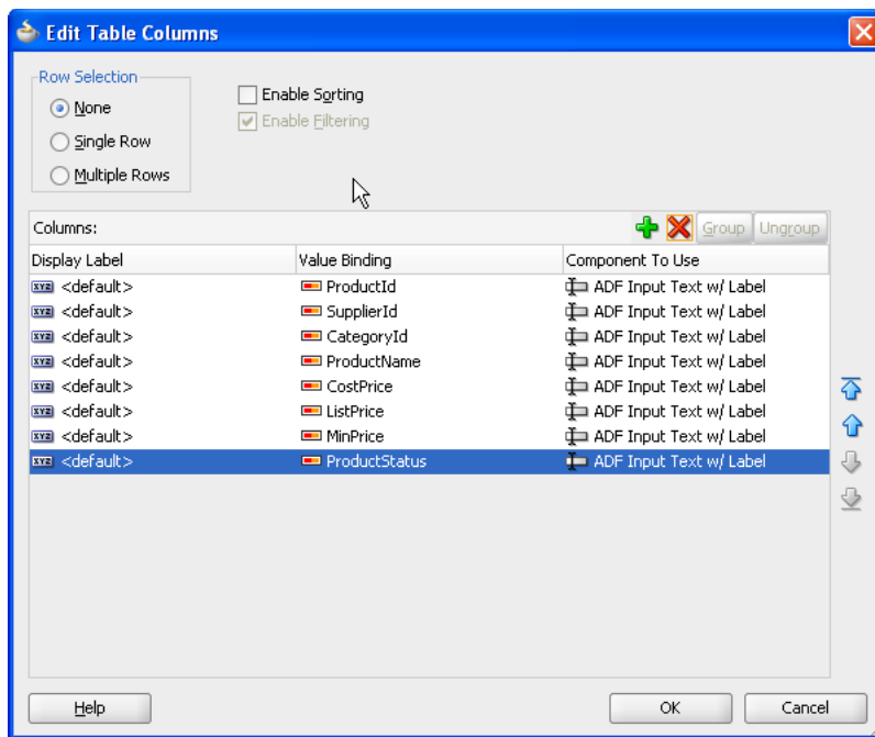
Figure 27–20 Edit Table Columns Dialog for Filtered Table
