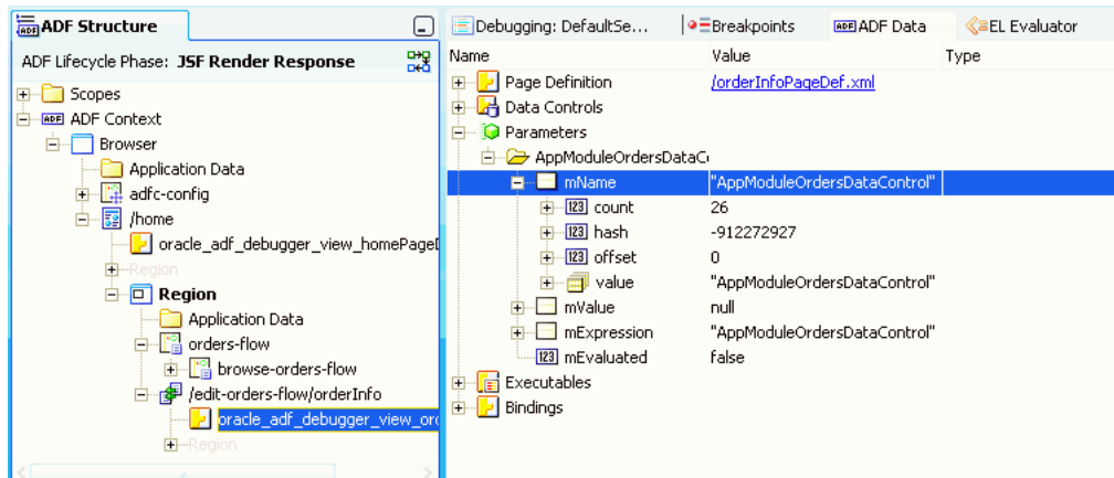
Figure 31-40 Parameters Selected for the ADF Data Window
