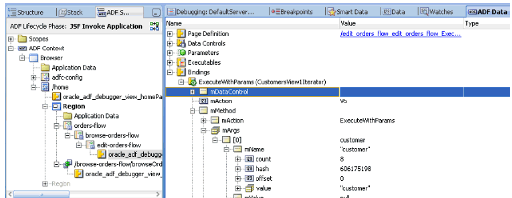
Figure 31–43 Method Bindings Selected for the ADF Data Window
