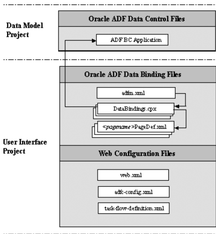
Figure A-1 Oracle ADF File Hierarchy Overview for the Fusion Web Application
