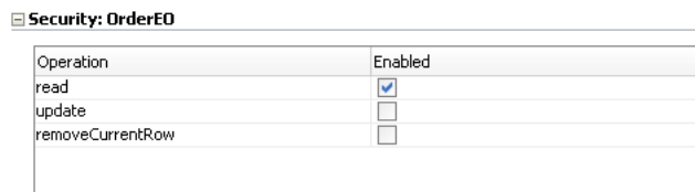
Figure 30–11 Permission Enabled on read Operation for an ADF Entity Object
