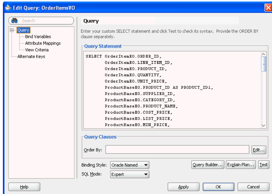
Figure 5–38 OrderItems Expert Mode View Object
