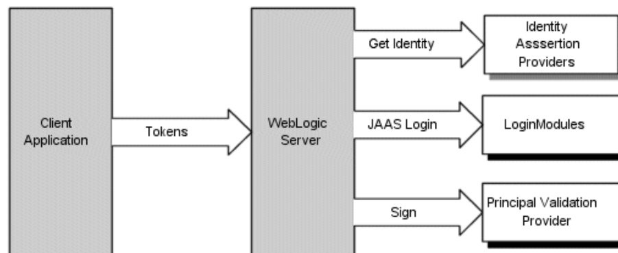
Figure 5-3 Perimeter Authentication
