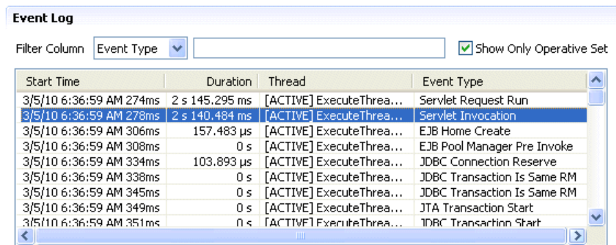
Figure 3–8 Adding all WebLogic Server Events to Operative Set
