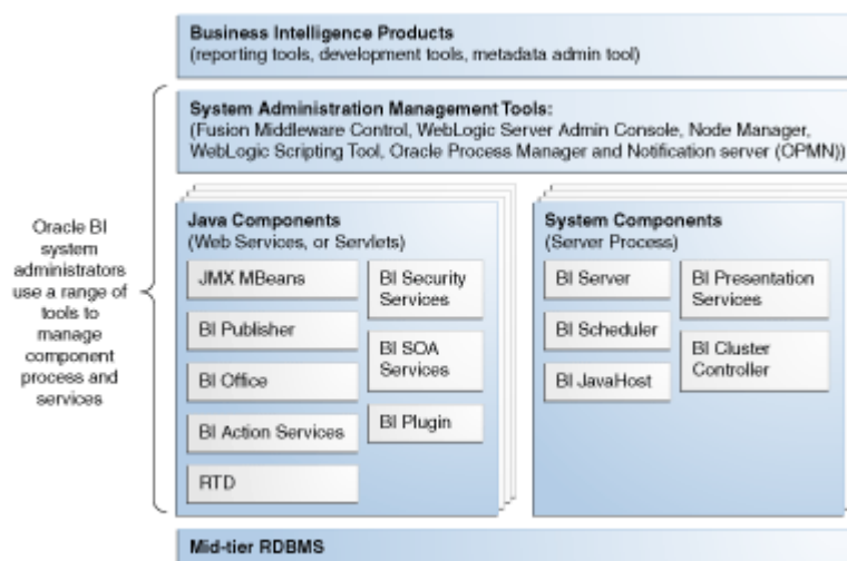
Figure 1–3 Oracle Business Intelligence Components
