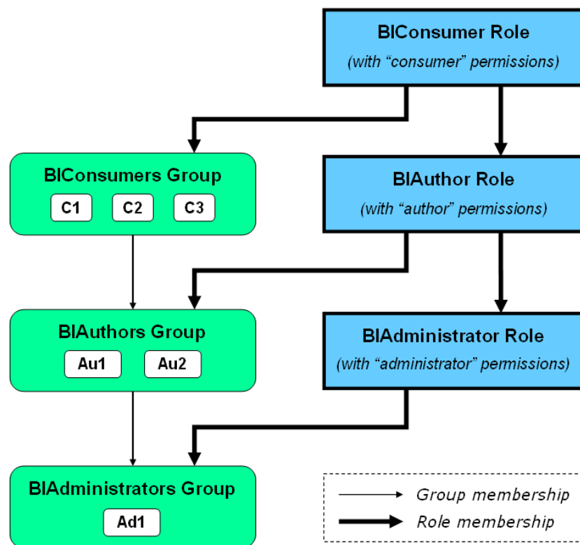
Figure 4–1 Example of Oracle Fusion Middleware Security Elements
