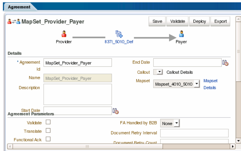
Figure 14–3 Mapset Page in Oracle B2B
