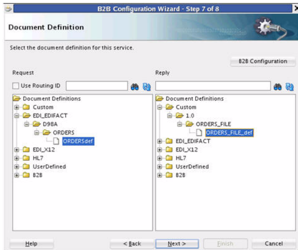
Figure B-3 B2B Configuration Wizard: Document Definition Page
