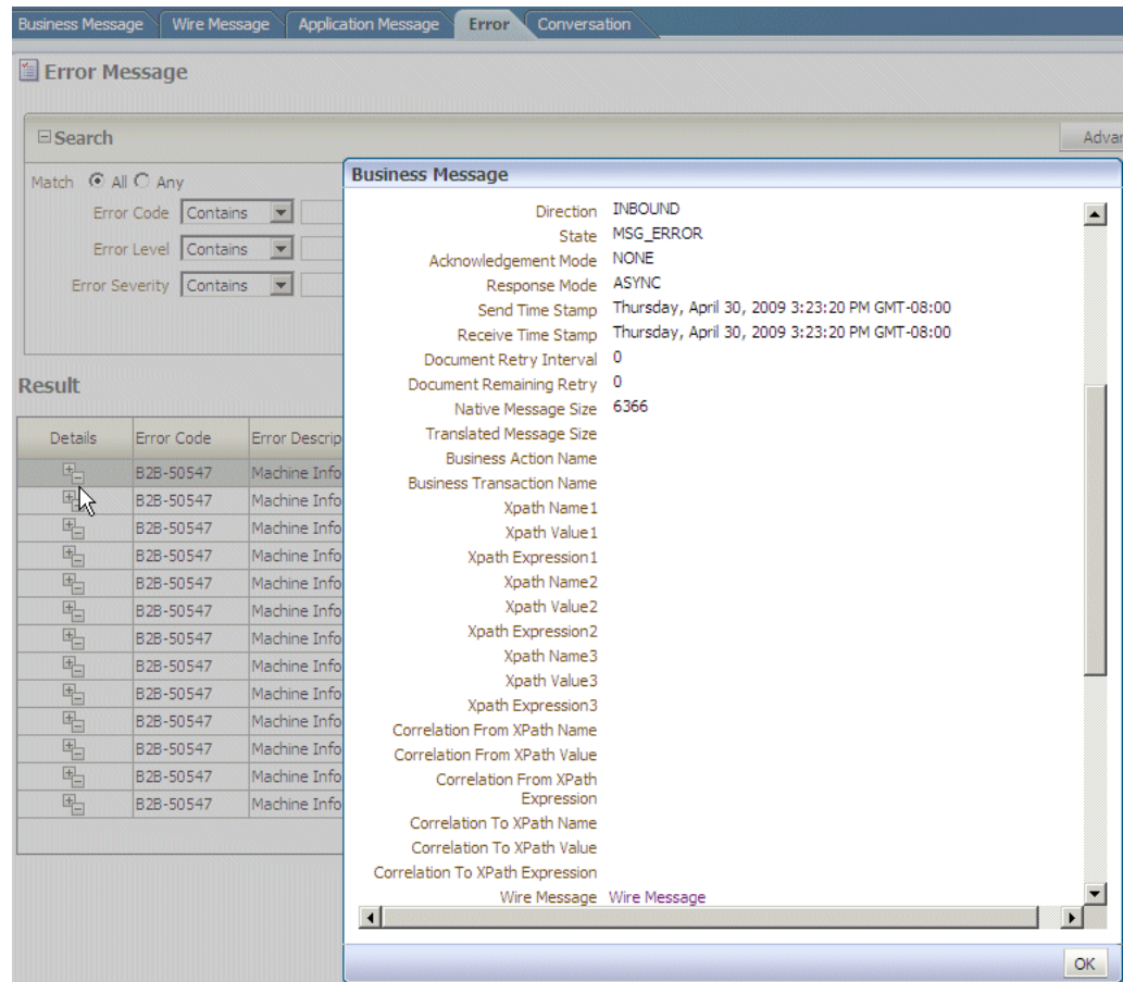
Figure 18–8 Error Reports
