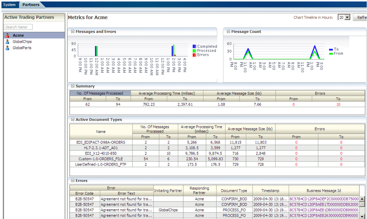
Figure 19–5 Partner Metrics
