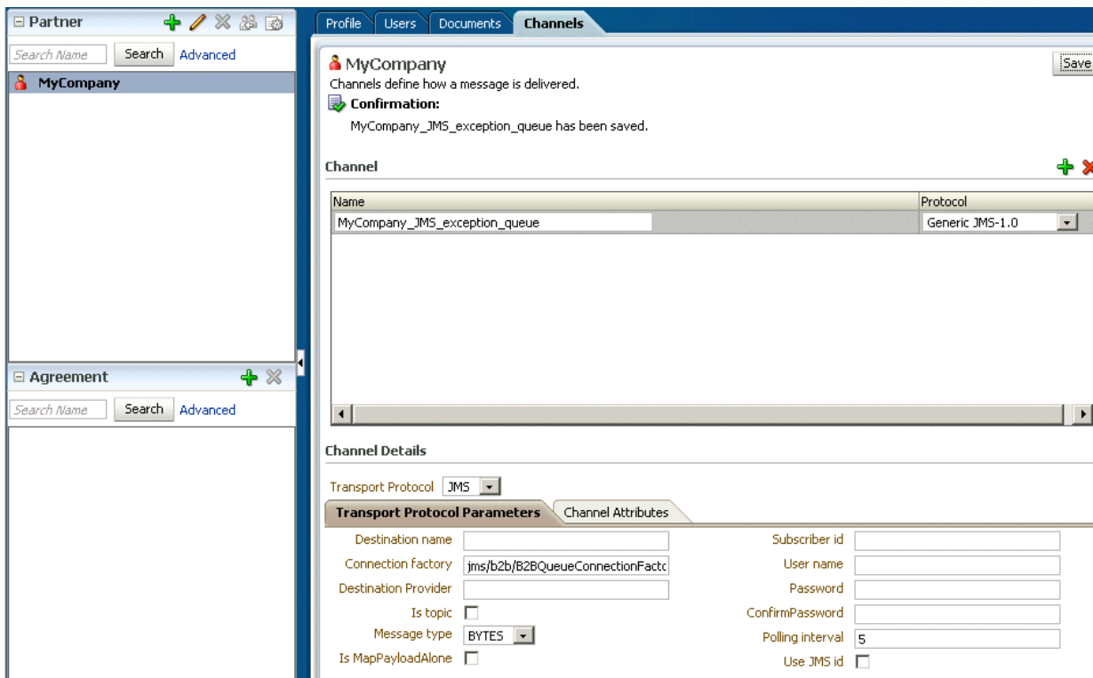
Figure G-1 Creating a Custom Exception Queue
