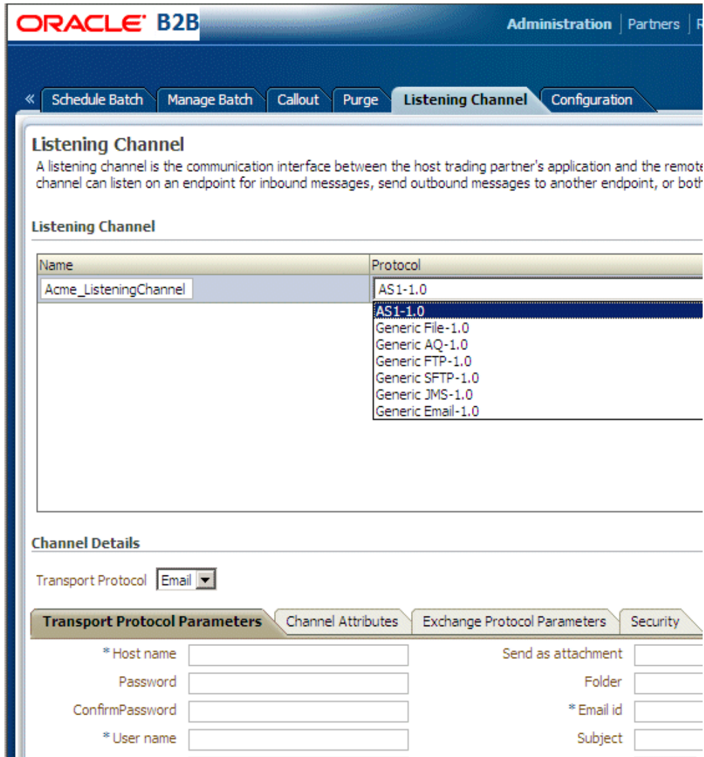
Figure 16–1 Adding a Protocol for a Listening Channel
