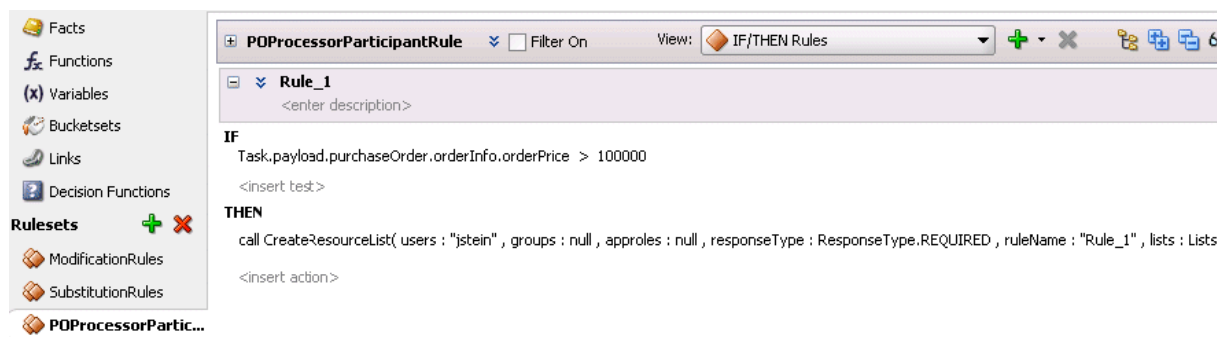
Figure 29–31 Business Rules
