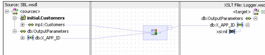
Figure 49–36 SBL_TO_COMMON_INSERT.xsl Transformation
