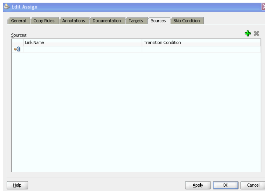
Figure 10–6 Source Activity
