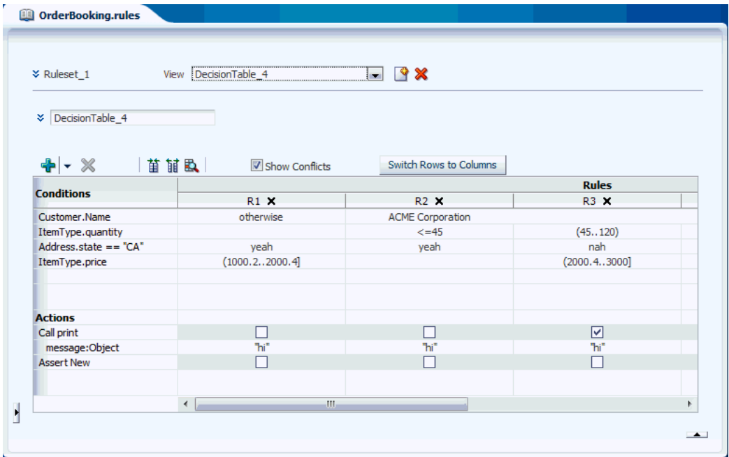
Figure 26–4 Decision Tables
