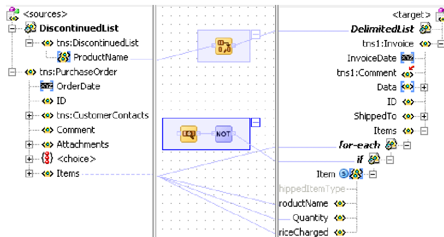
Figure 40–53 Mapper File
