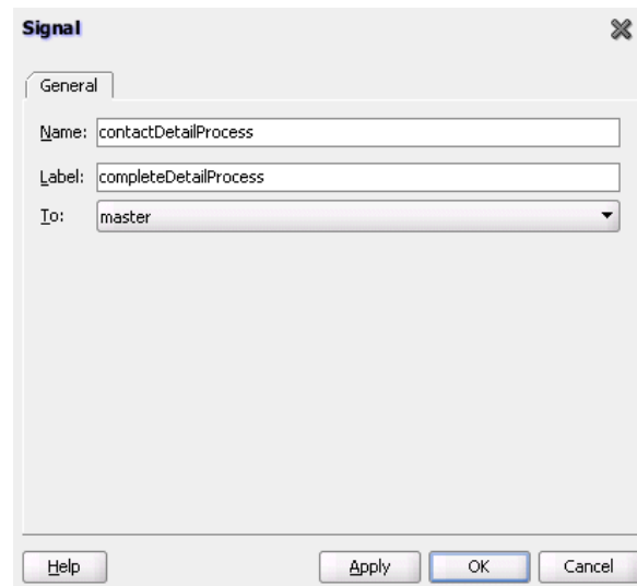
Figure 16–7 Signal Dialog
