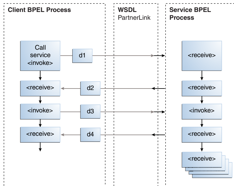
Figure 5–9 Partial Processing
