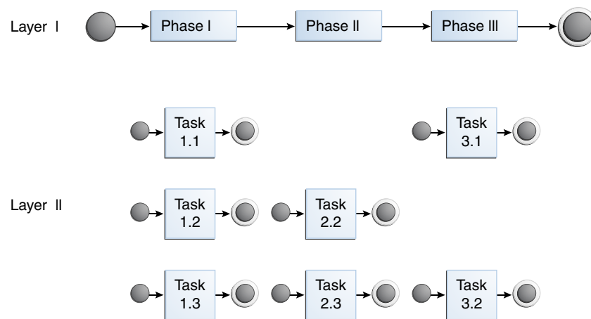
Figure 51–1 Two-Layer BPM
