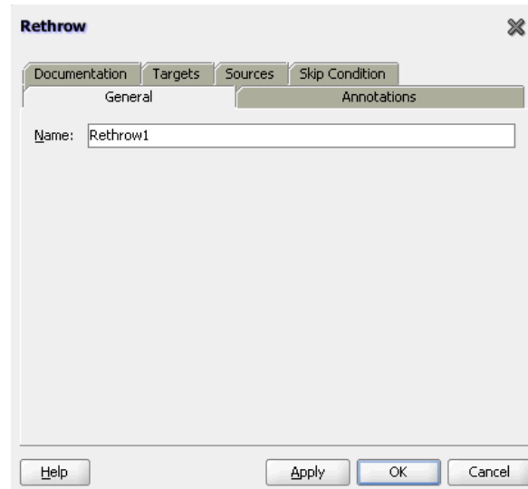
Figure 12-4 Rethrow Dialog
