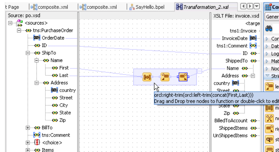
Figure 40–20 Chaining Functions
