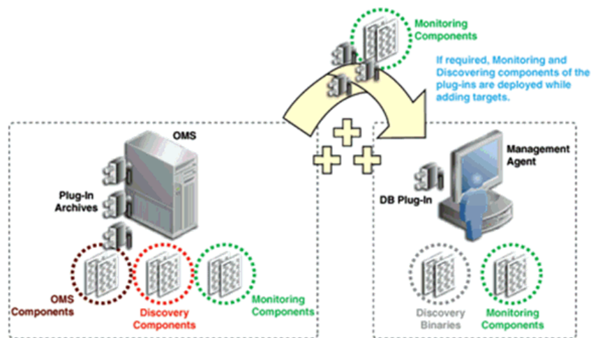
Figure 22–4 Adding Targets
