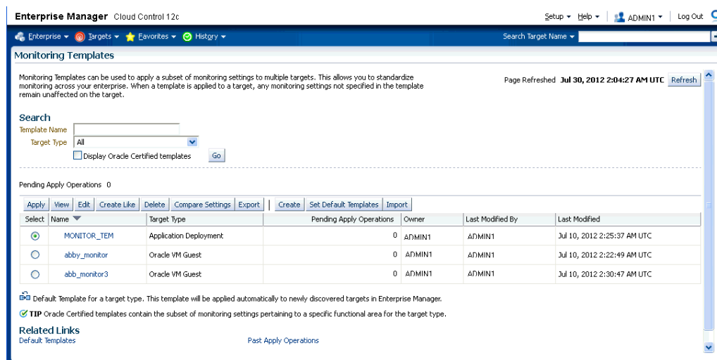
Figure 7–1 Monitoring Templates
