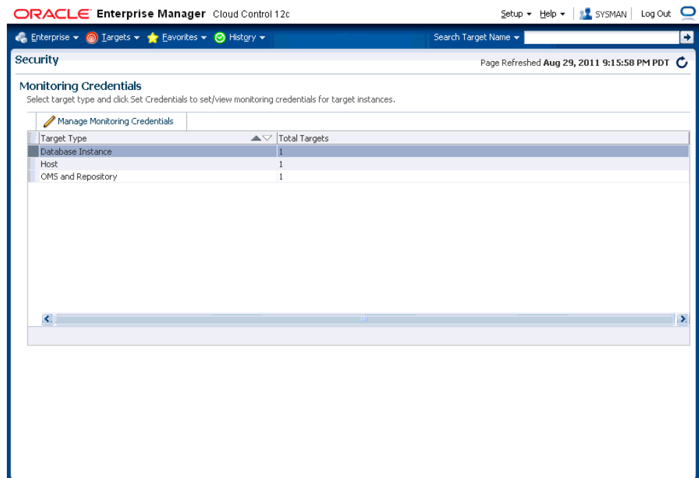
Figure 13–5 Monitoring Credentials
