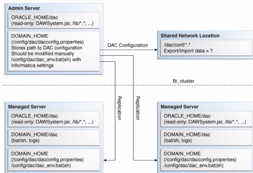
Figure 3–1 DAC Server Migration Approach to Failover
