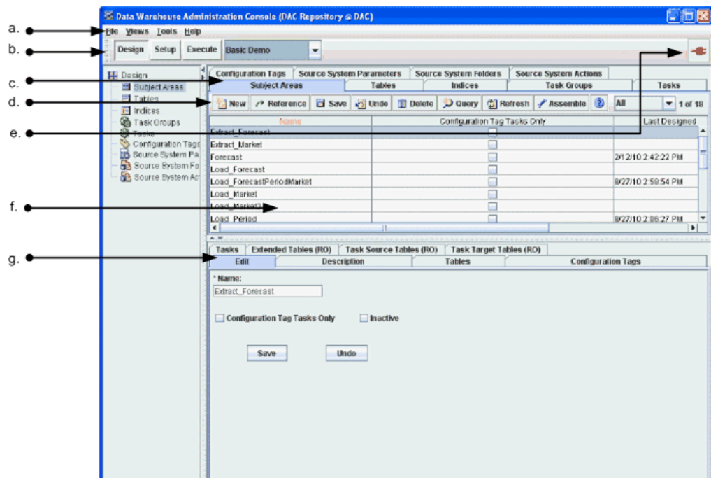
Figure 2–6 DAC Main Window
