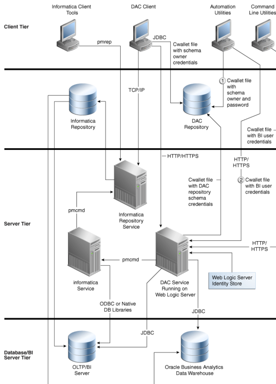
Figure 1–1 DAC Server Running as Service on WebLogic Server
