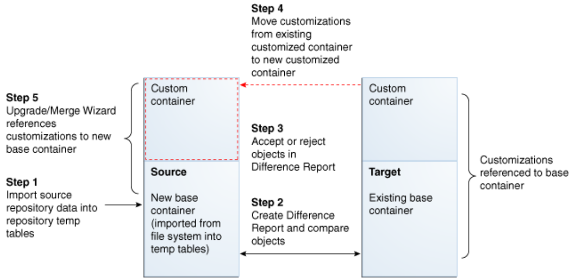
Figure 14–3 Upgrade Process for Refresh Base Option
