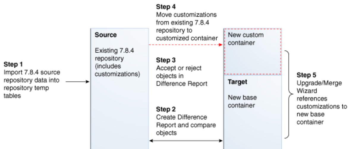
Figure 14–2 Upgrade Process for Repository Upgrade (DAC 784) Option
