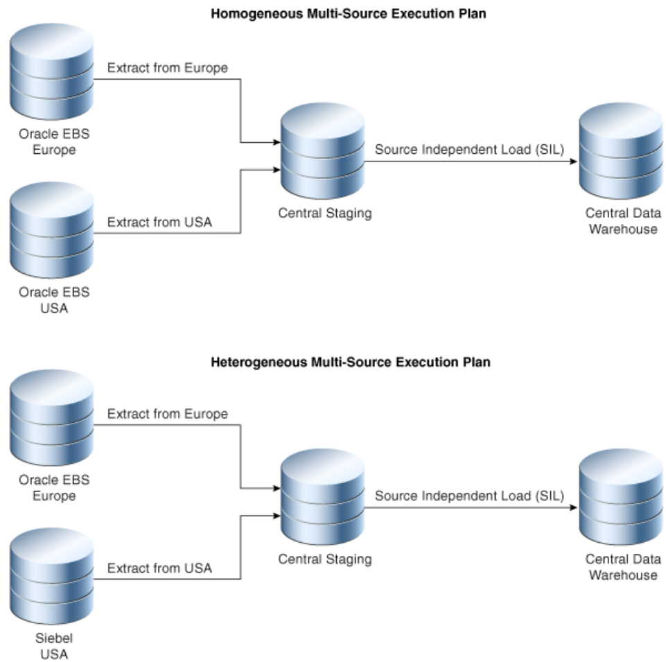
Figure 5–2 Multiple Extract and Single Load Option
