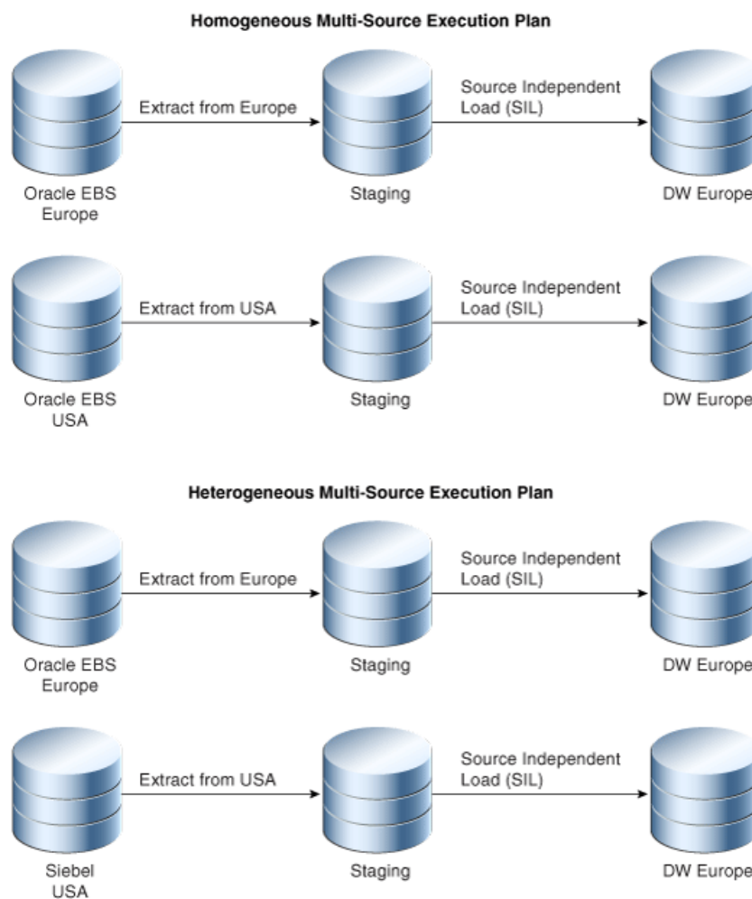
Figure 5–3 Multiple Extract and Multiple Load Scenario
