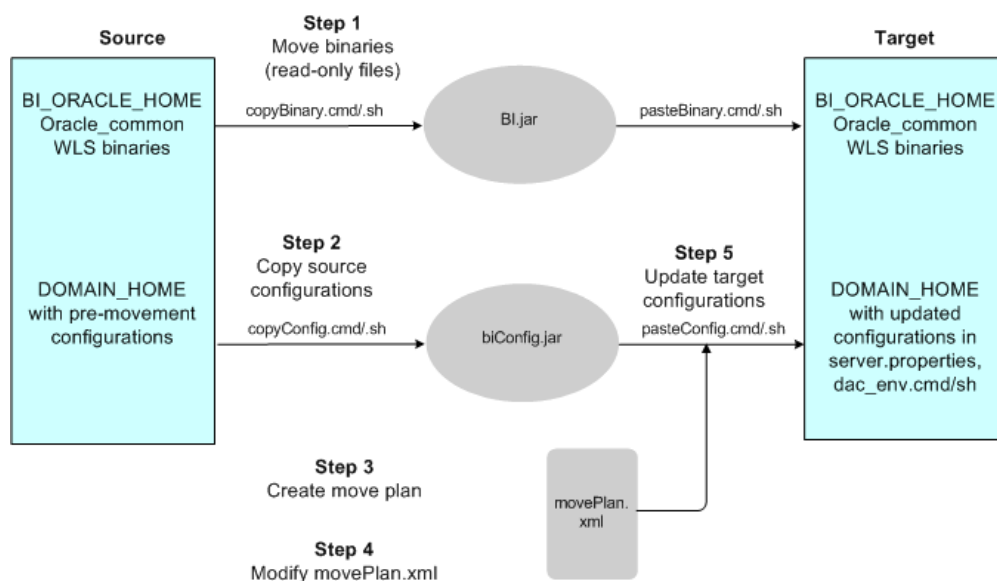
Figure 3–3 Flow for Moving DAC Components
