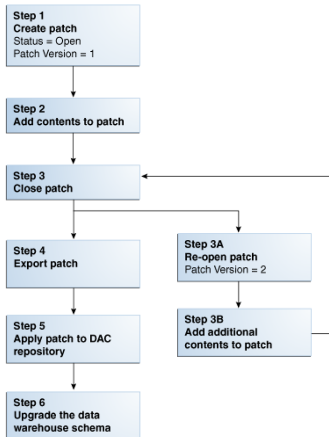
Figure 11–1 DAC Patch Process
