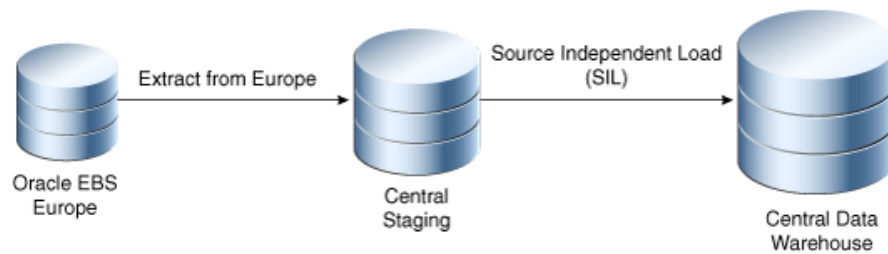
Figure 5–1 Single Extract and Single Load Option
