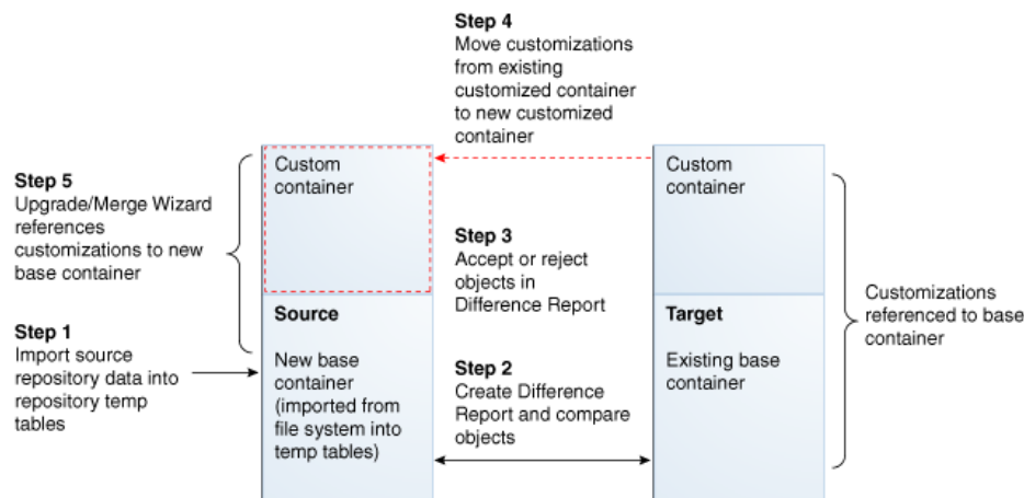
Figure 14–4 Upgrade Process for Replace Base Option
