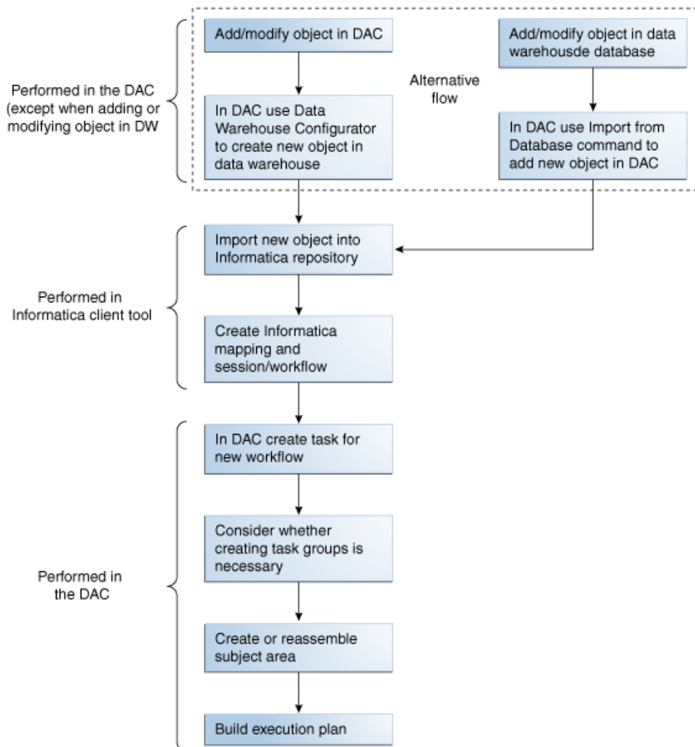
Figure 6–1 Process Flow to Add New Object to Data Warehouse
