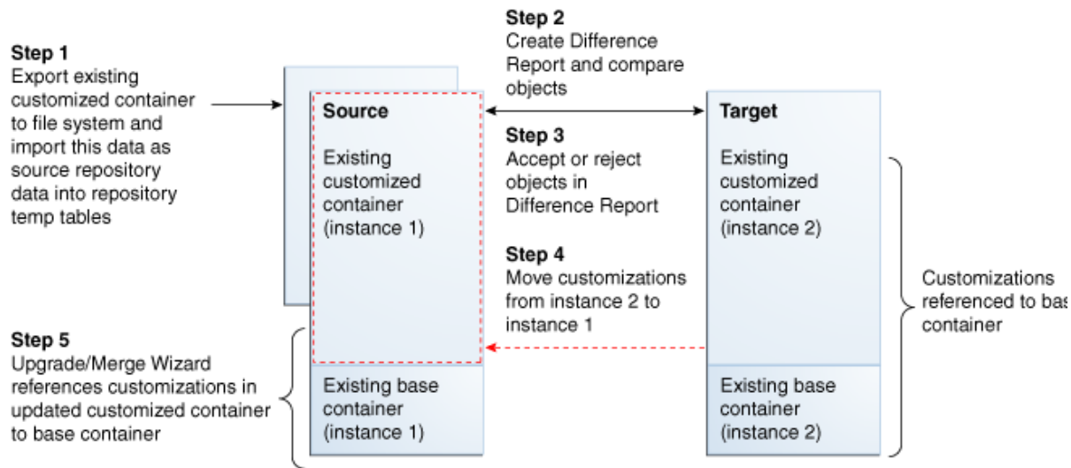
Figure 14–5 Merge Process for Peer to Peer Merge Option
