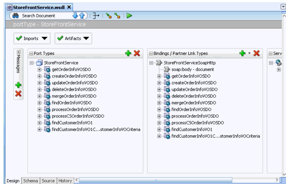
Figure 11–6 WSDL Document
