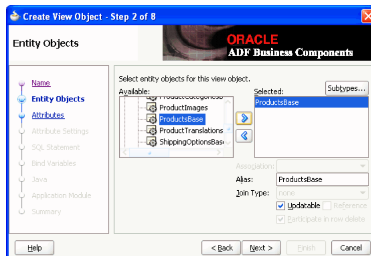
Figure 33–19 Creating View Object Using Entity Objects from ADF Library
