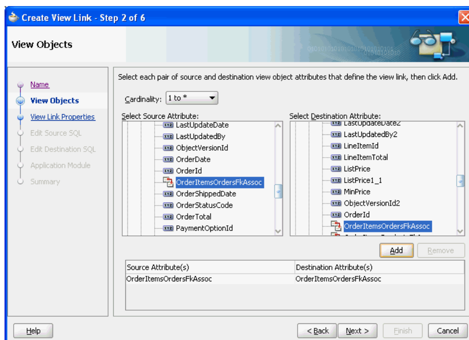
Figure 5–26 Master and Detail Related by an Association Selection
