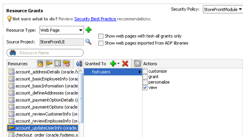
Figure 30–10 Granting to an Application Role for an ADF Page Definition in the Overview Editor
