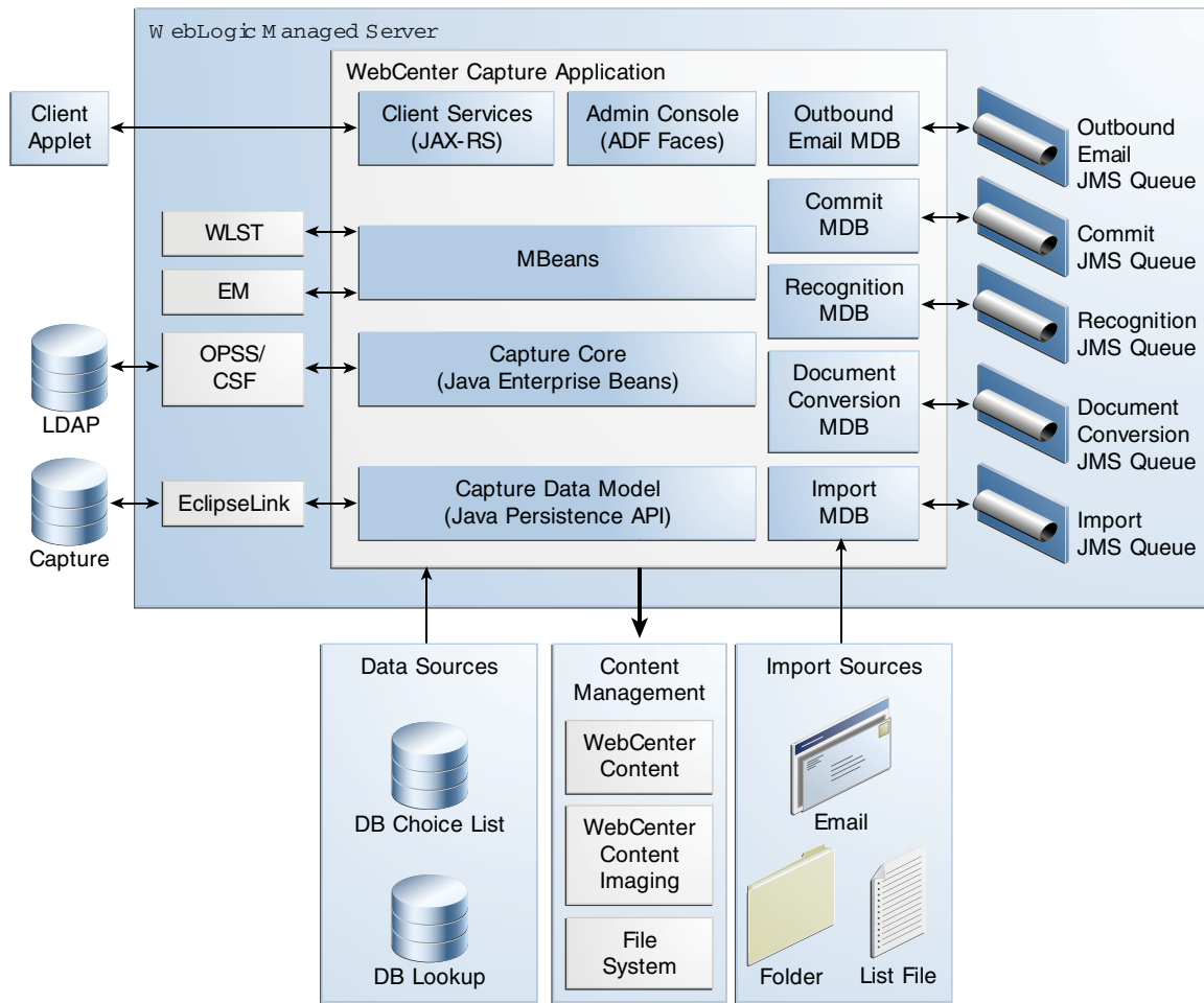
Figure 11–3 Capture Components for a Single Instance
