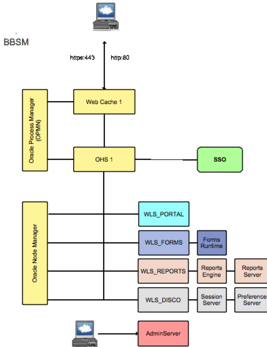
Figure 14-1 Oracle Portal, Forms, Reports, and Discoverer Architecture
