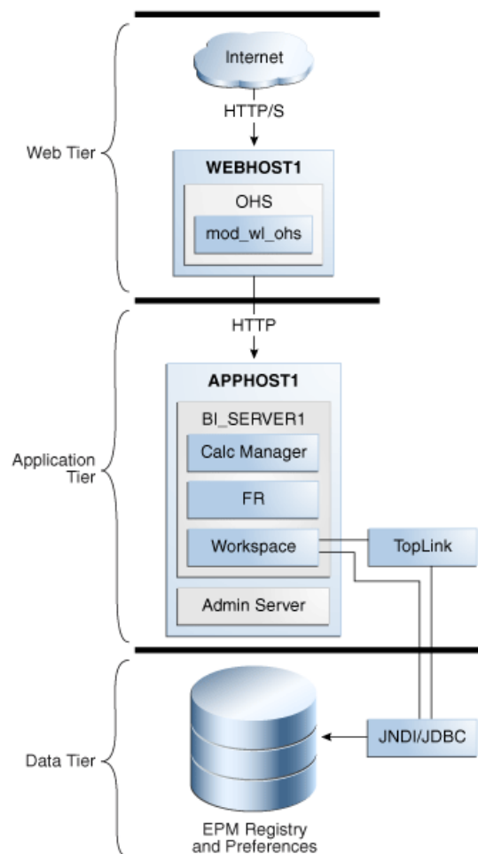
Figure 15-5 Workspace Single Instance Architecture
