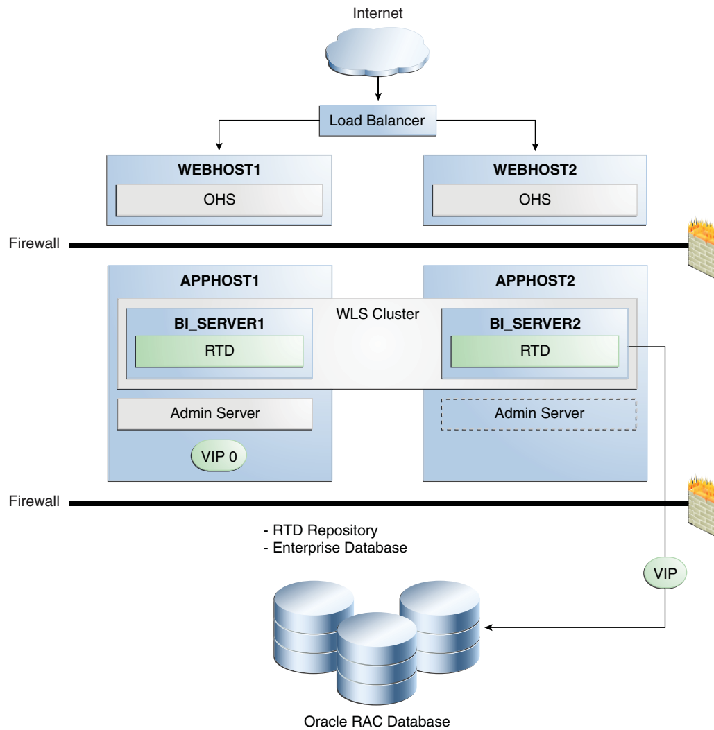
Figure 15–13 Oracle RTD High Availability Architecture
