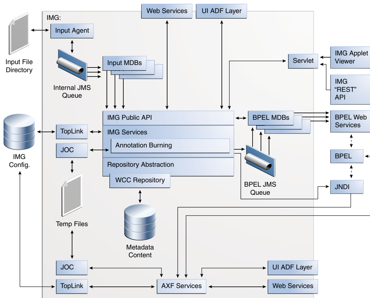
Figure 11-1 Imaging Components for a Single Instance
