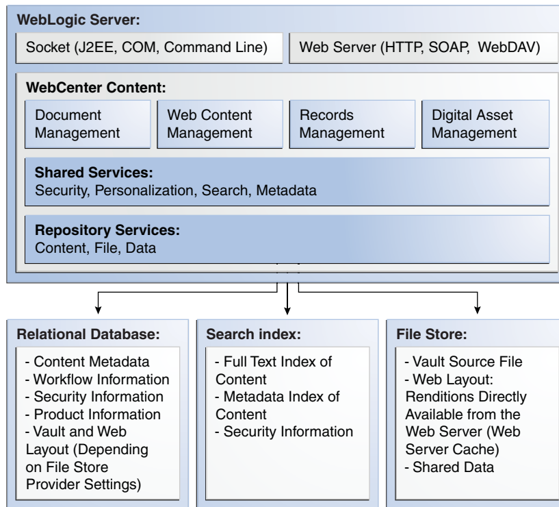
Figure 11–4 Oracle WebCenter Content Single Instance Architecture
