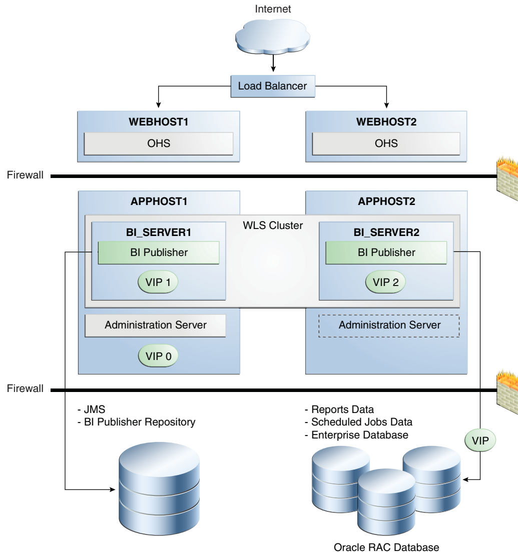
Figure 15–11 Oracle BI Publisher High Availability Architecture
