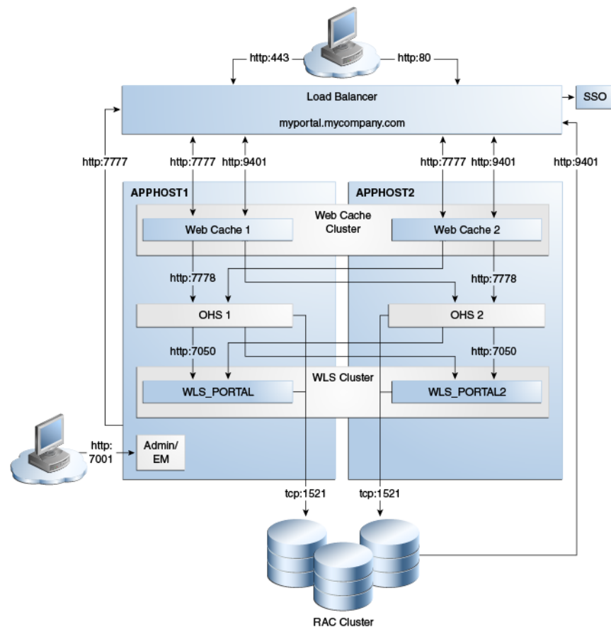
Figure 14–2 Oracle Portal High Availability Deployment
