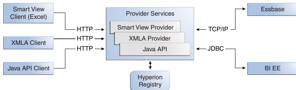
Figure 15–4 Provider Services Single Instance Architecture
