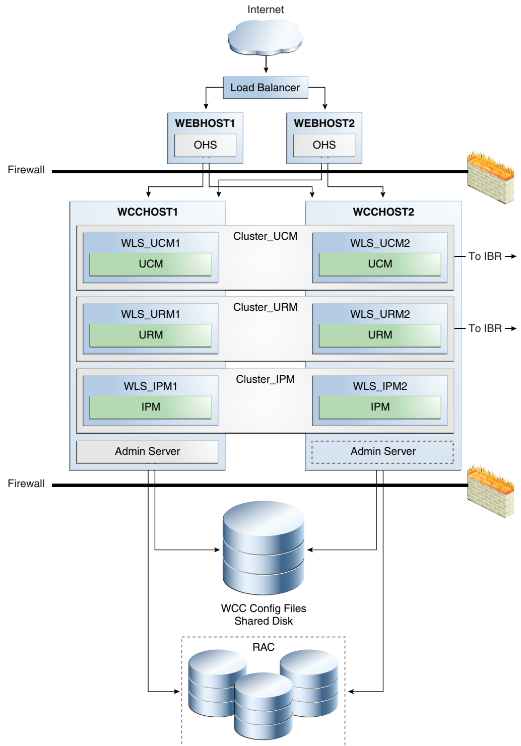
Figure 11–6 Oracle WebCenter Content High Availability Architecture
