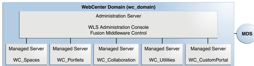
Figure 6-4 Basic Single-Node Oracle WebCenter Portal Architecture
