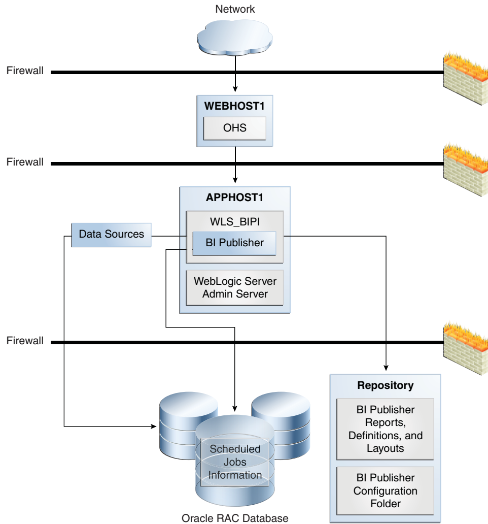
Figure 15–10 Oracle BI Publisher Single Instance Architecture
