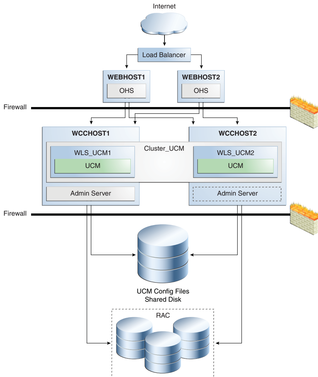
Figure 11–5 Oracle WebCenter Content Two-Node Cluster
