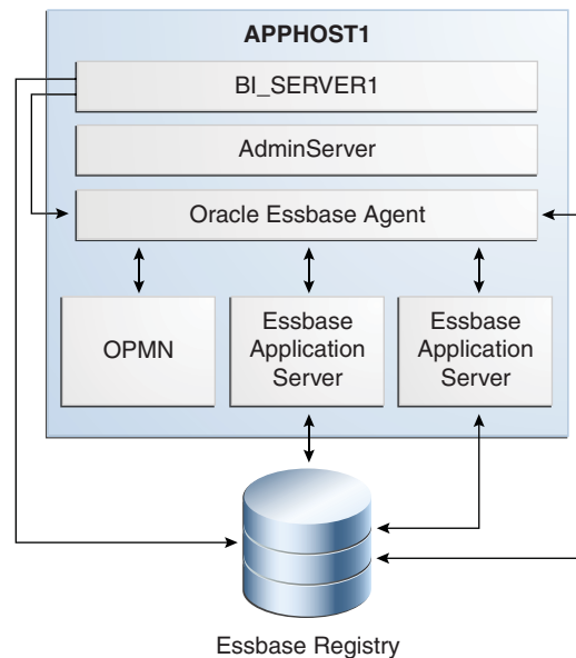
Figure 15-3 Oracle Essbase Single Instance Architecture
