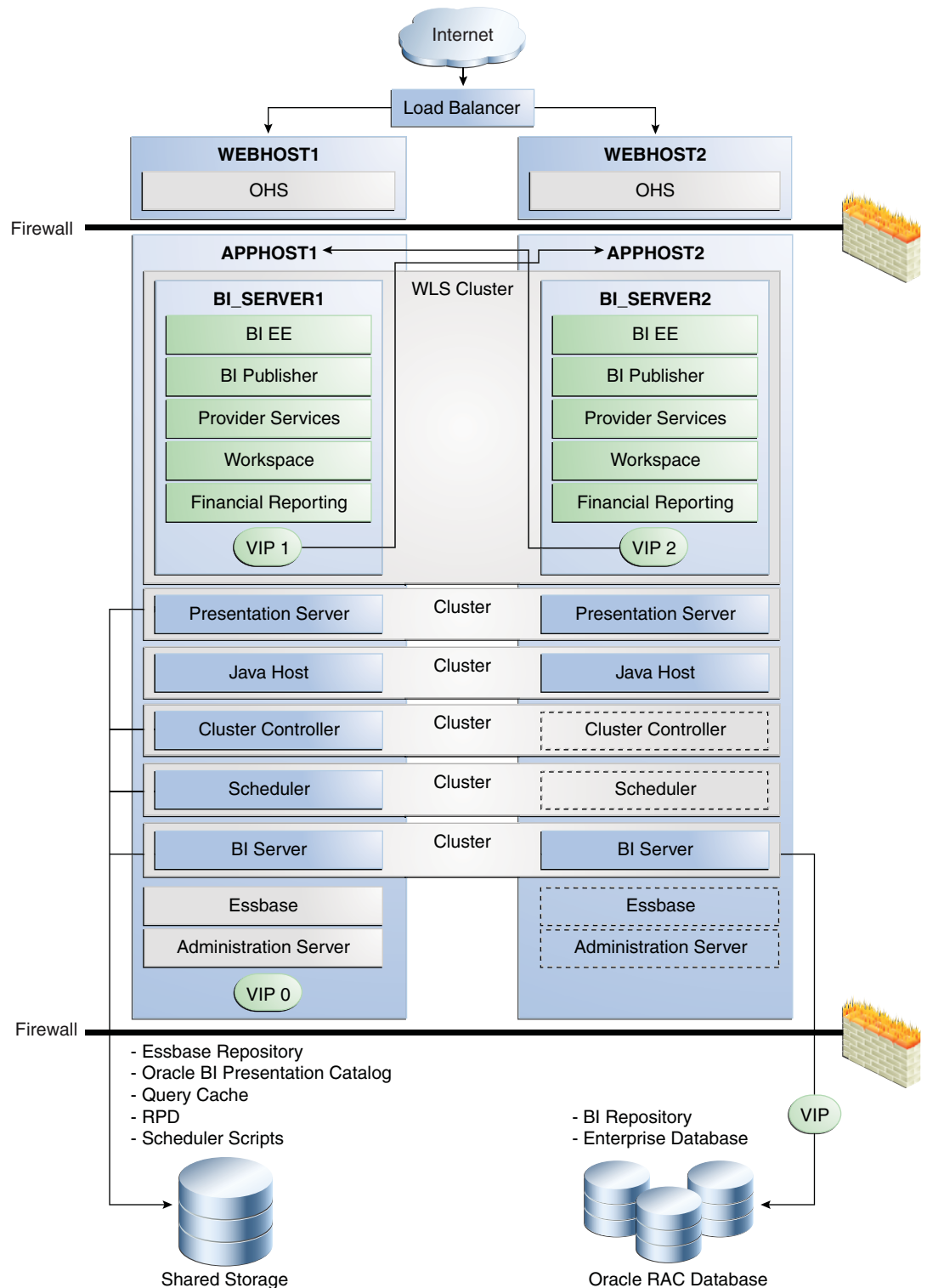
Figure 15–2 A Highly Available Oracle BI EE and EPM Deployment
