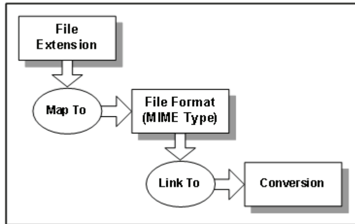
Figure 21–1 Mapping File Formats to a Conversion
