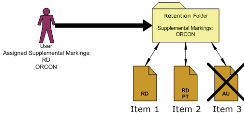
Figure 13–5 User Must Match At Least One Supplemental Marking
