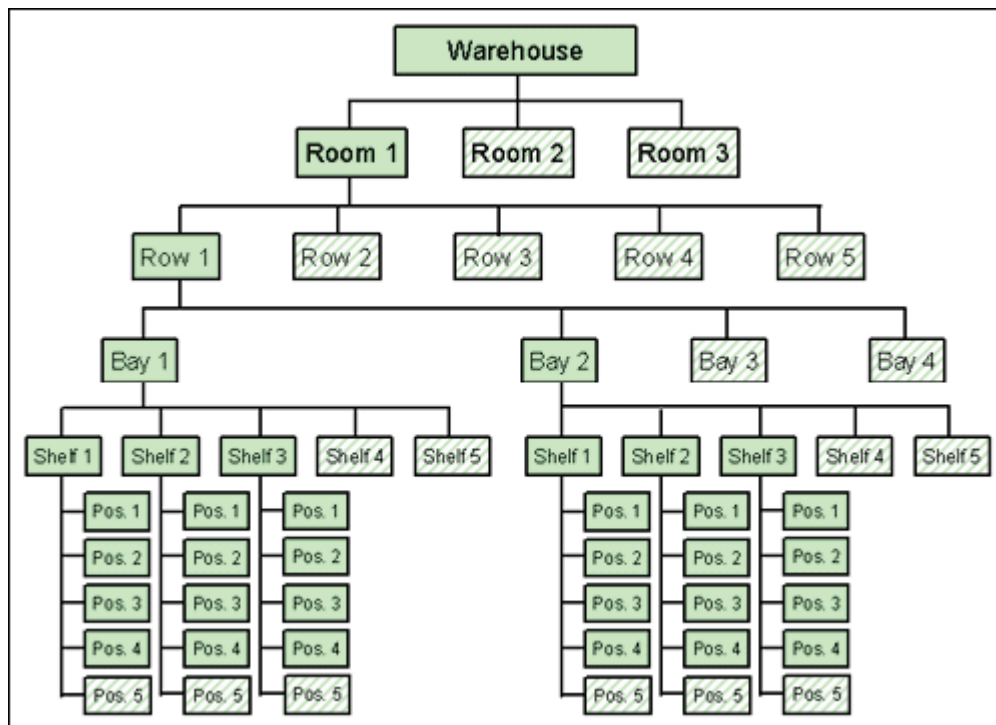
Figure 16–2 Example Storage Space Environment
