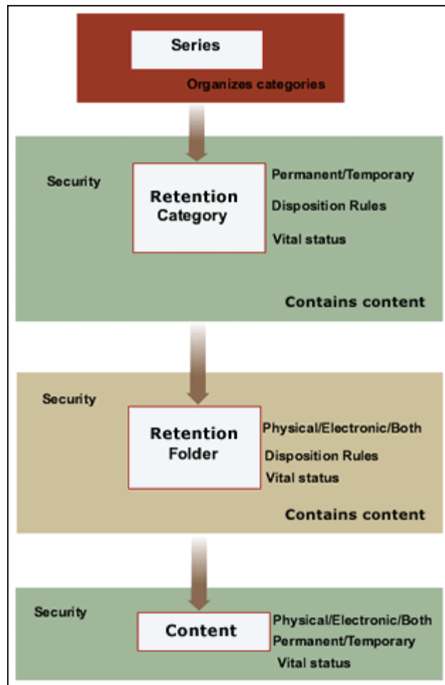
Figure 12–2 Attributes of Retention Schedule Objects
