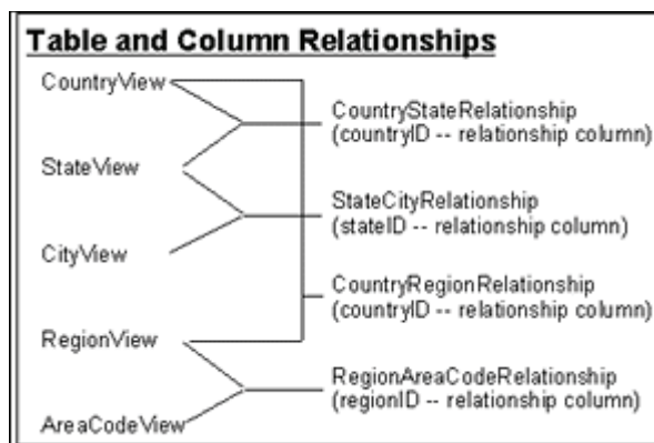
Figure 7-4 Table and Column Relationships
