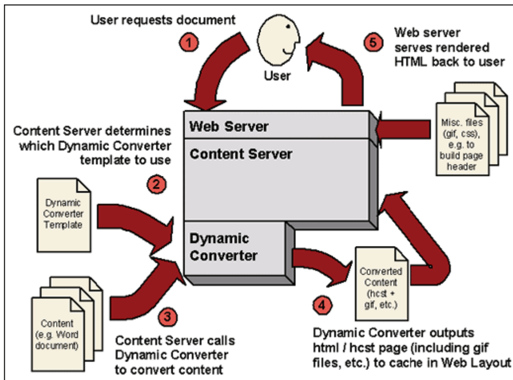
Figure 27–1 Basic Dynamic Converter Process
