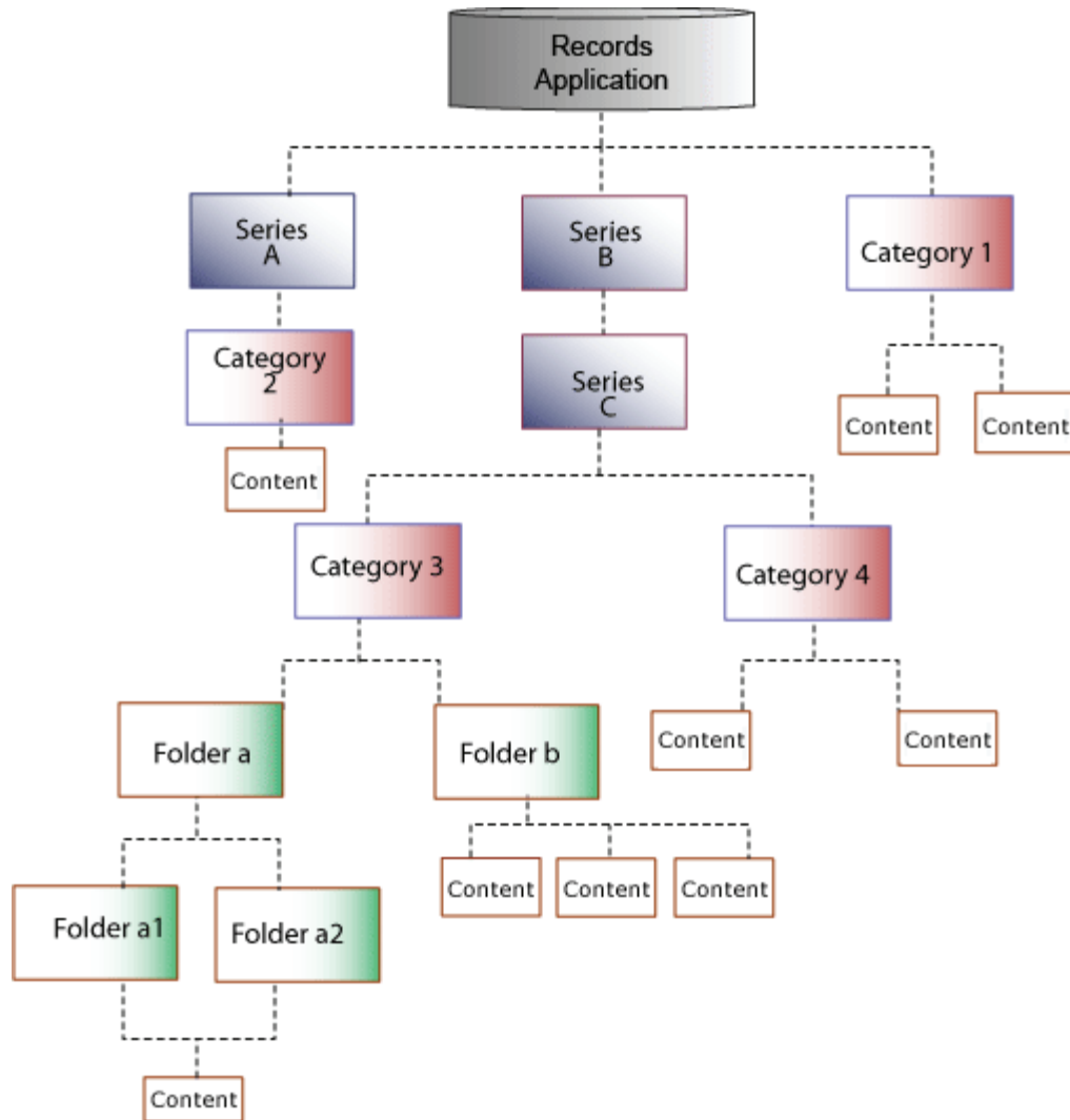
Figure 12-3 Sample Retention Schedule Hierarchy
