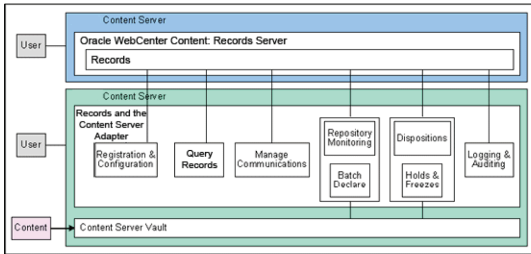
Figure 15–1 Content Server Adapter Retention Functions Overview
