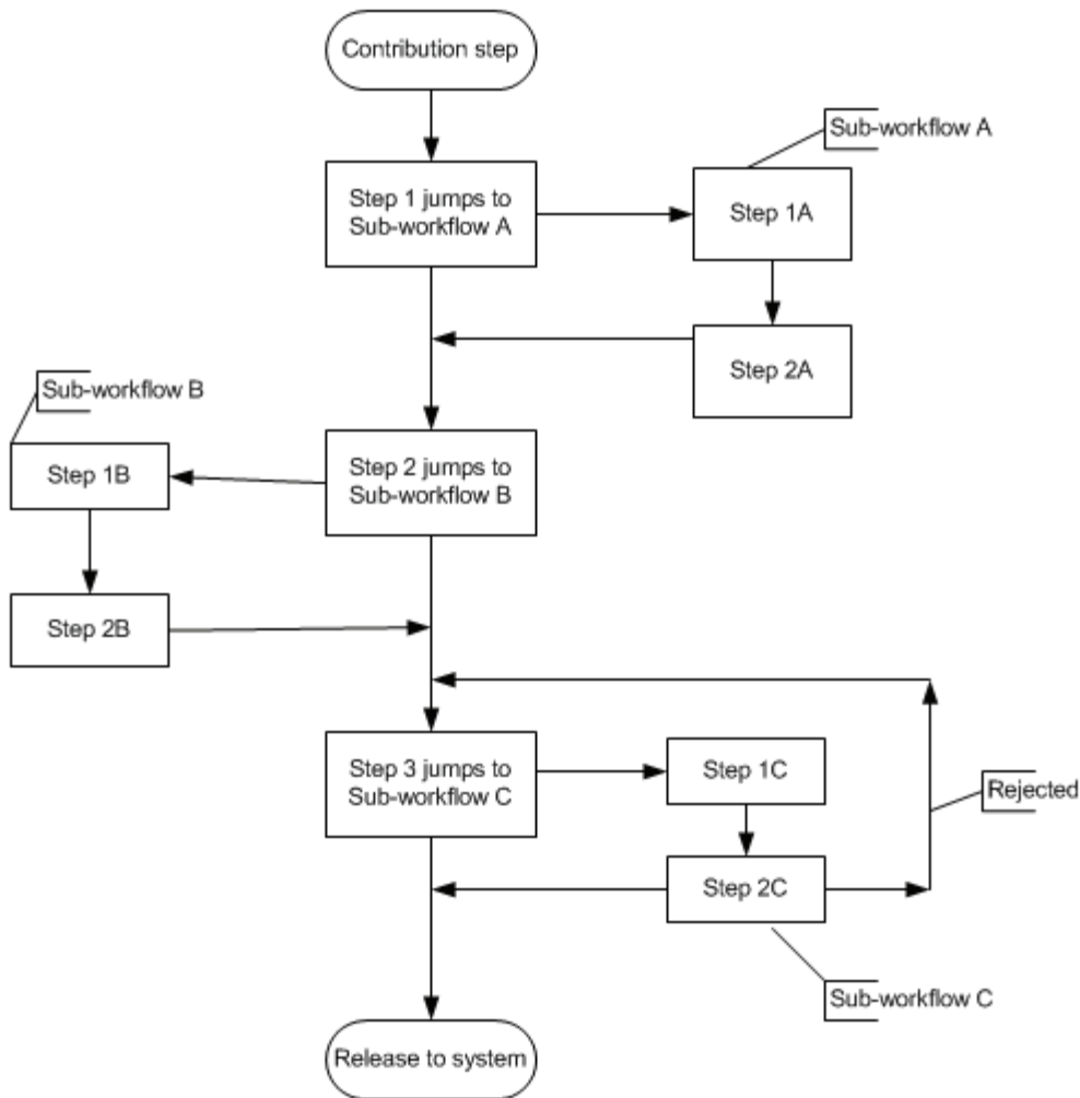
Figure 6–4 Sample Jump Flowchart
