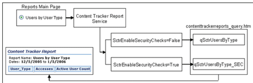
Figure 9–2 Report Query Selection Process
