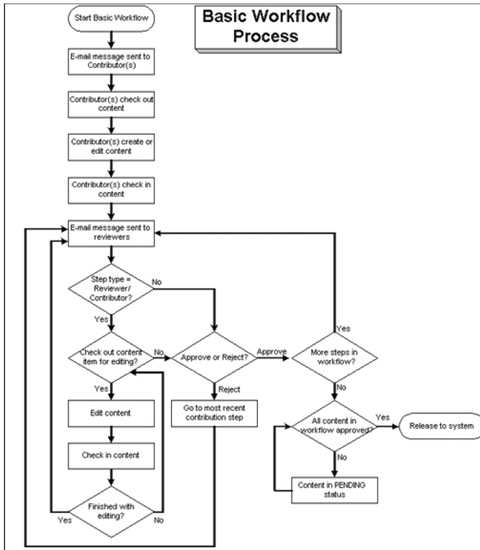
Figure 6–2 Basic Workflow Process
