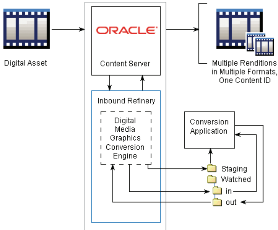
Figure 24–1 Rendering a Video Asset
