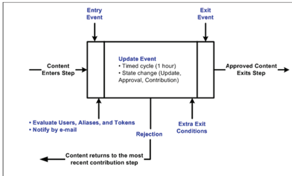
Figure 6–3 Jumps and Events
