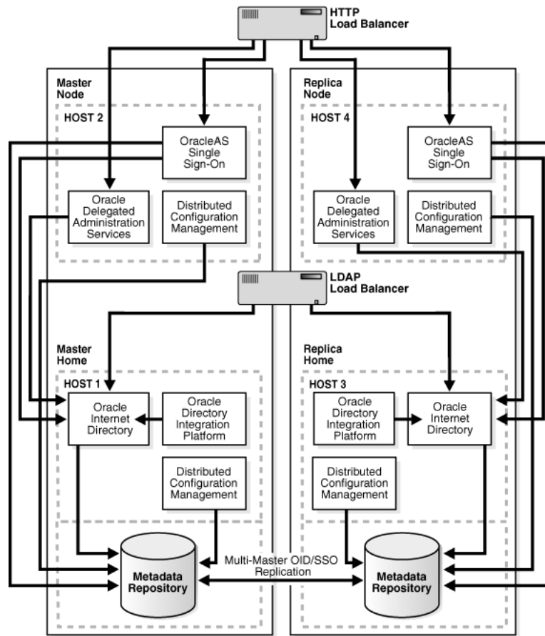
Figure 10–1 A Typical Oracle Identity Management 10g Release 2 (10.1.2) Multimaster Replication Environment
