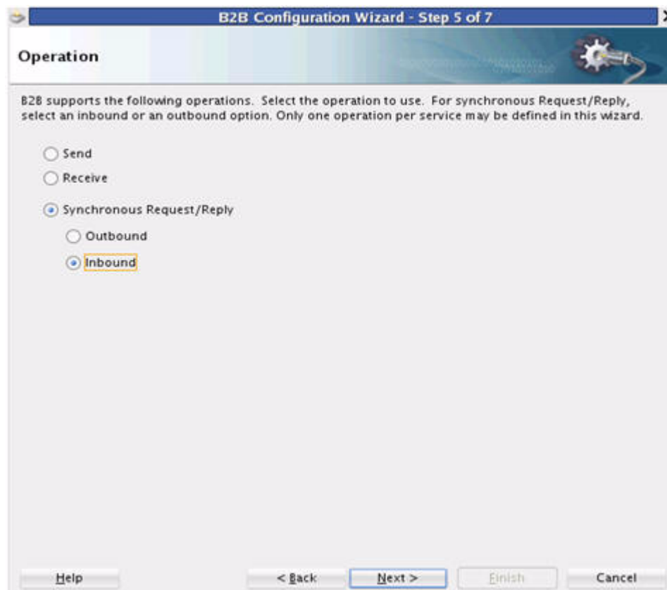
Figure C-6 B2B Configuration Wizard: Operation Page
