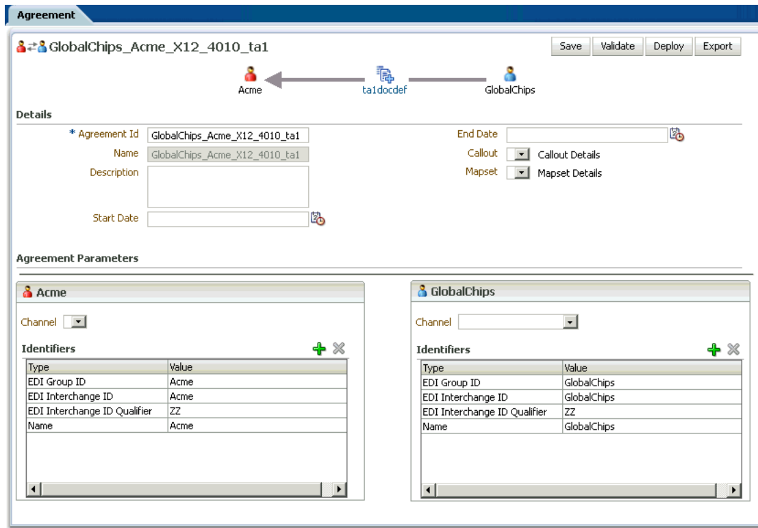
Figure K-3 A Sample TA1 Agreement
