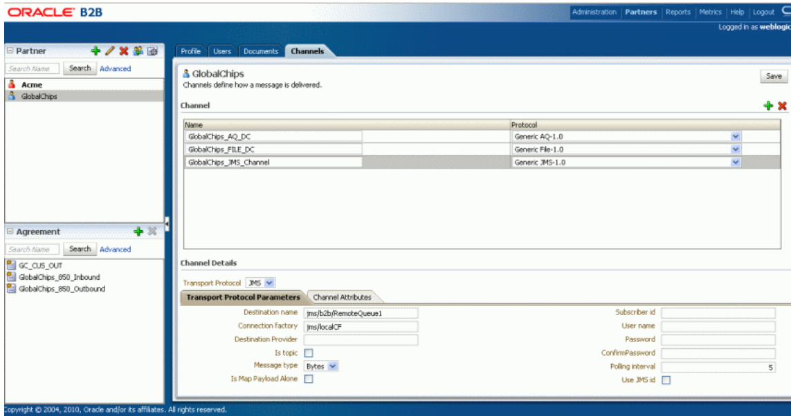
Figure G-6 Creating a JMS Channel in the B2B User Interface
