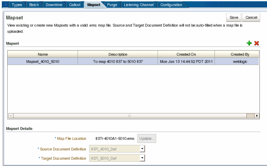
Figure 14–2 Mapset Defined in the Oracle B2B Console
