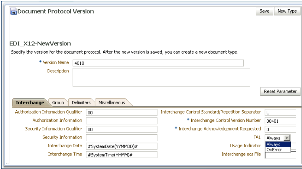
Figure K-4 Configuring TA1
