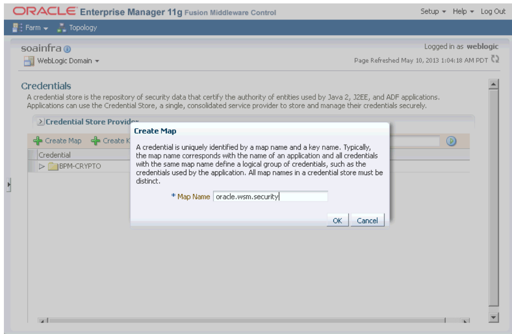
Figure 22–6 Create Map Dialog Box
