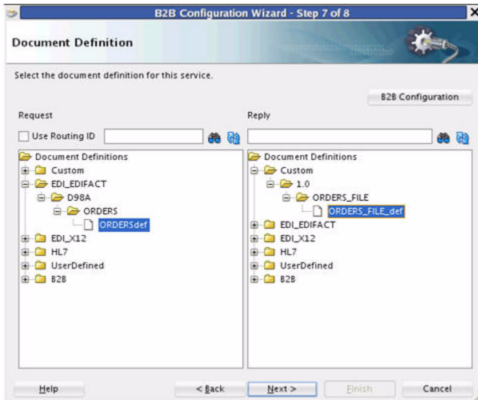
Figure C-7 B2B Configuration Wizard: Document Definition Page
