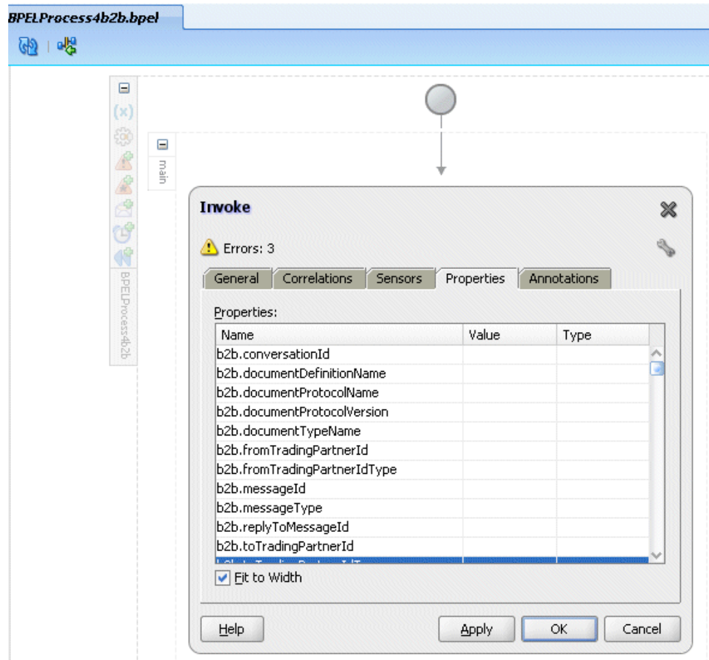
Figure E-1 Invoke Activity Showing B2B Normalized Message Properties
