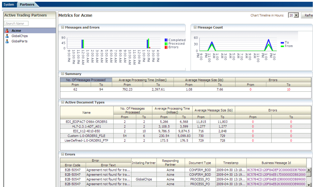
Figure 19–5 Partner Metrics
