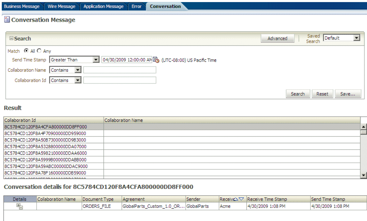
Figure 18–9 Conversation Report
