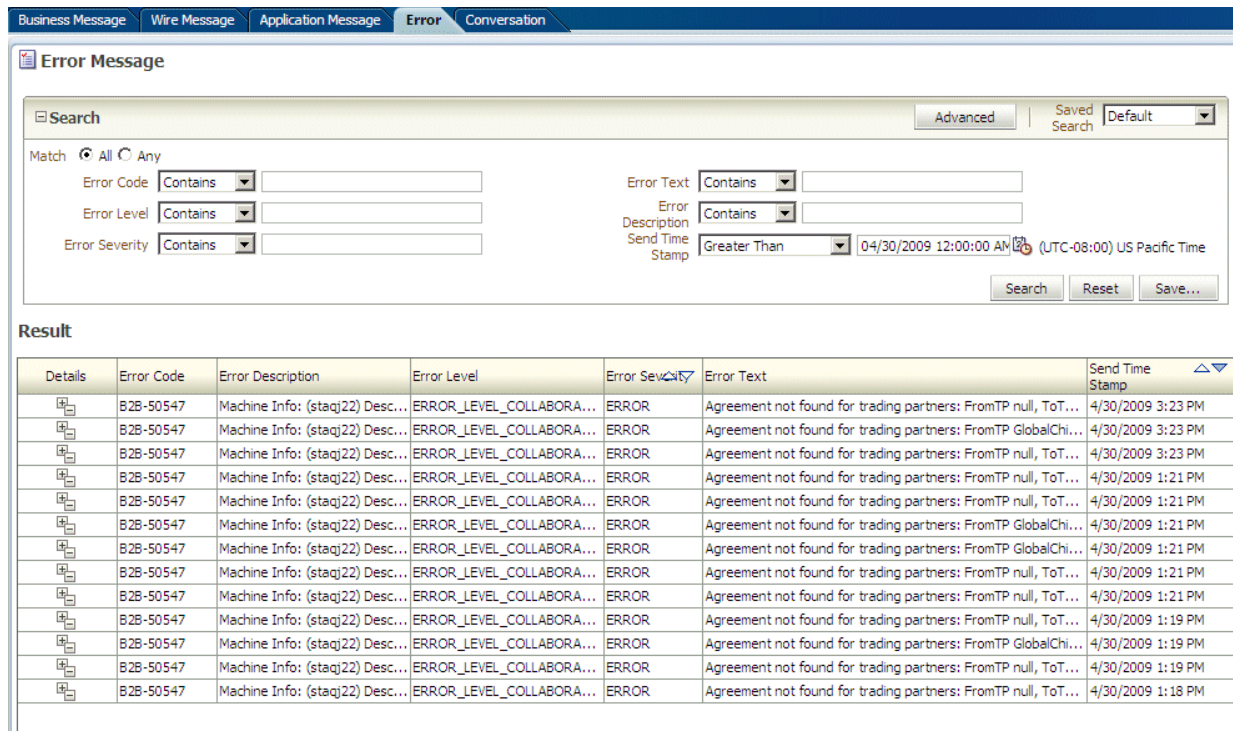
Figure 18–7 Error Report
