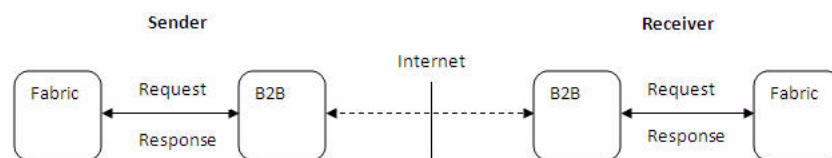
Figure C-1 Synchronous Request/Reply
