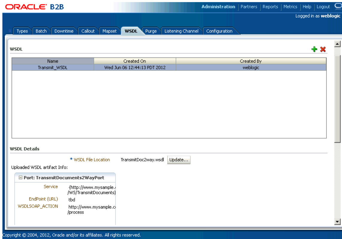
Figure 22–1 WSDL Artifacts
