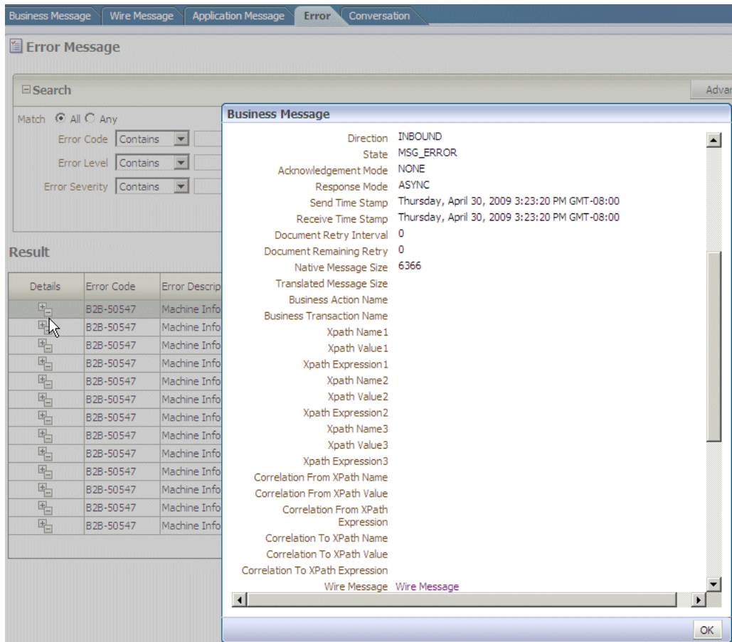
Figure 18–8 Error Reports
