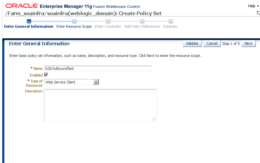
Figure 22–9 Create Policy Set - Enter General Information Page
