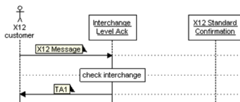
Figure K-1 TA1 acknowledgment
