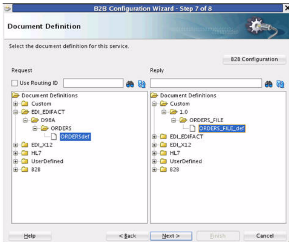
Figure C-3 B2B Configuration Wizard: Document Definition Page
