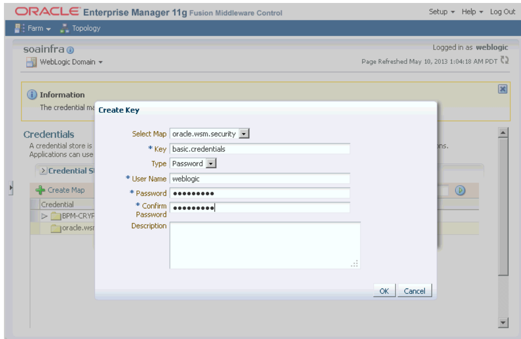
Figure 22–7 Create Key Dialog Box
