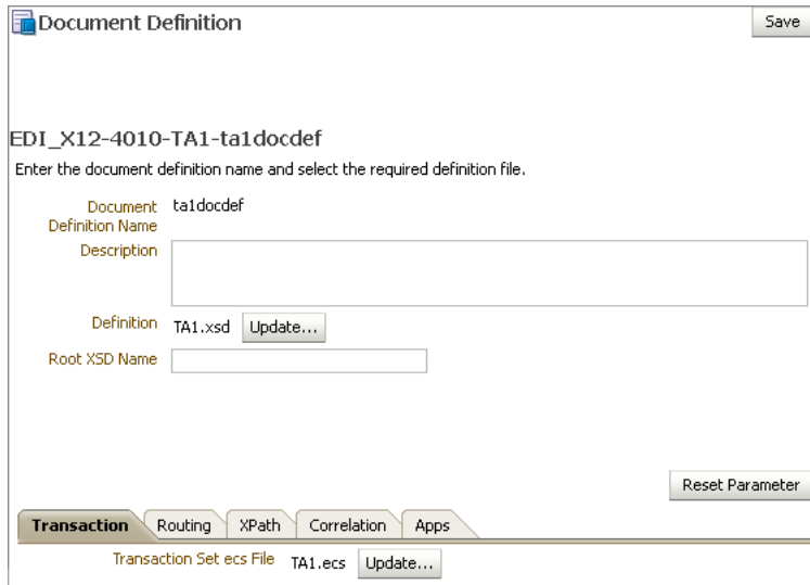
Figure K-2 A Sample TA1 Document Definition
