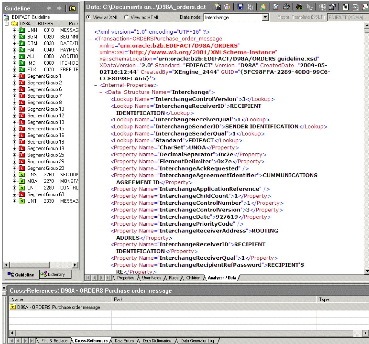
Figure 3–18 Analyzer Data
