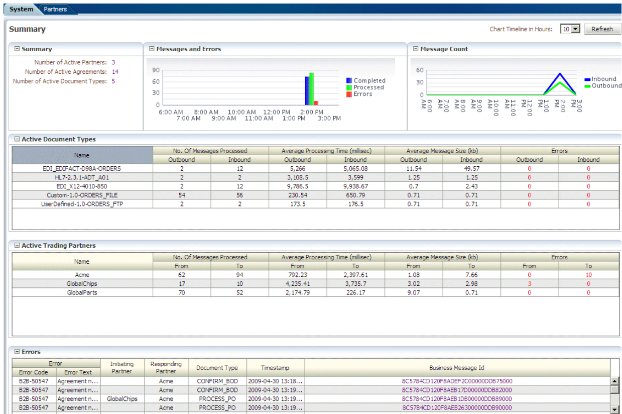
Figure 19–4 System Metrics
