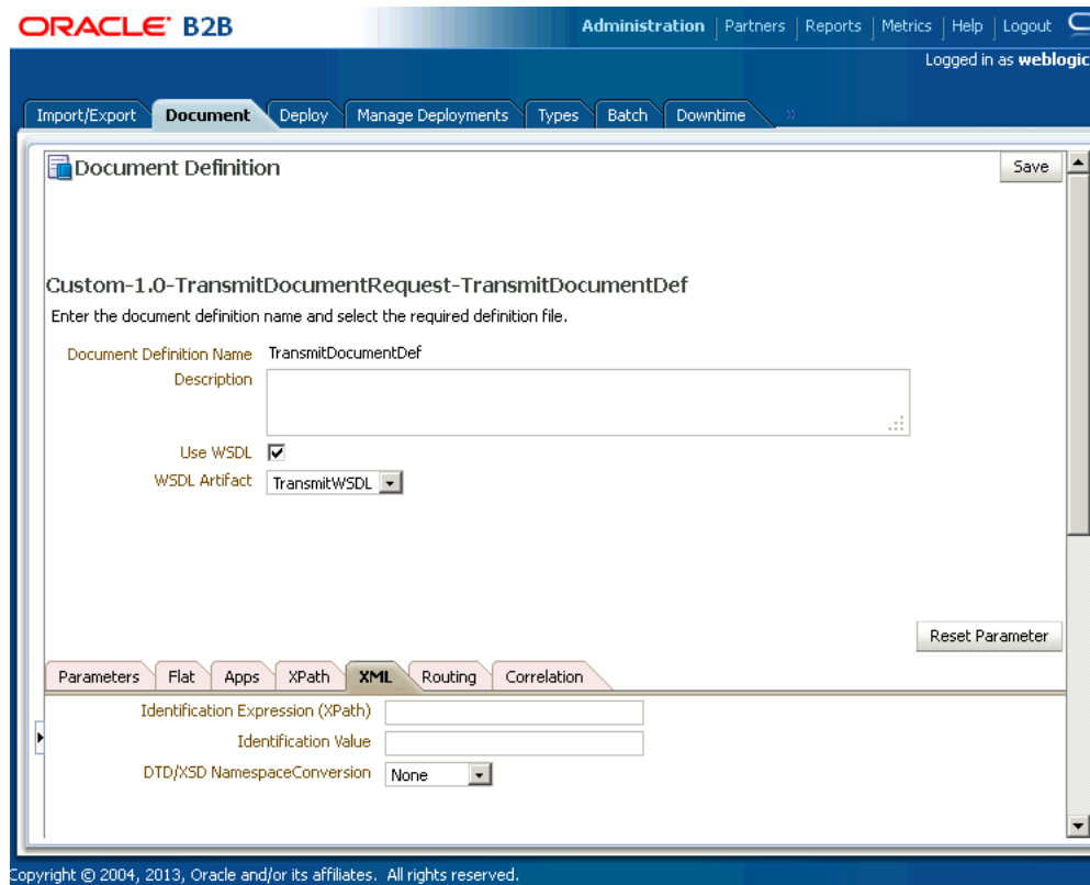
Figure 22–2 Creating Documents
