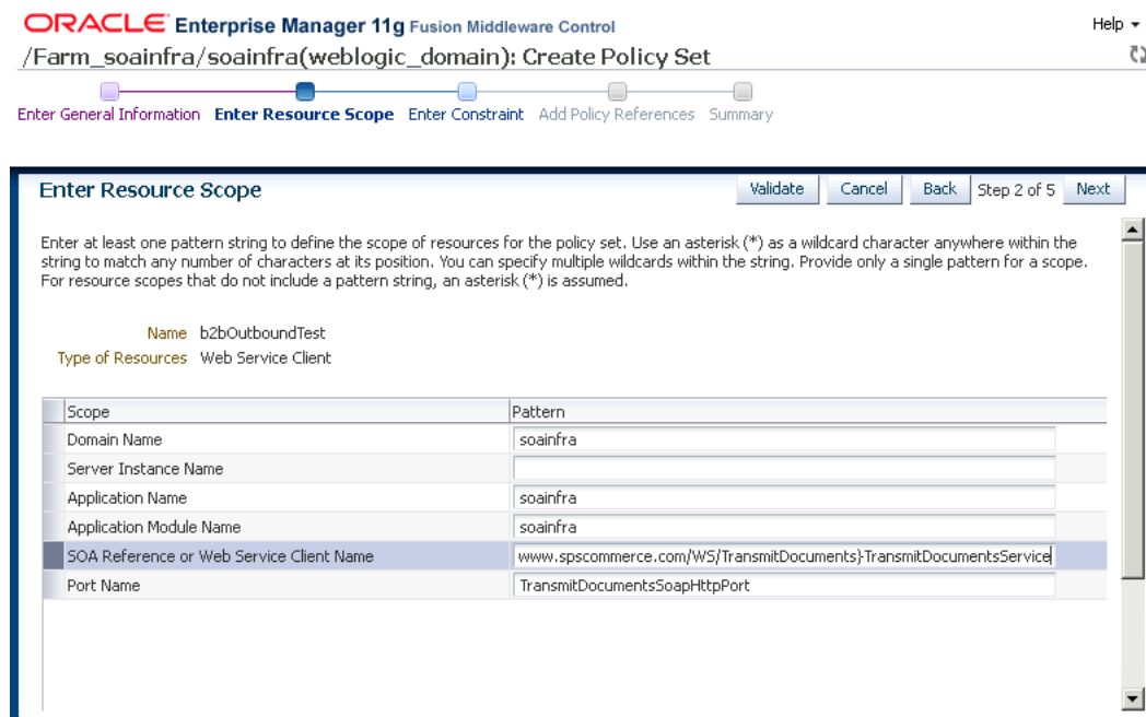
Figure 22–10 Create Policy Set - Enter Resource Scope Page
