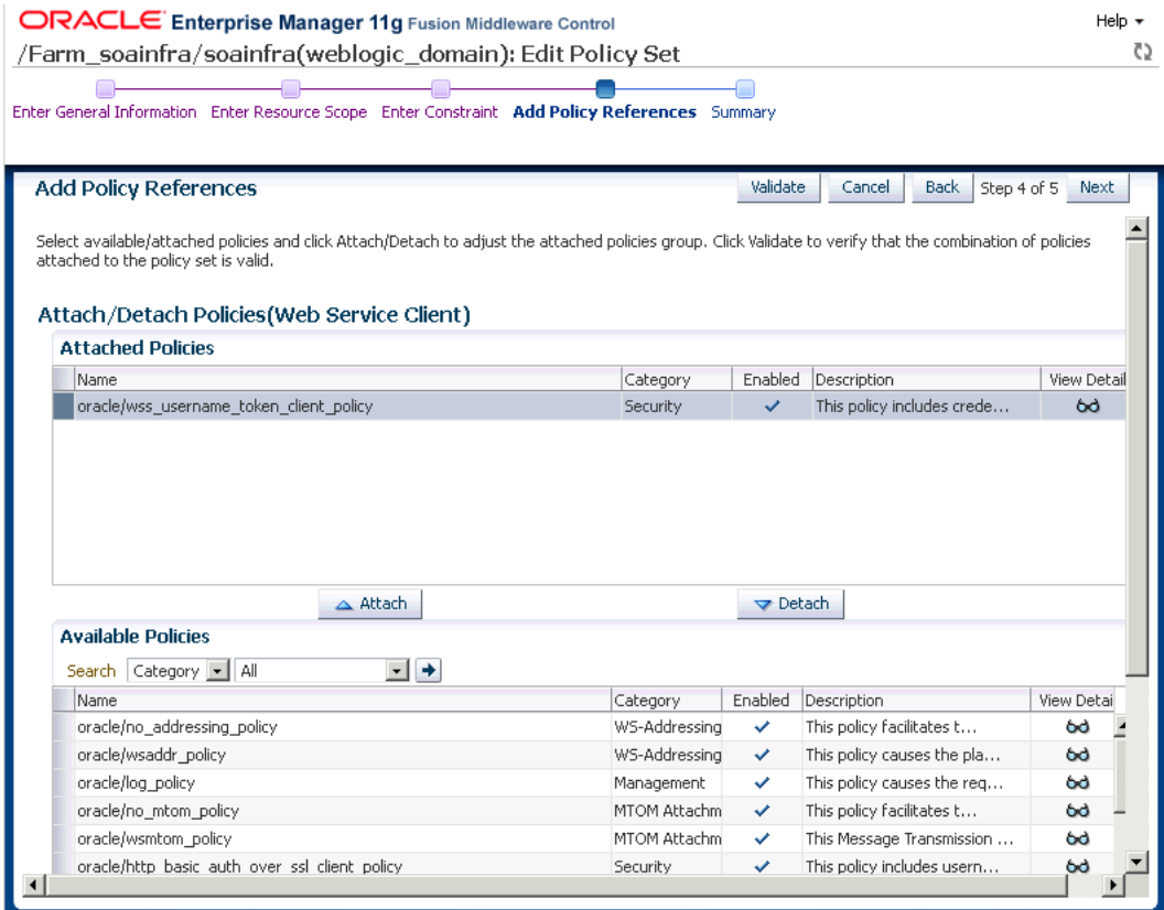
Figure 22–11 Create Policy Set - Add Policy References Page
