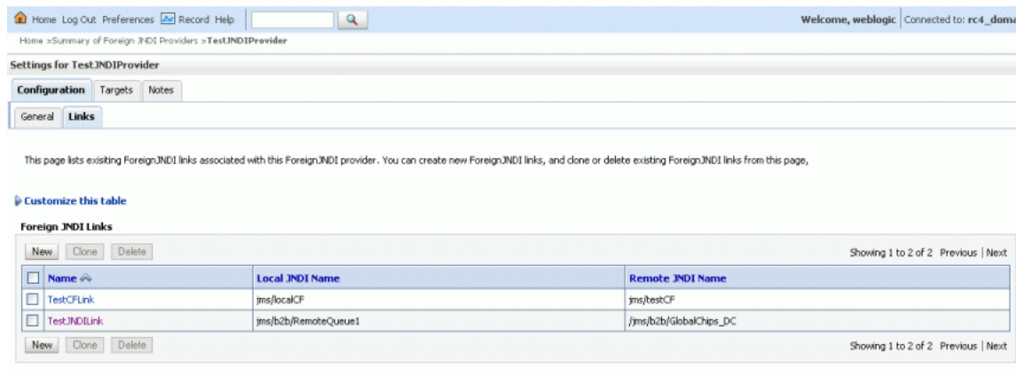
Figure G-5 Foreign JNDI Links
