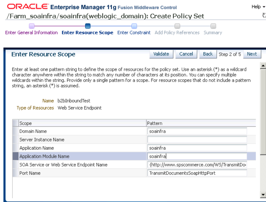
Figure 22–13 Create Policy Set - Enter Resource Scope Page
