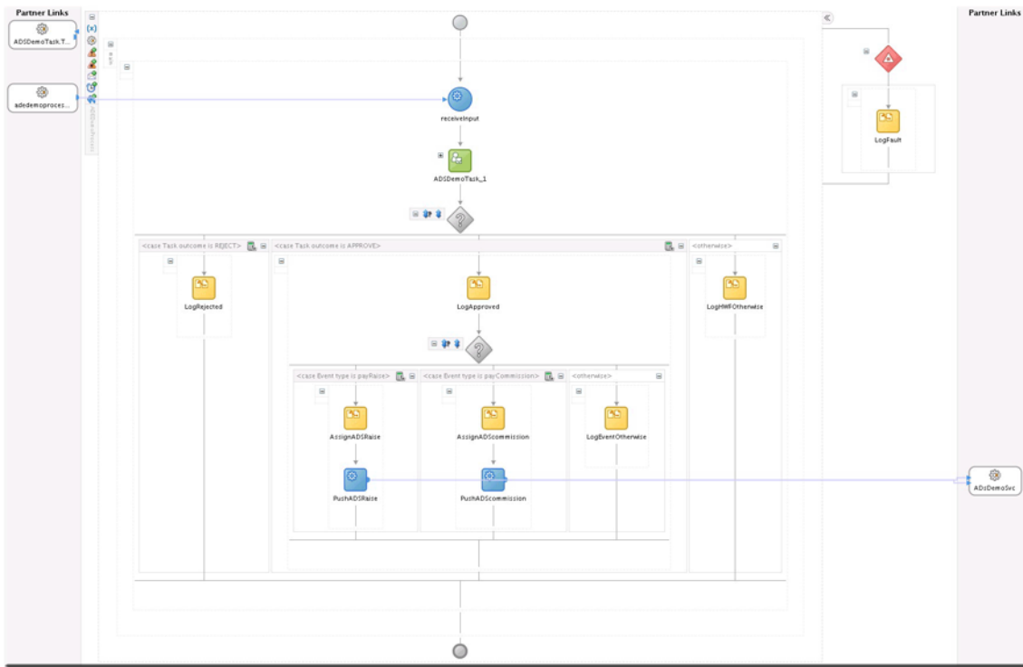
Figure 43–4 BPEL Flow
