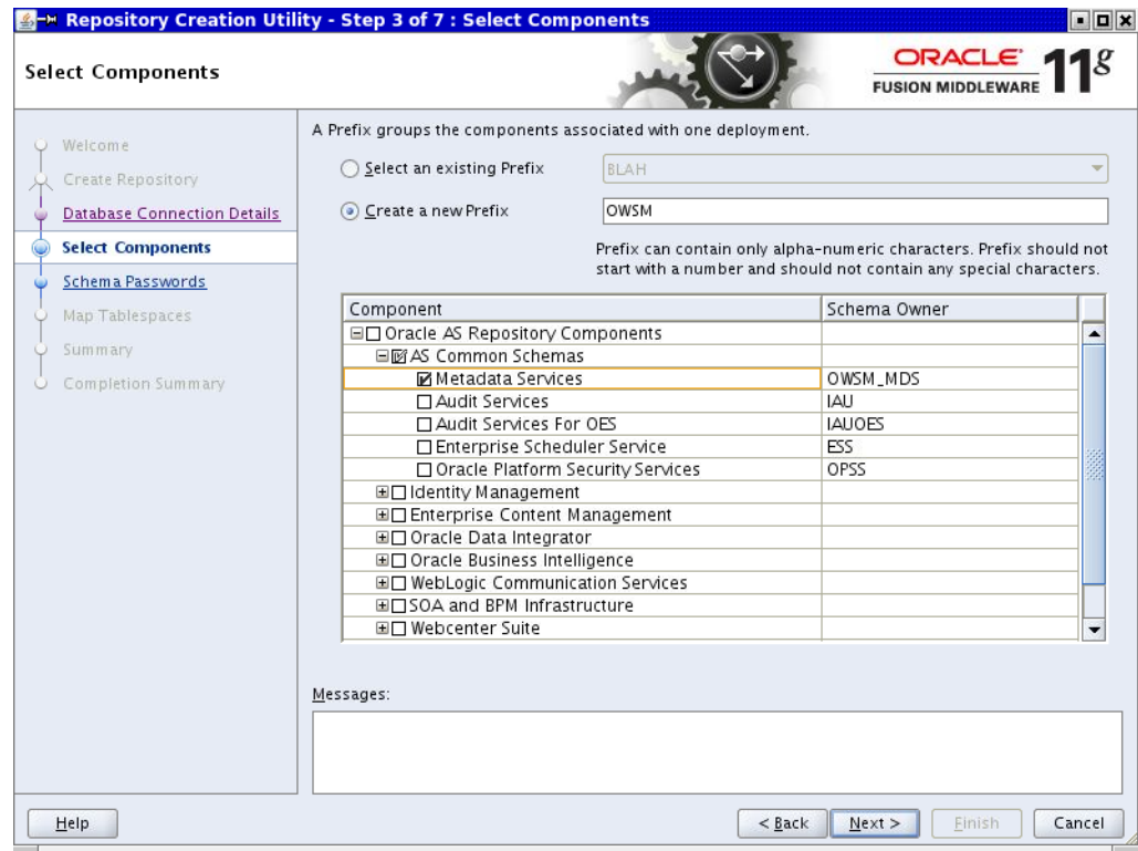
Figure 2–34 Selecting Components
