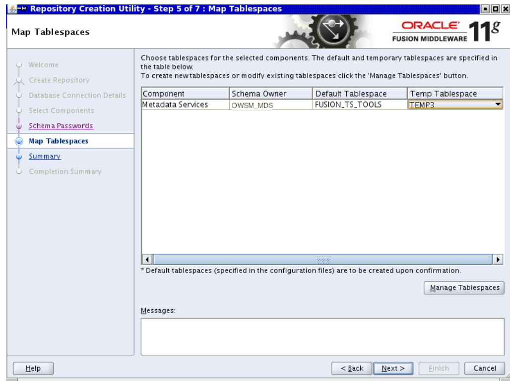
Figure 2–37 Mapping Tablespaces
