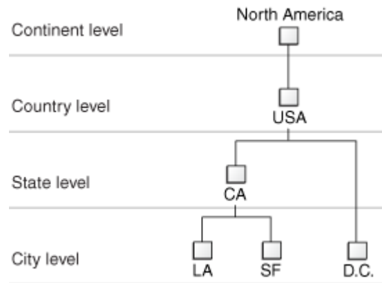
Figure 19–78 Leaf-to-Root Order
