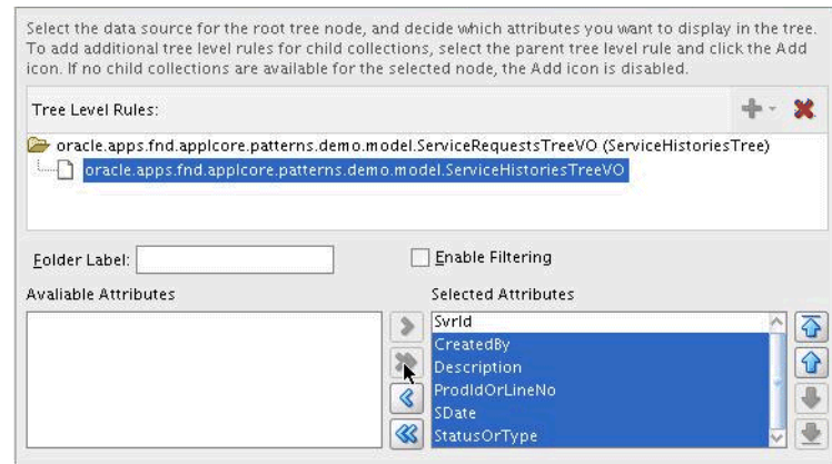
Figure 16–23 Selecting Attributes
