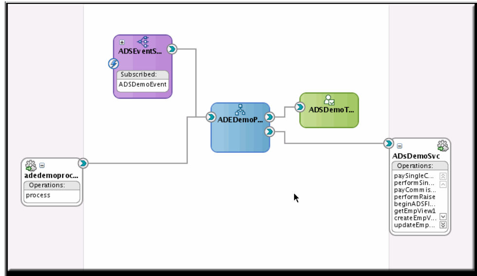
Figure 43–3 Pattern Composite
