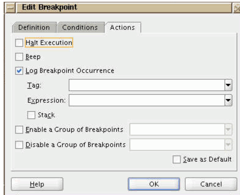
Figure 58–11 Edit Breakpoint
