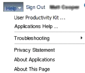
Figure 13–27 Help Menu
