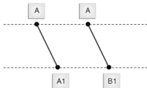
Figure 19–76 Flattening Delta
