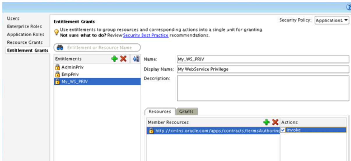
Figure 5–4 Entitlement Grants
