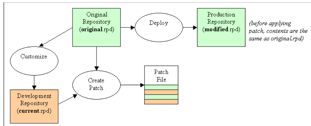
Figure 17–7 Development-to-Production: Creating the Patch
