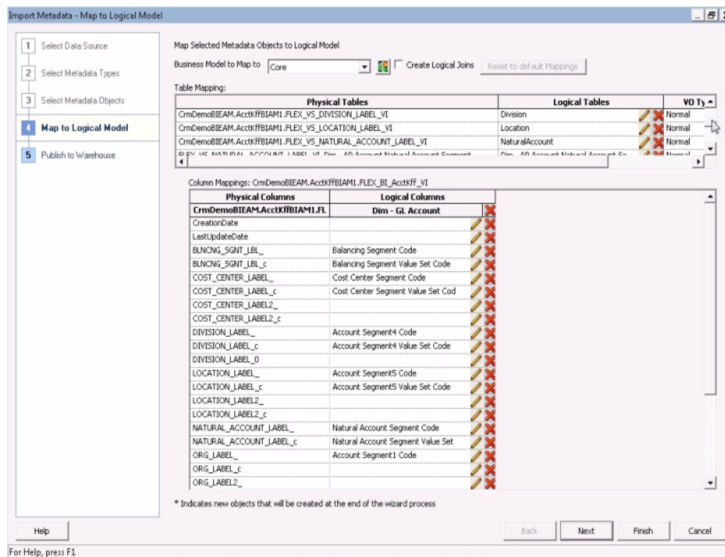
Figure 6–3 Map to Logical Model Screen of Import Metadata Wizard
