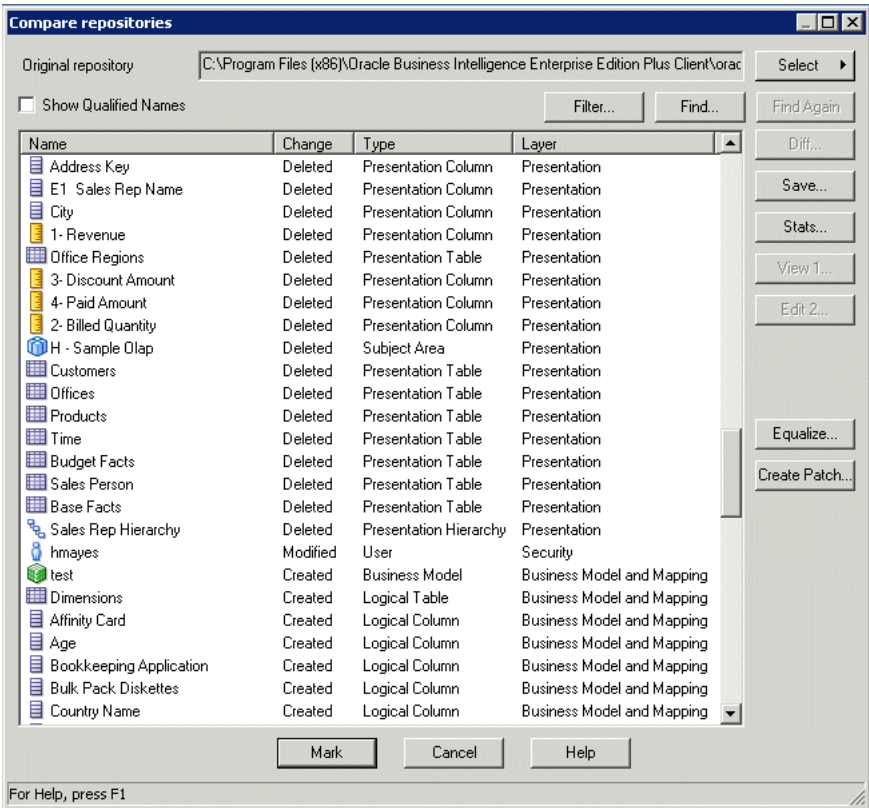
Figure 17–1 Compare Repositories Dialog
