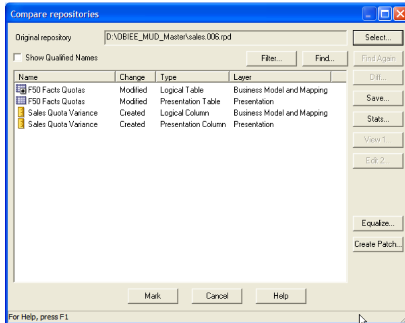
Figure B-7 Compare Repositories Dialog for sales.rpd and sales.006.rpd
