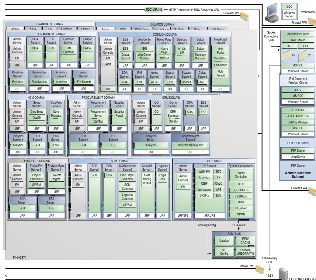
Figure A–2 Administrative Subnet Topology Details
