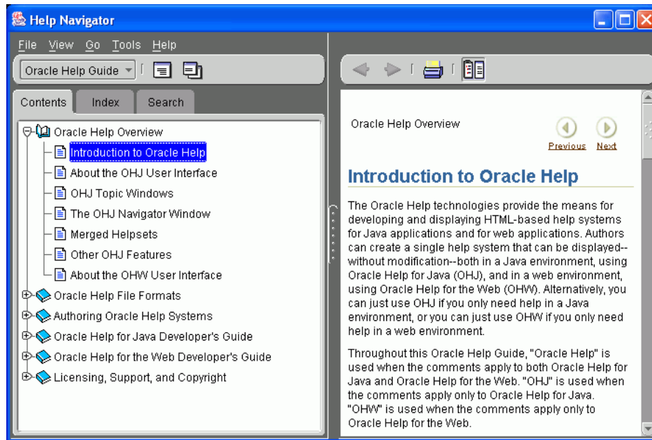
Figure 2-2 Docked Windows
