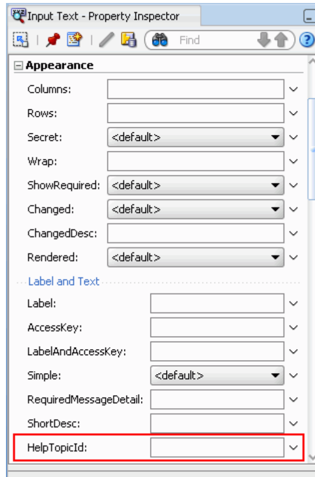
Figure 19–2 HelpTopicId Attribute
