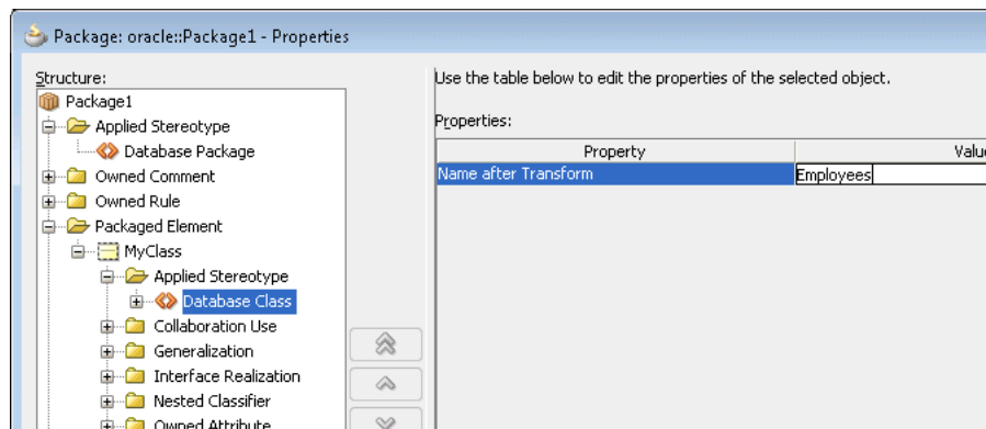
Figure 22–28 Stereotype Properties
