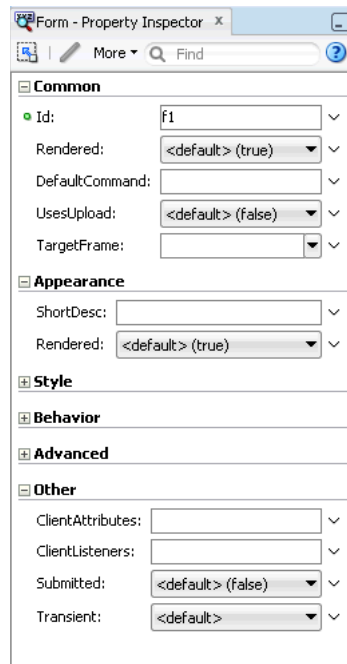
Figure 11–6 Property Inspector
