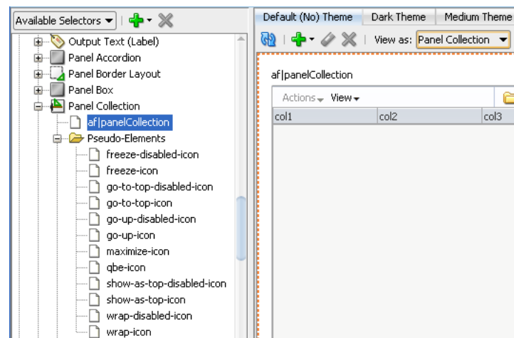
Figure 2–4 Panel Collection Pseudo-Elements for Icon Images
