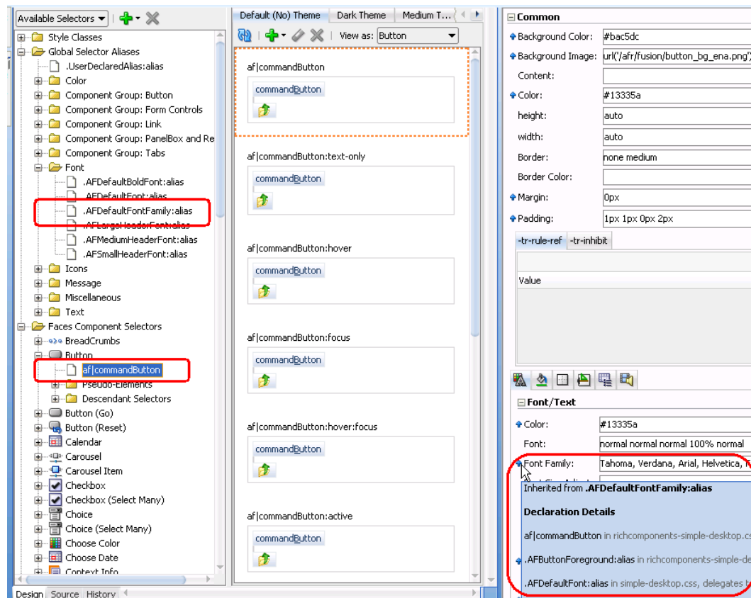
Figure 8–1 Component Selector Inheriting Value from Global Selector Alias
