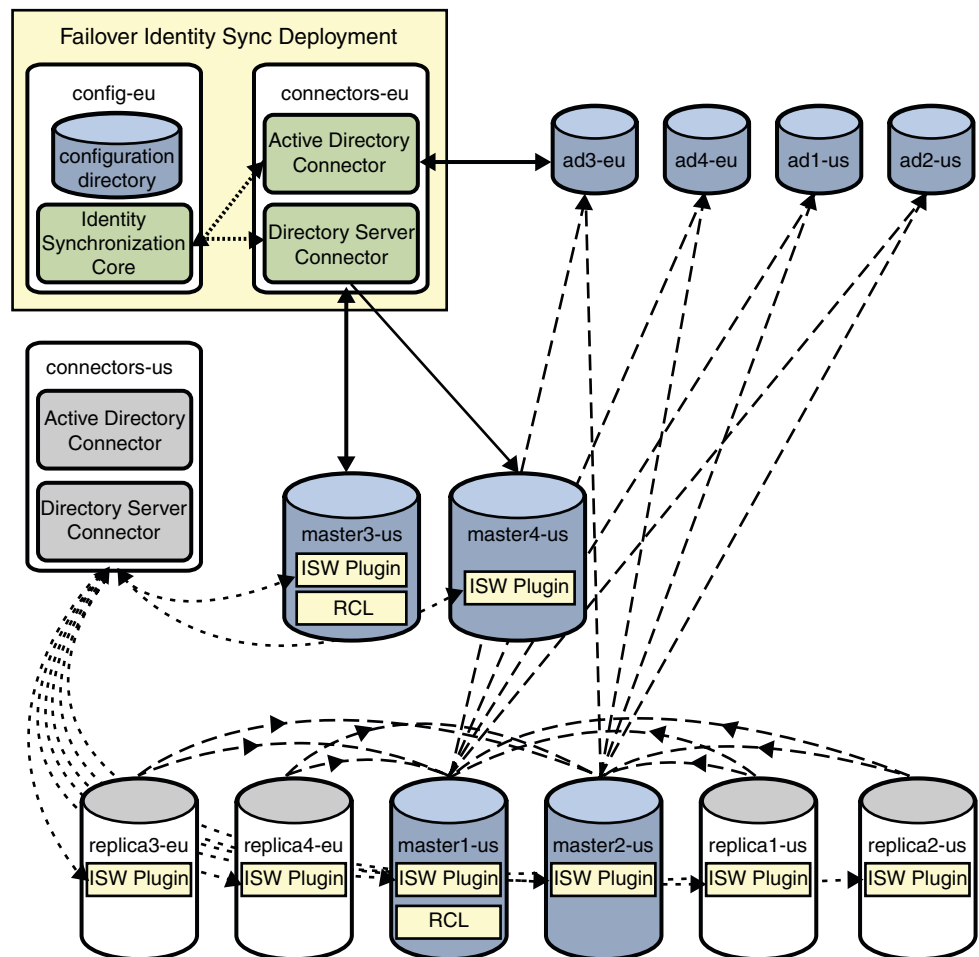
FIGURE 3-4 Failover Installation while the Primary Installation is Active
