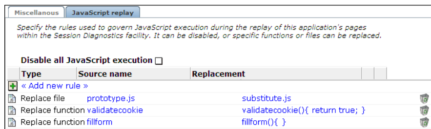
Figure 8–41 JavaScript Replay Rules
