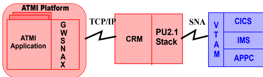
Figure 1-1 Tuxedo Mainframe Adapter for SNA Architecture
