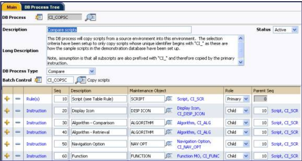
Figure 6: A DB Process With 6 Instructions
