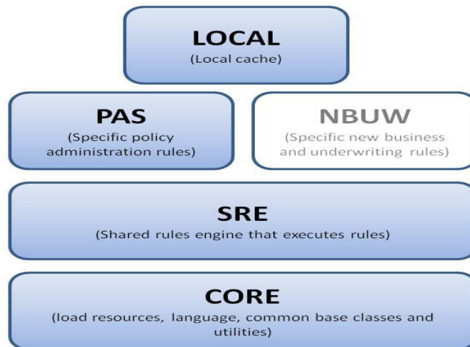
Cache Regions
