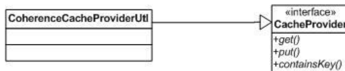
Coherence CacheProviderUtl
