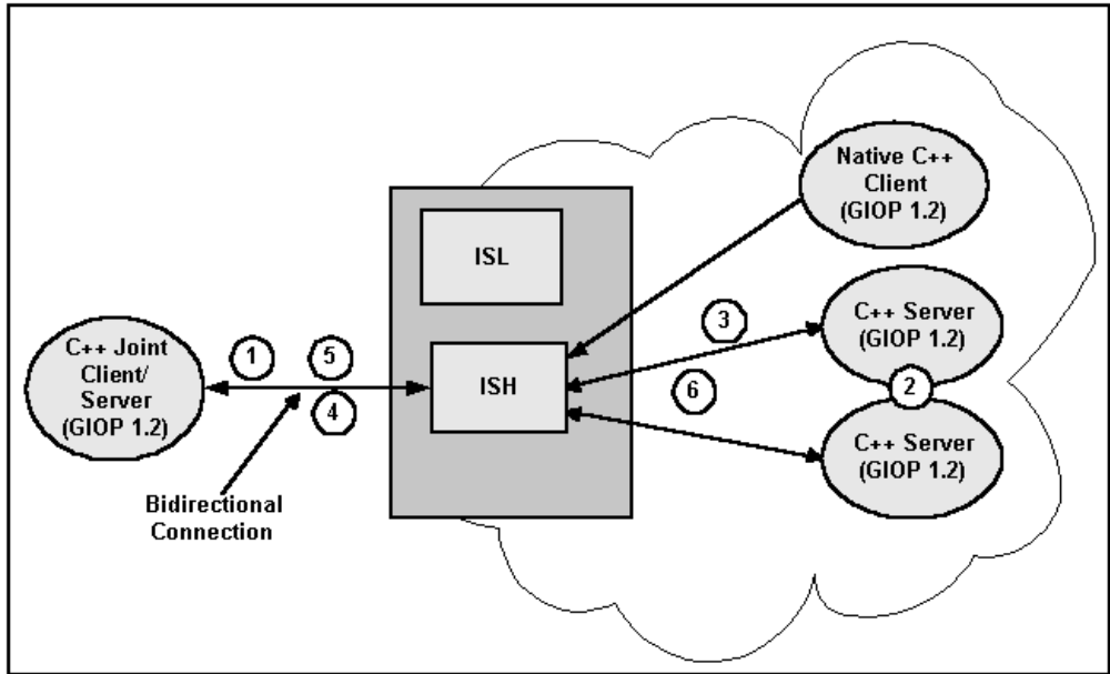
Figure 15-3 Bidirectional Connection
