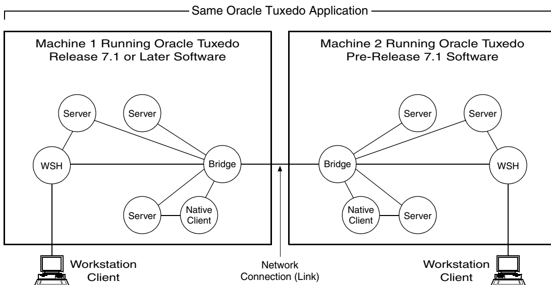
Figure 1-13 Intra-Domain Interoperability
