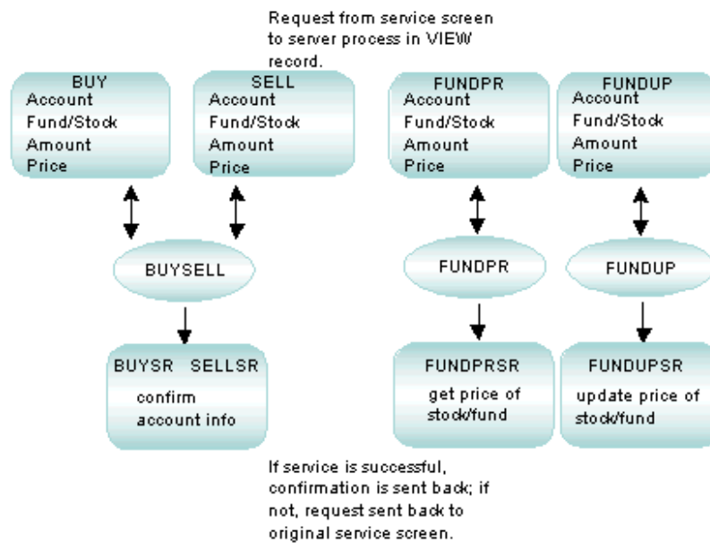
Figure 5-1 STOCKAPP Requests
