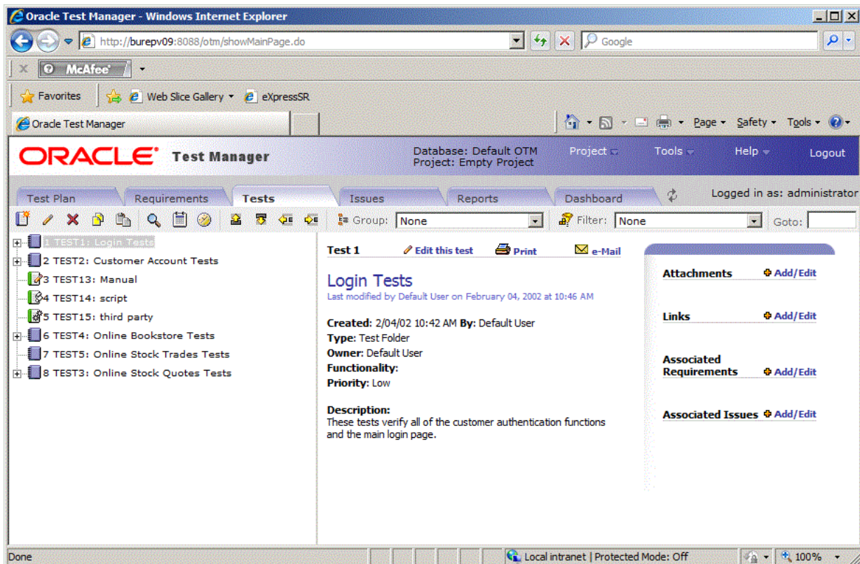
Figure 2–26 Tests Tab
