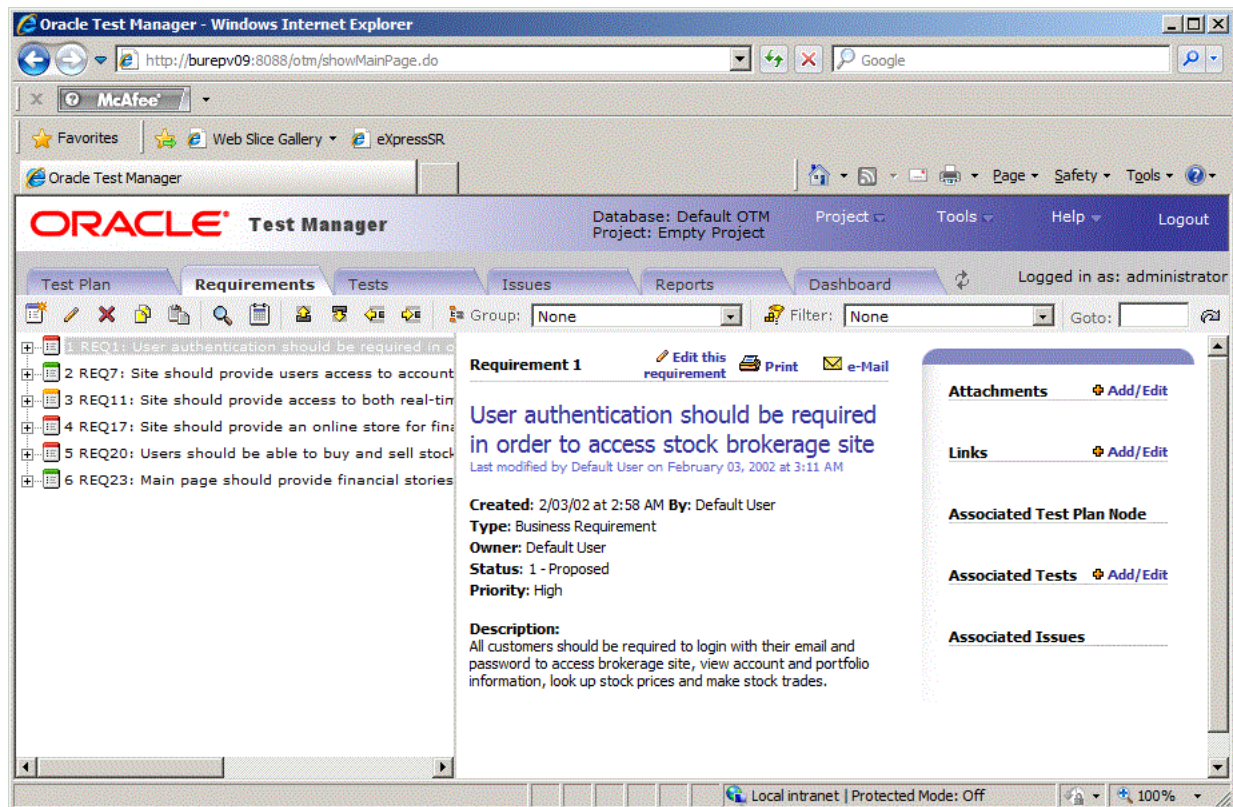
Figure 2-25 Requirements Tab
