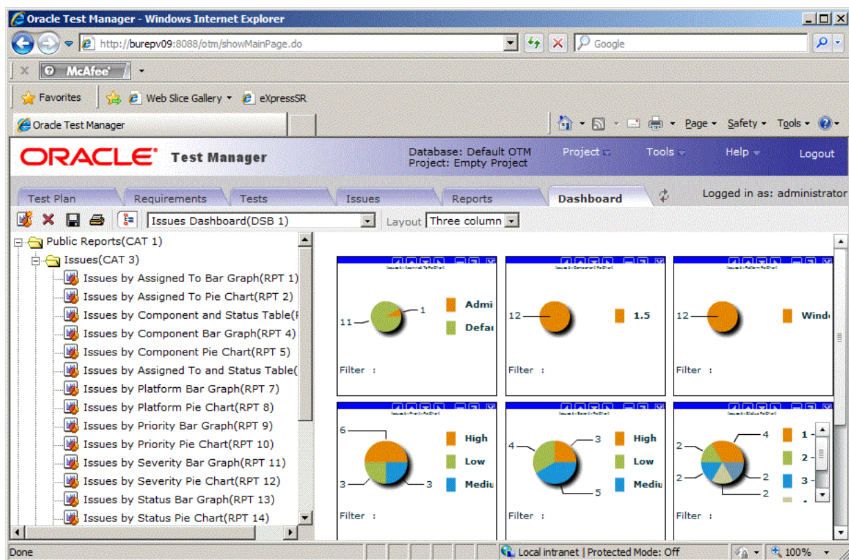
Figure 2–29 Dashboard Tab
