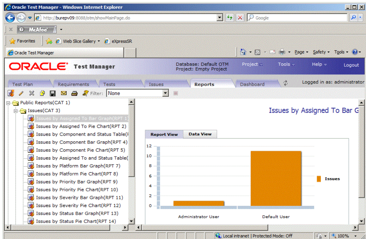
Figure 2–28 Reports Tab
