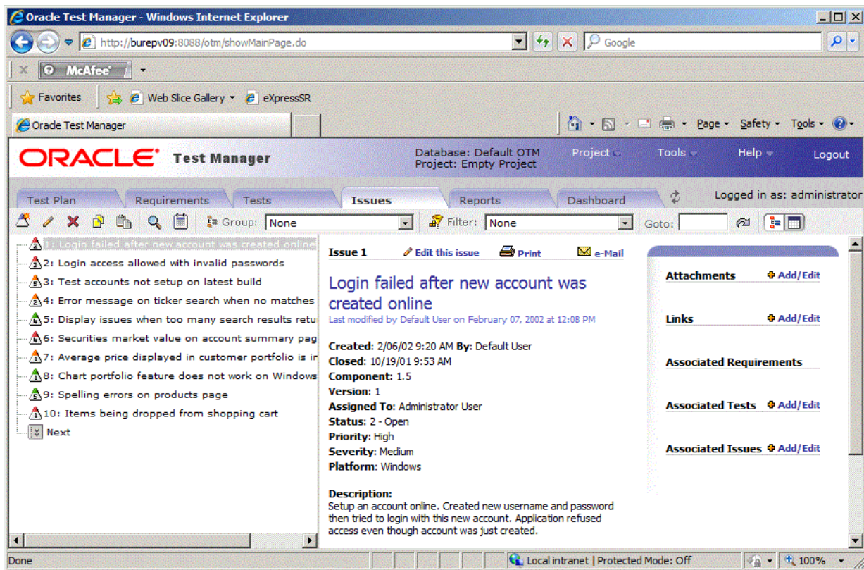
Figure 2-27 Issues Tab
