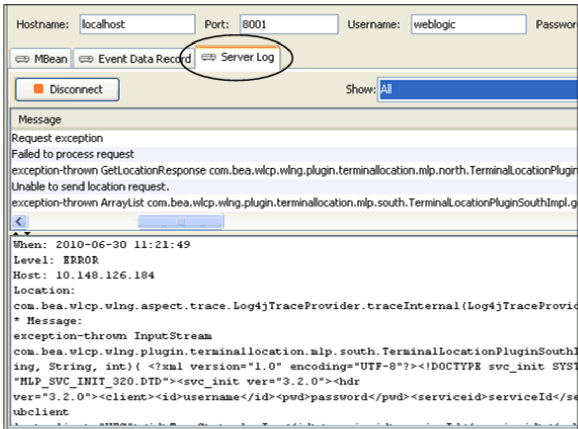
Figure 2–4 Server Log Message and Detail Panels
