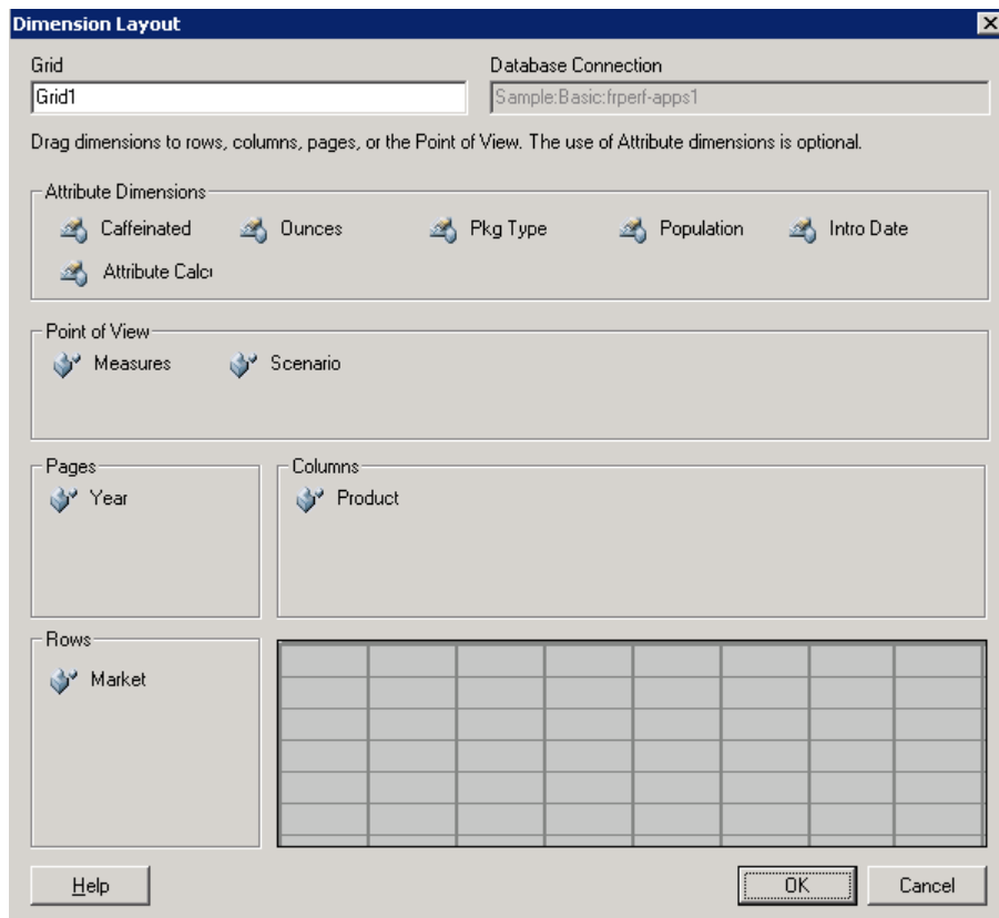
Figure 11 Dimension Layout Dialog Box
