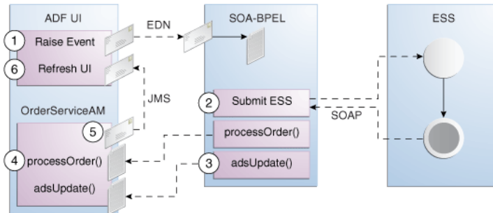
Figure 43–1 Technology Flow Diagram (with Optional Oracle Enterprise Scheduler Job Submission)
