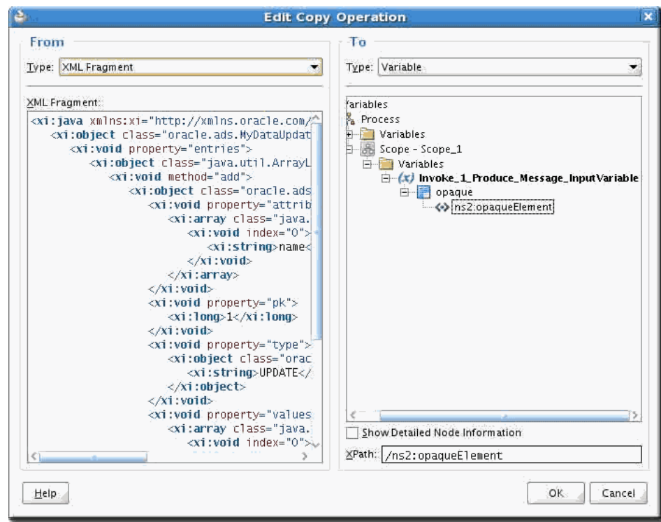
Figure 41–10 XML Fragment Copy Operation
