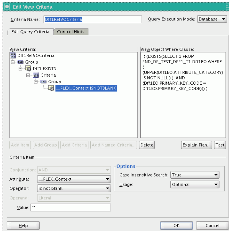
Figure 22–28 Edit Query Criteria Tab of View Object View Criteria Definition
