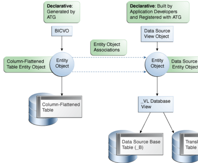
Figure 60–3 Declarative BICVO Based on Single Data Source View Object, Single Data Source Entity Object
