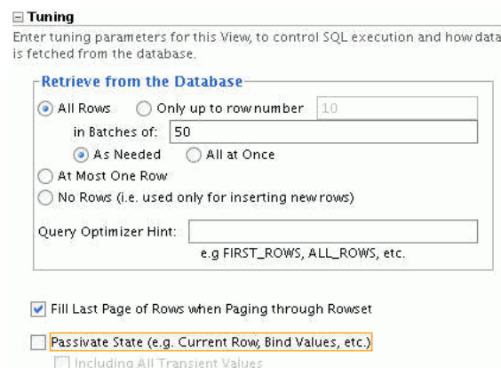
Figure 58–8 View Object Editor — Tuning
