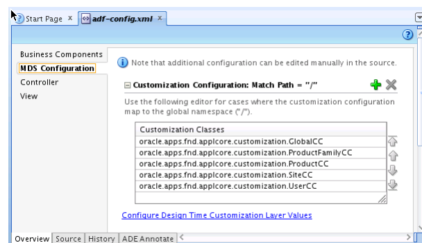
Figure 62-2 adf-config.xml — Customization Classes
