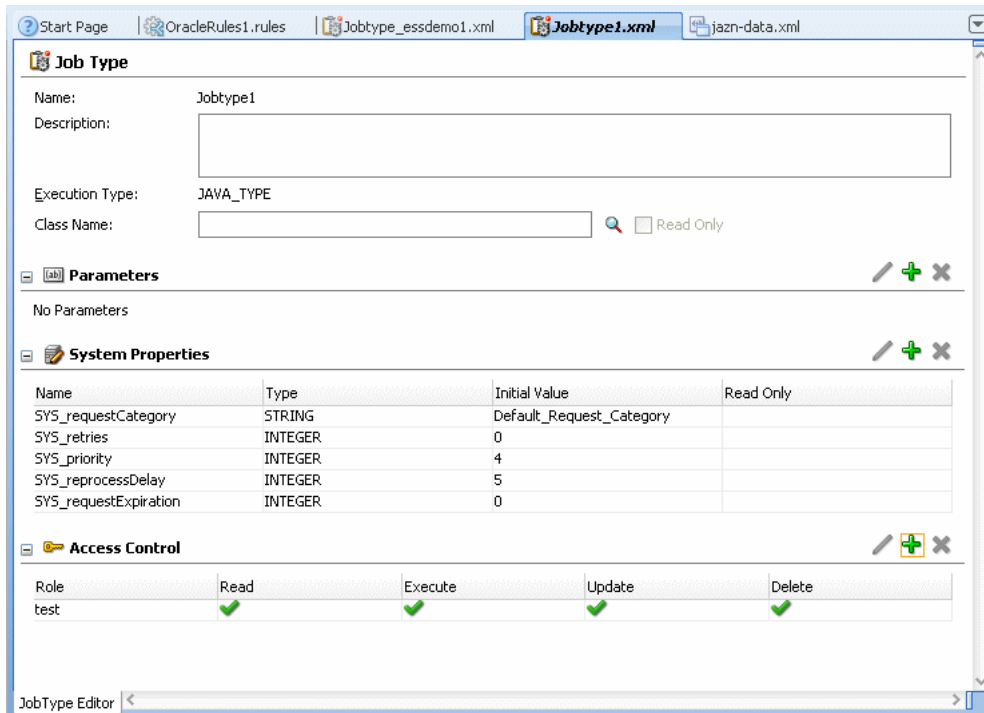
Figure 64–2 Security Roles for Oracle Enterprise Scheduler Metadata
