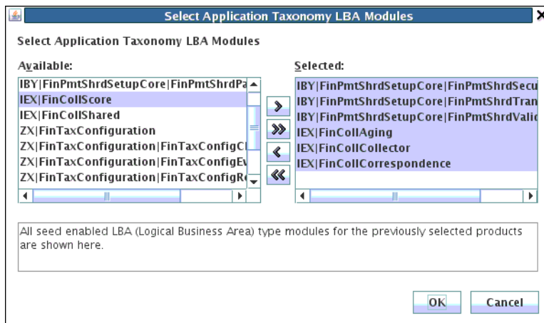
Figure 56–12 Selecting Application Taxonomy LBA Modules
