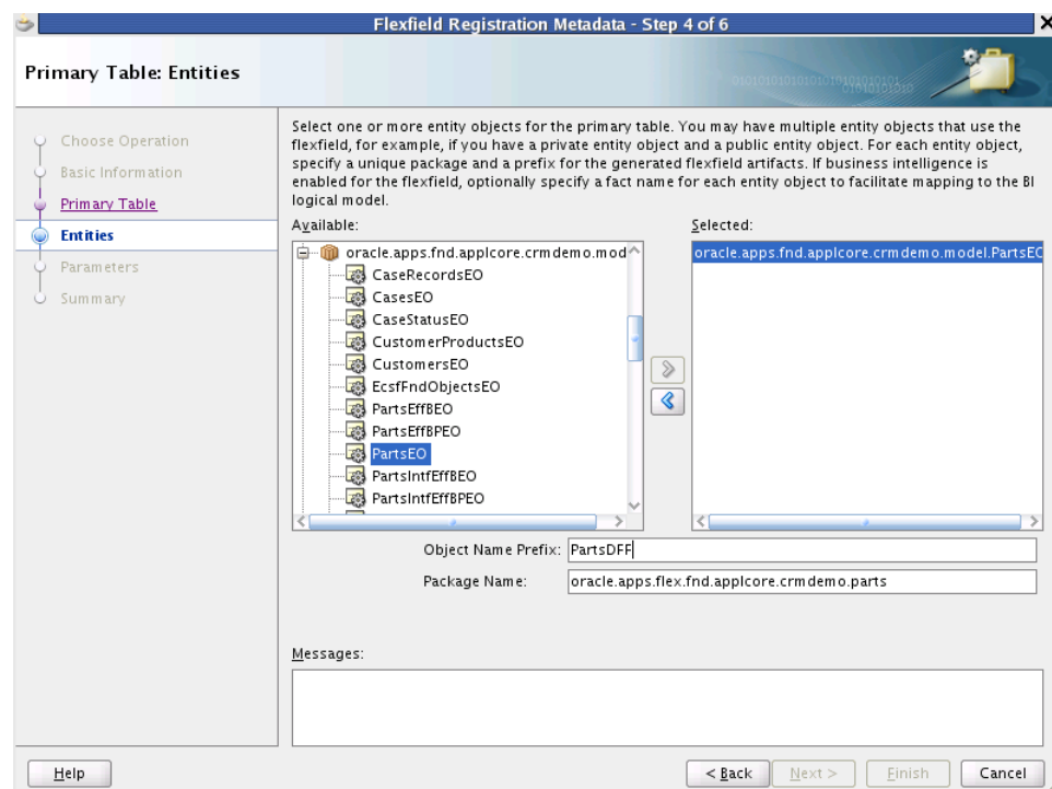
Figure 22-4 Flexfield Registration Metadata Wizard — Entities Page
