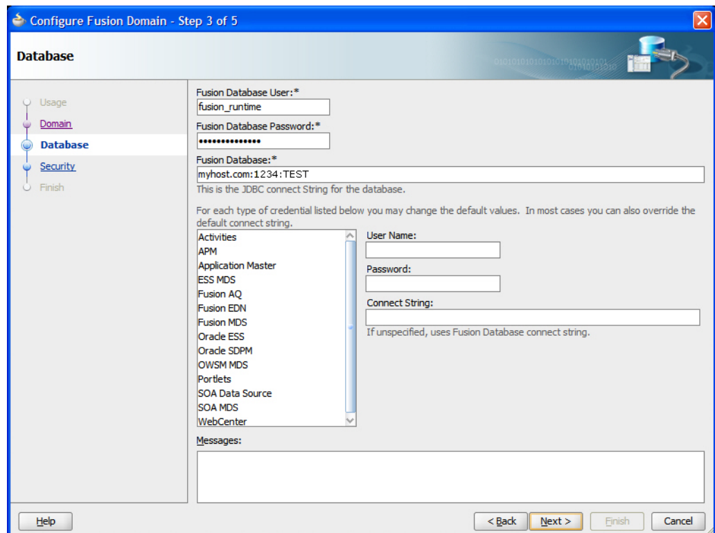
Figure 2–23 Configuring the Database
