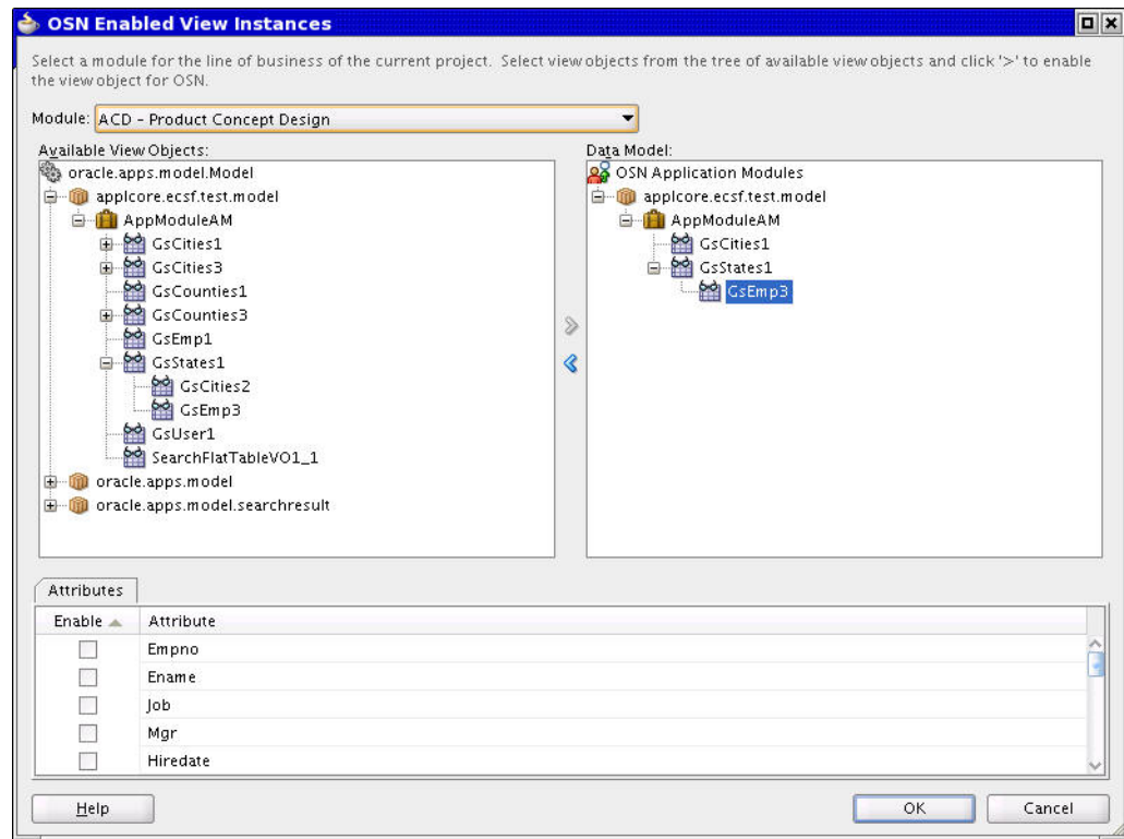
Figure 65–1 OSN Enabled View Instances Wizard
