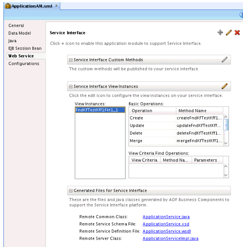
Figure 25–12 Application Module Service Interface Properties
