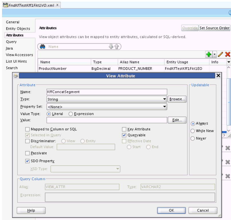
Figure 25–9 Adding a Transient Attribute to the Master View Object
