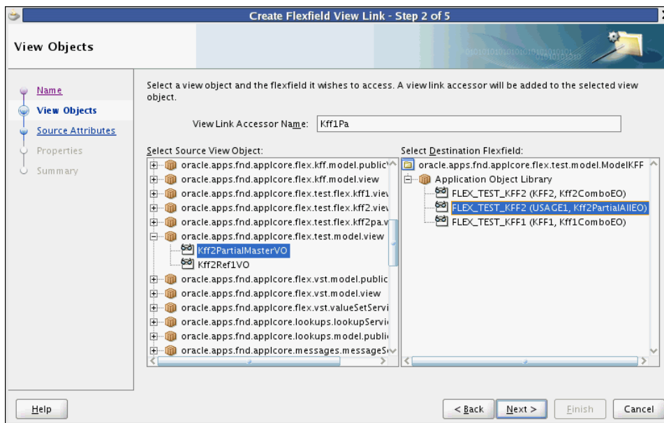
Figure 25–18 Create Flexfield View Link Wizard — View Objects Page
