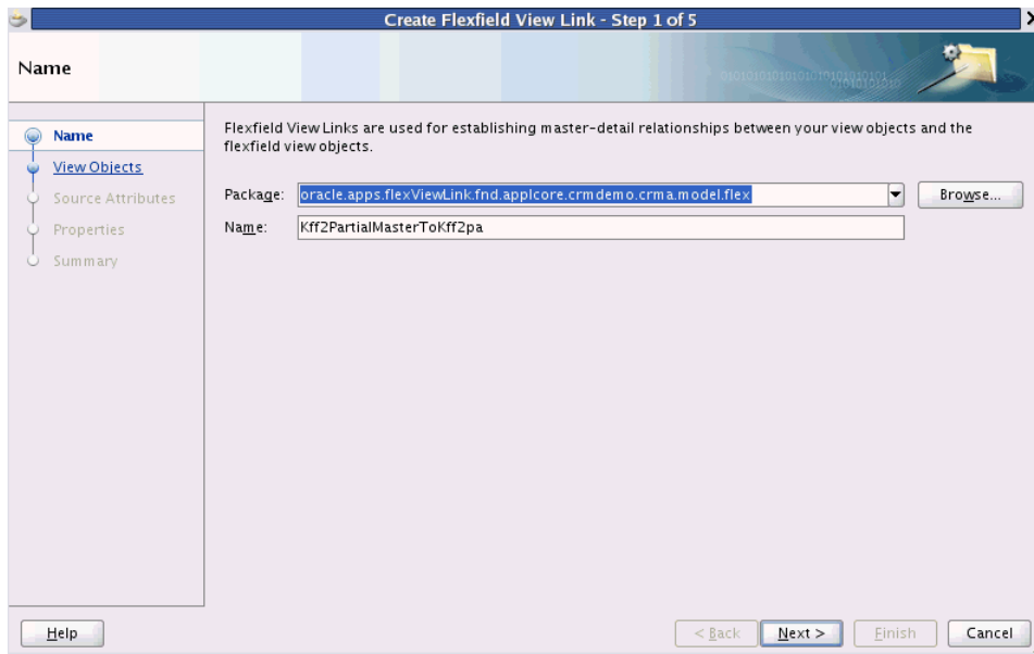
Figure 25–17 Create Flexfield View Link Wizard — Name Page
