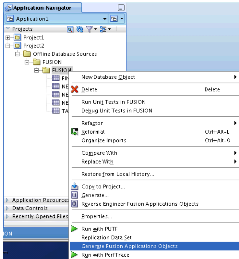
Figure 57-9 Deploying Offline Schema Object
