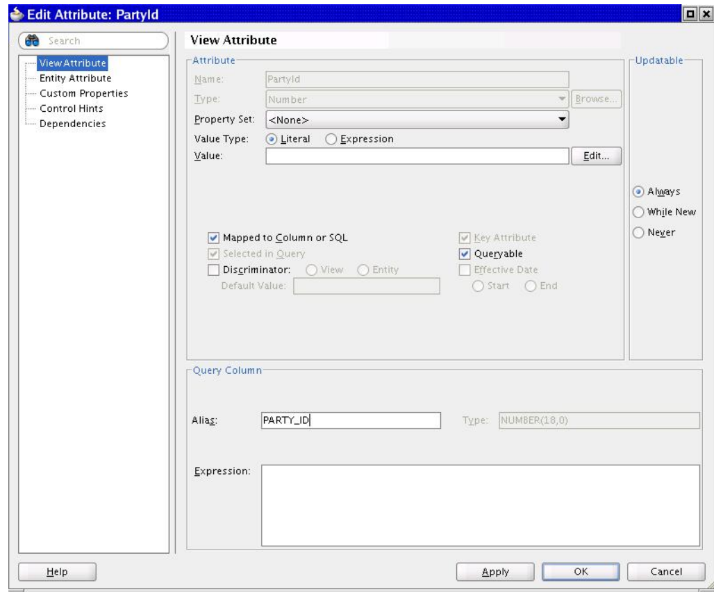
Figure 28–8 Changing the Alias Value in the Attribute Editor
