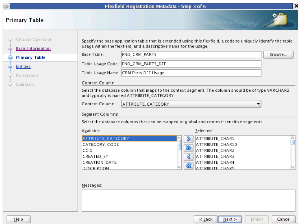
Figure 22–3 Flexfield Registration Metadata Wizard — Primary Table Page
