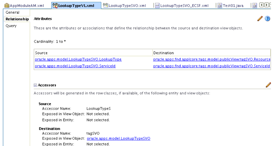
Figure 14–35 View Link Example
