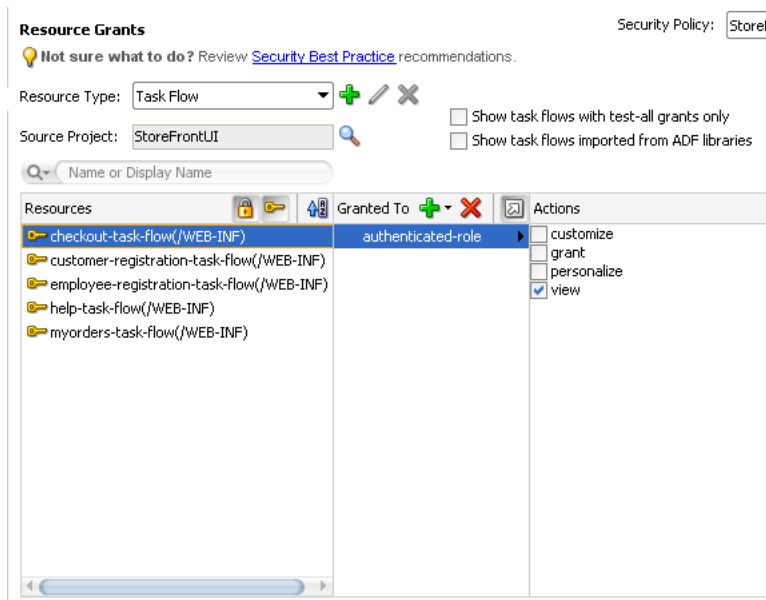
Figure 50–2 Granting to authenticated-role in the Overview Editor
