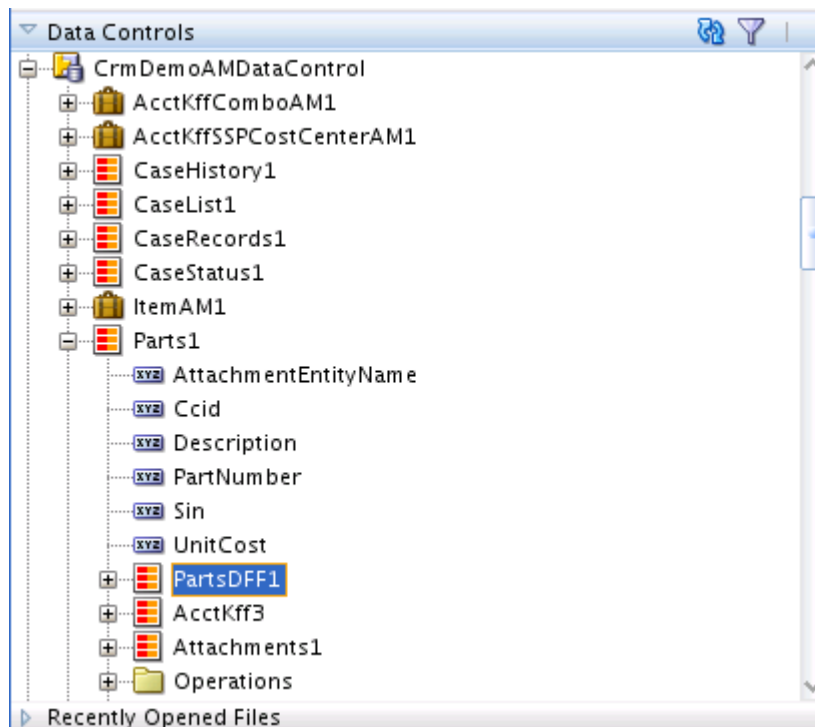
Figure 22–21 Flexfield View Object Nested Under Master View Object
