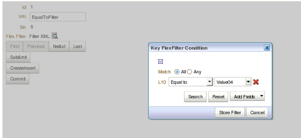
Figure 25–25 Table-Based Code-Combination Filter User Interface
