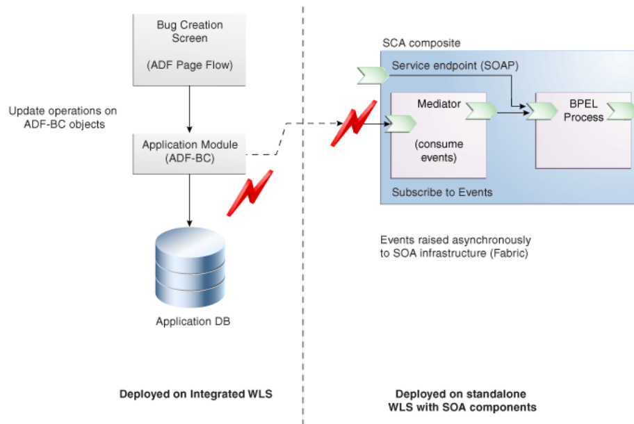
Figure 33-1 Mediator Service Component Subscribes to an Event and Invokes BPEL Service Component
