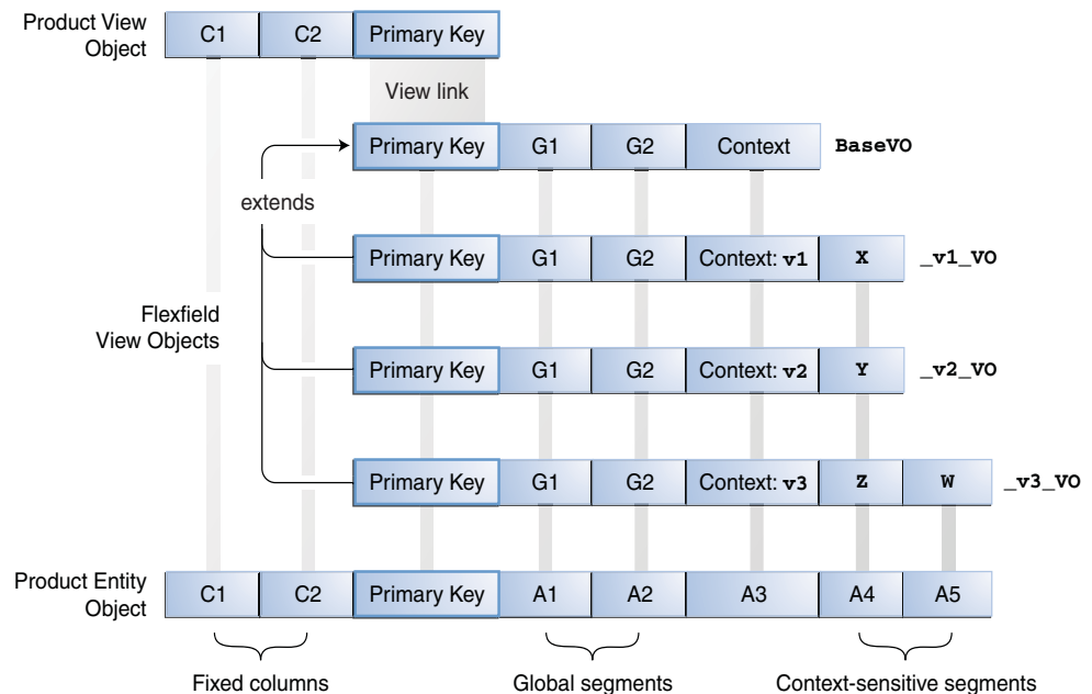
Figure 22–13 Descriptive Flexfield Modeled as ADF Business Components Component
