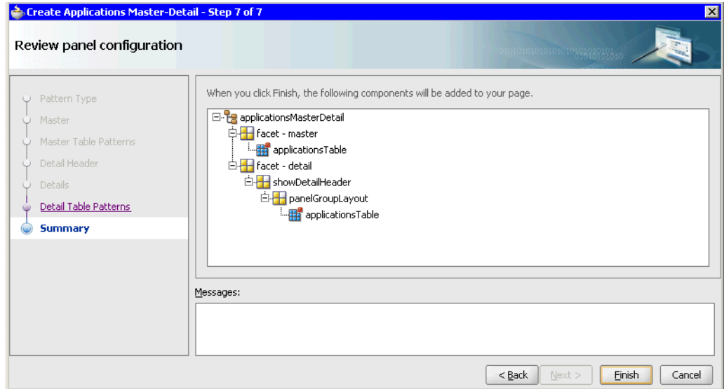
Figure 17-22 Reviewing the Panel Configuration
