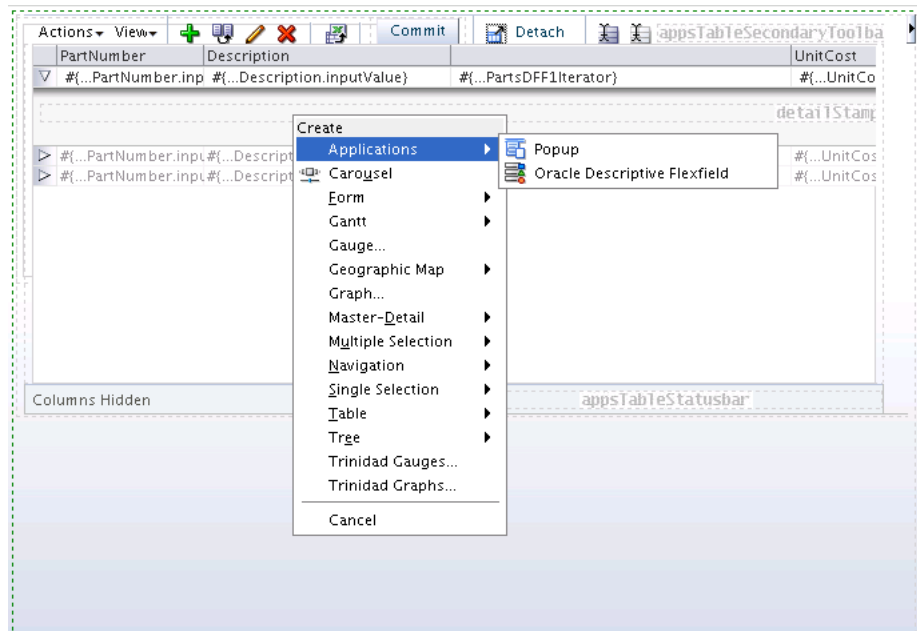
Figure 22–24 Descriptive Flexfield Dropped into a Detail Region
