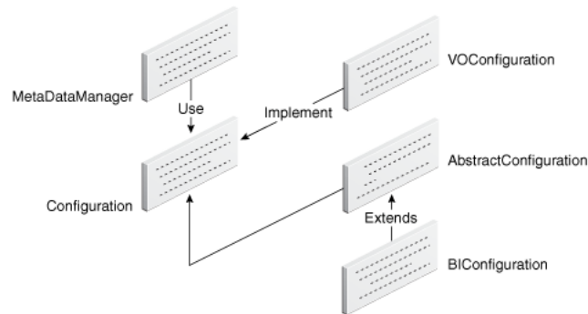
Figure 32–5 Runtime Architecture with Configuration Interface
