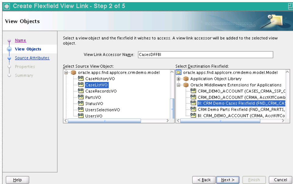
Figure 22–31 Create Flexfield View Link Wizard — View Objects Page
