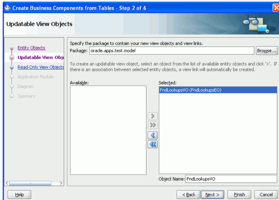
Figure 2–50 Create Business Components from Tables — Updatable View Objects
