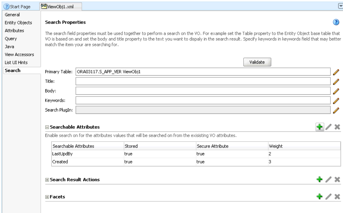
Figure 28–6 Search Page for Configuring Search Properties of View Object Attributes
