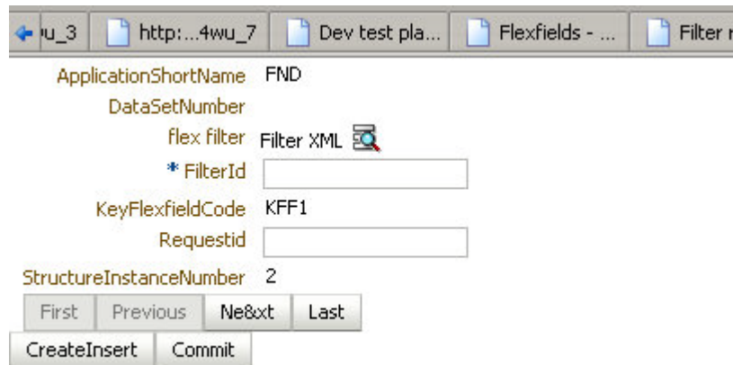
Figure 25–27 Form-Based Report Submission Code-Combination Filter UI
