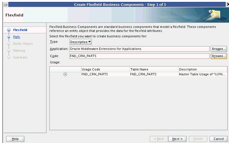
Figure 22–14 Create Flexfield Business Components Wizard — Flexfield Page
