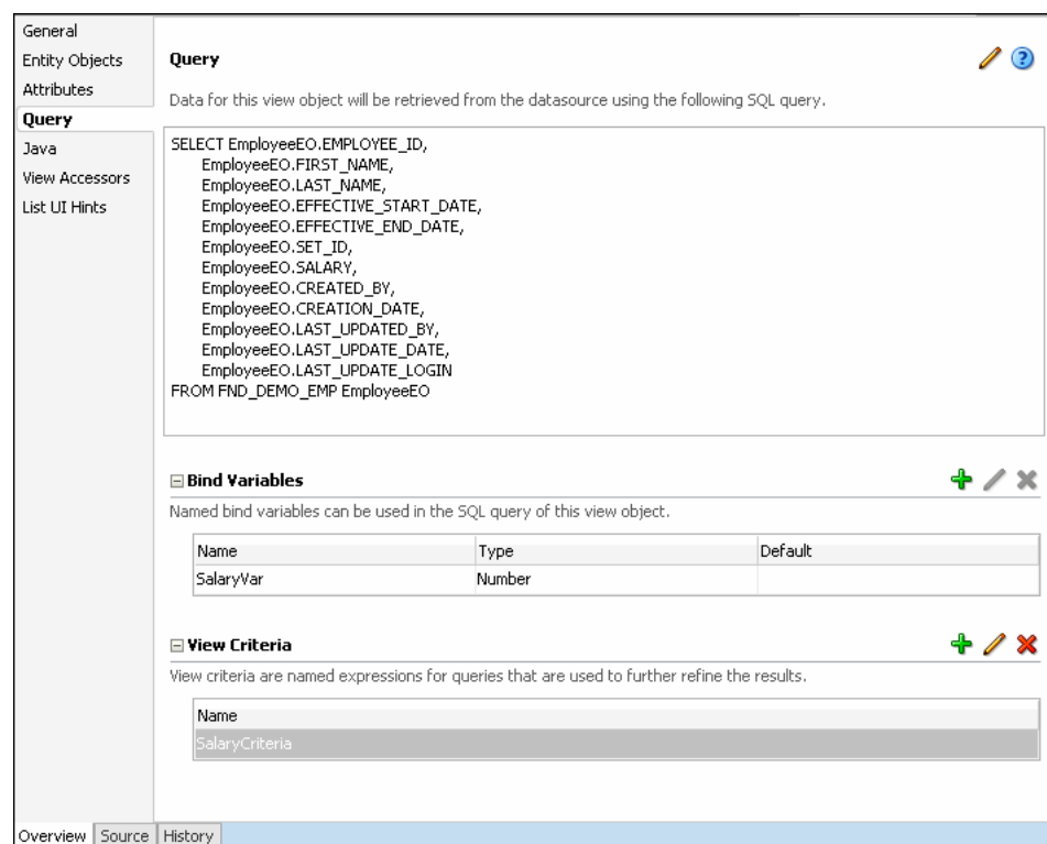
Figure 19–75 Bind Variables and View Criteria Settings
