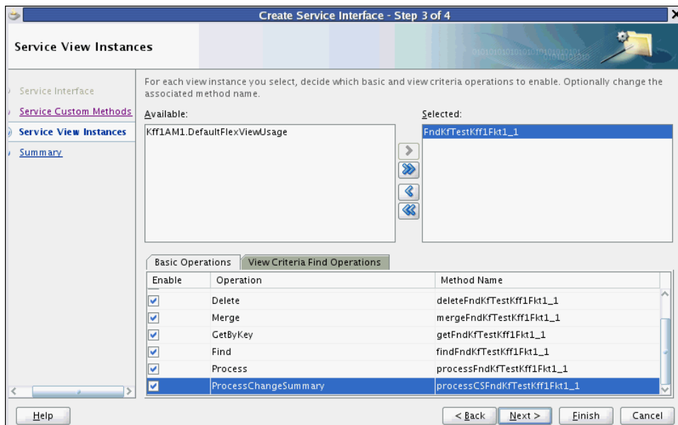
Figure 25–11 Create Service Interface Wizard — Service View Instances Page
