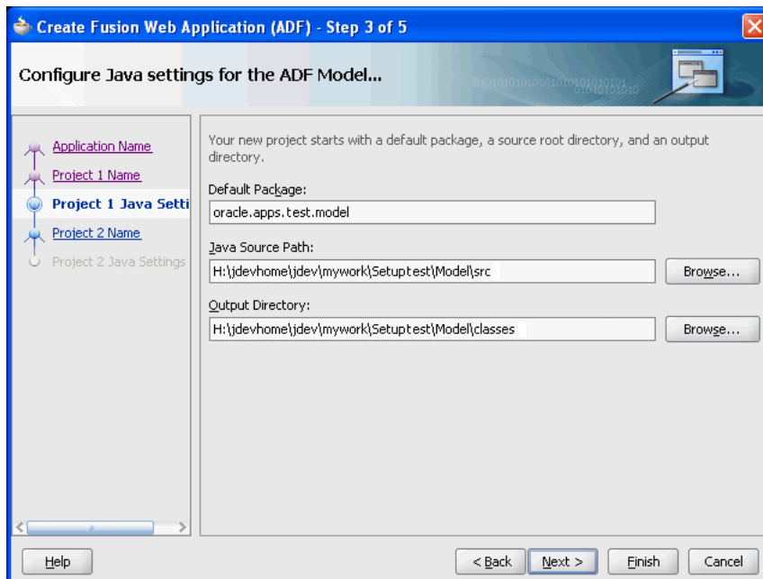
Figure 2–45 Configuring Java Settings for the ADF Model
