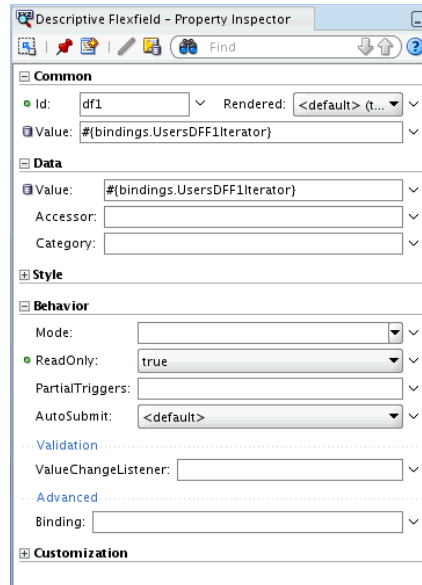
Figure 22–27 Descriptive Flexfield Property Inspector
