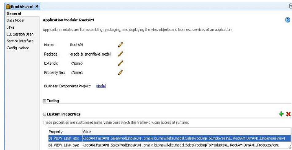
Figure 22–32 Custom Properties for Business Intelligence-Enabled Application Module
