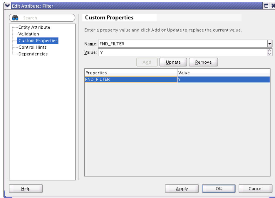
Figure 25–21 Edit Filter Attribute — Custom Properties Page
