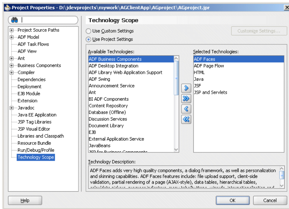
Figure 15–7 Adding the ADF Faces and ADF Page Flow Technologies to the Client Application
