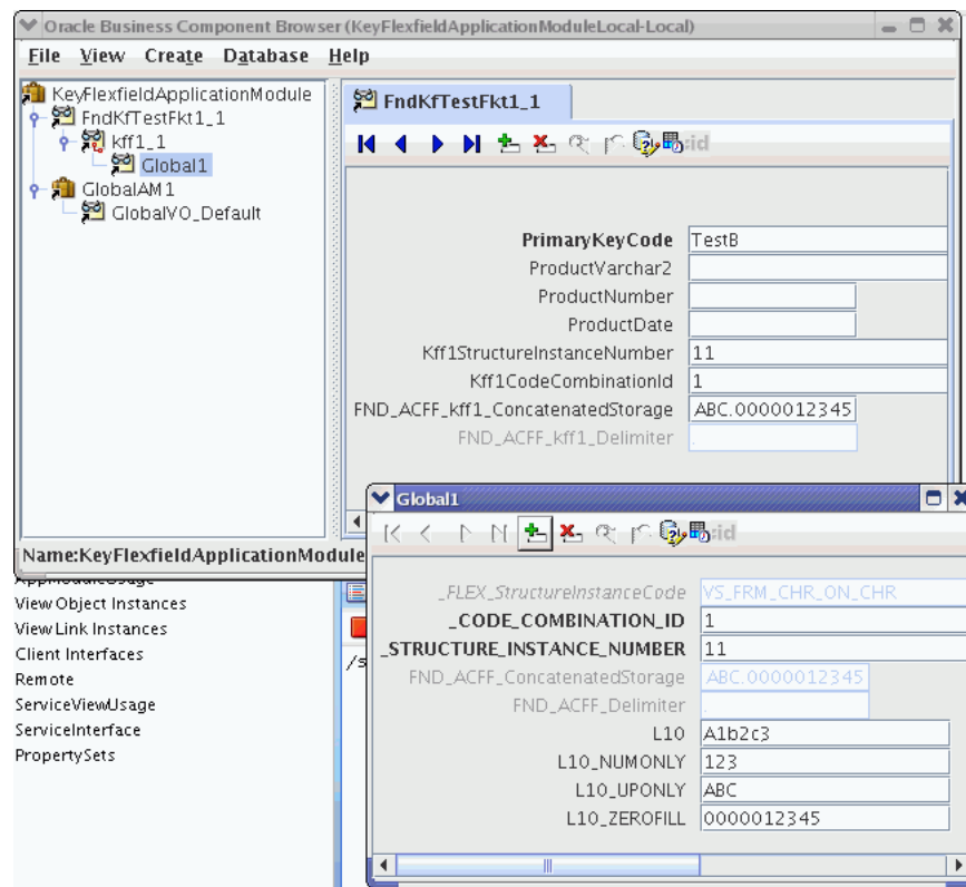
Figure 25–5 Business Component Browser View of Flexfield Row with SIN = 11
