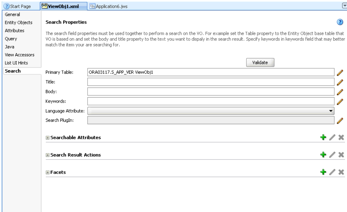
Figure 28–3 Search Page for Configuring Search Properties of View Objects
