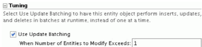
Figure 58-1 Entity Object Editor — Tuning
