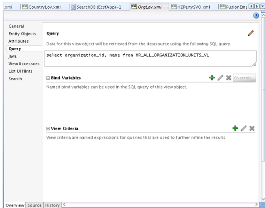
Figure 32–9 Querying a View Object
