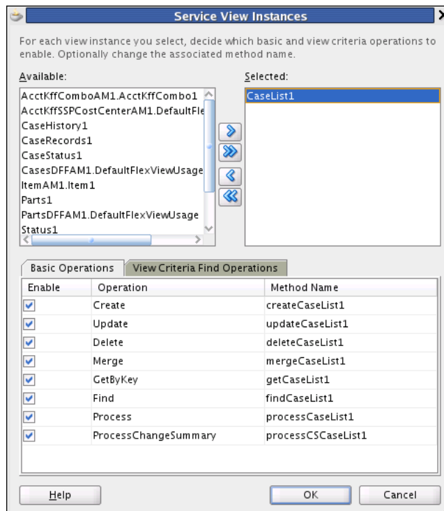
Figure 22–35 Selecting Master View Object Instances to Expose
