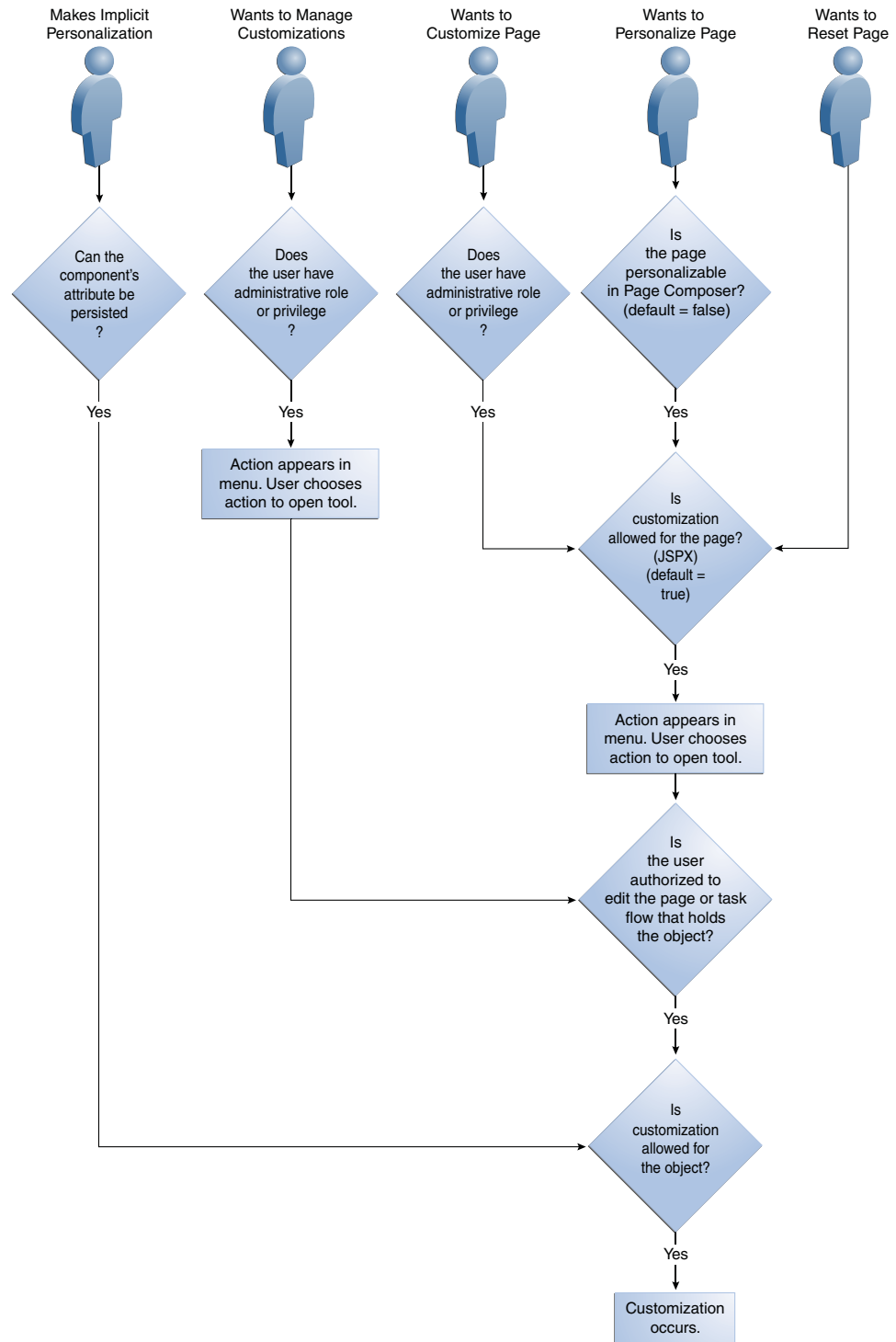
Figure 62–3 Runtime Effects of Customization Settings
