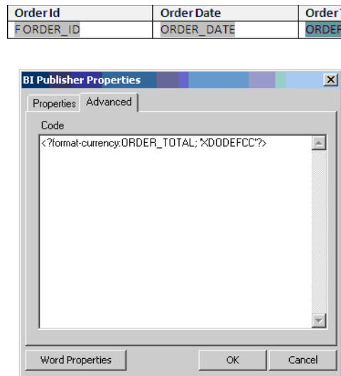
Figure 20–24 Entering Currency Code in Oracle BI Publisher Properties
