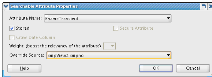
Figure 28–7 Searchable Attribute Properties Dialog
