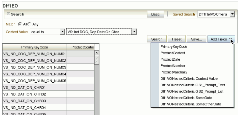
Figure 22–30 Descriptive Flexfield Search Form UI
