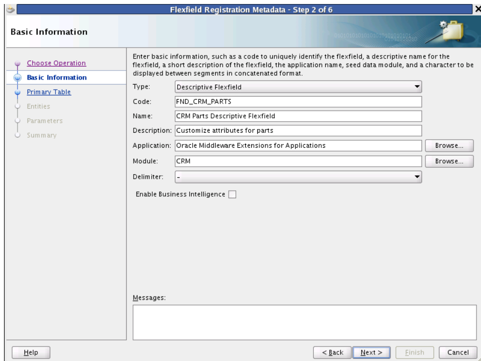
Figure 22–2 Flexfield Registration Metadata Wizard — Basic Information Page
