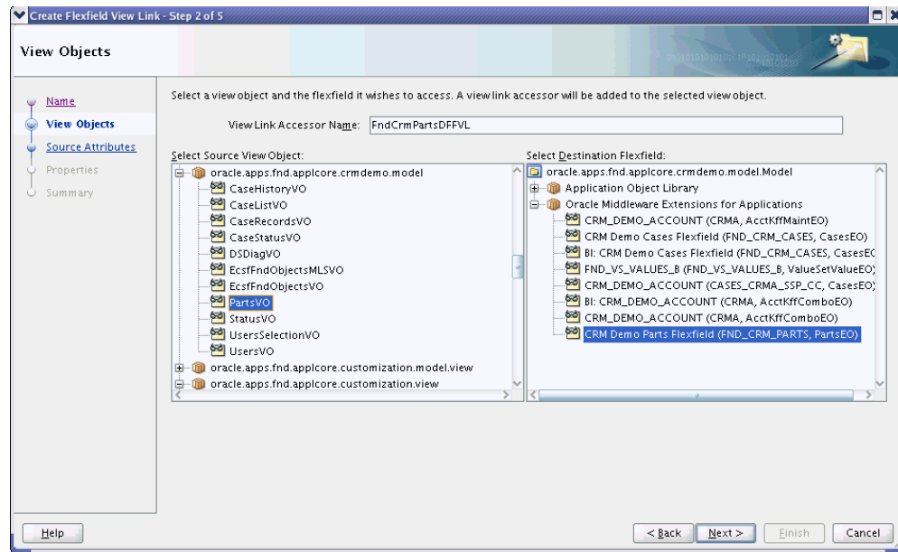
Figure 22–18 Create Flexfield View Link Wizard — View Objects Page
