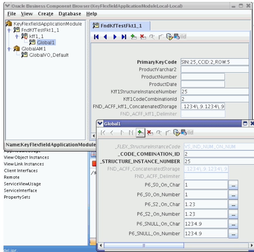
Figure 25–6 Business Component Browser View of Flexfield Row with SIN = 25
