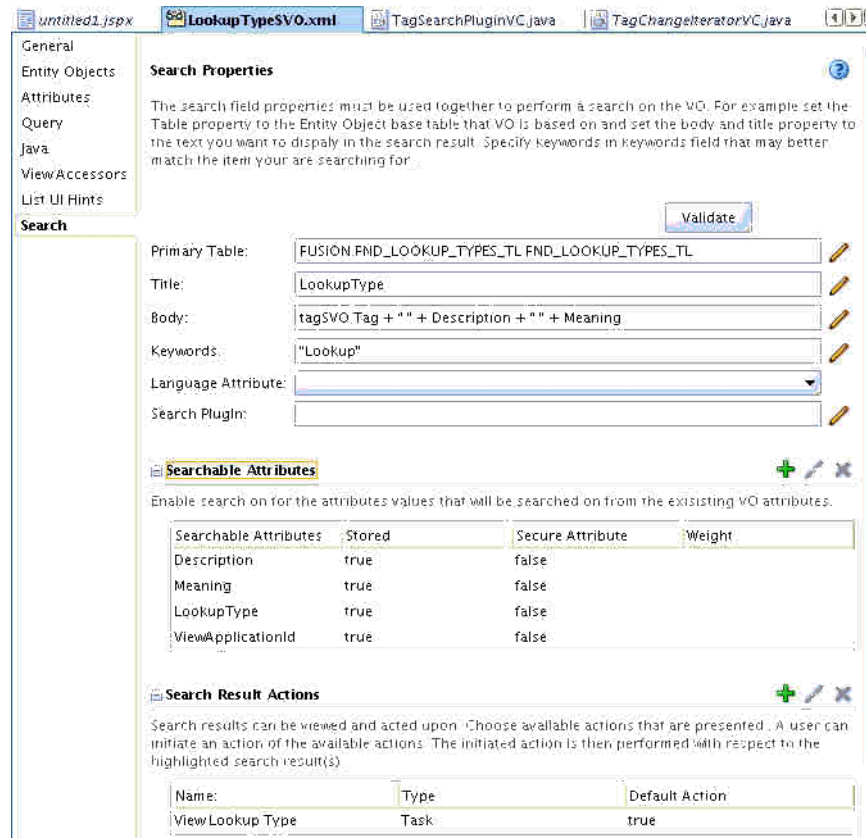
Figure 14–34 Tags - Lookup Types
