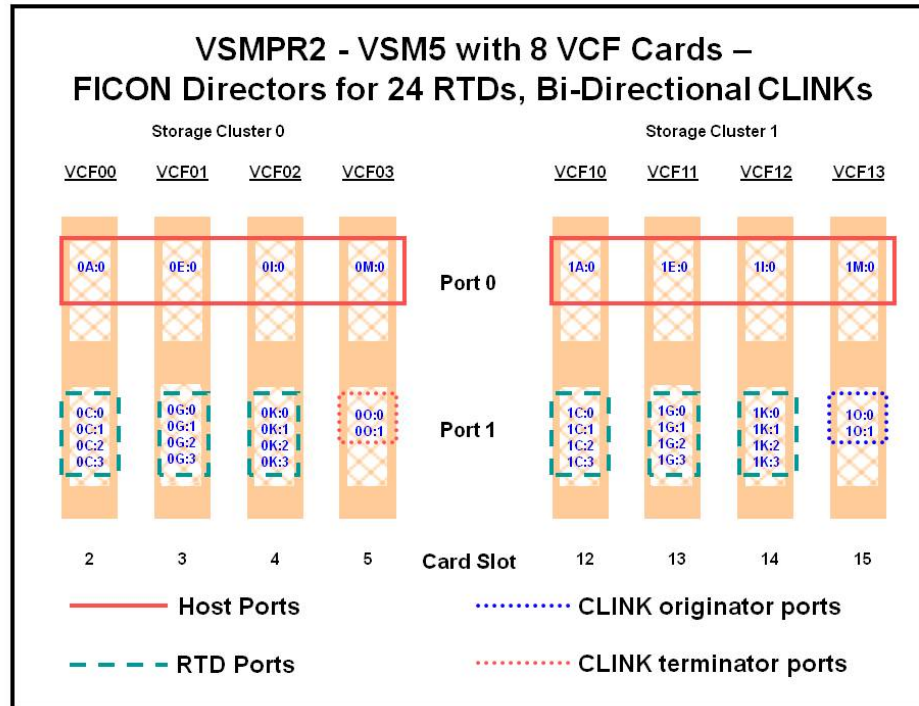
FIGURE A-11 VSM2R - VSM5 with 8 VCF Cards, 8 Host Ports, FICON Directors for 24 RTDs, 4 CLINKs
