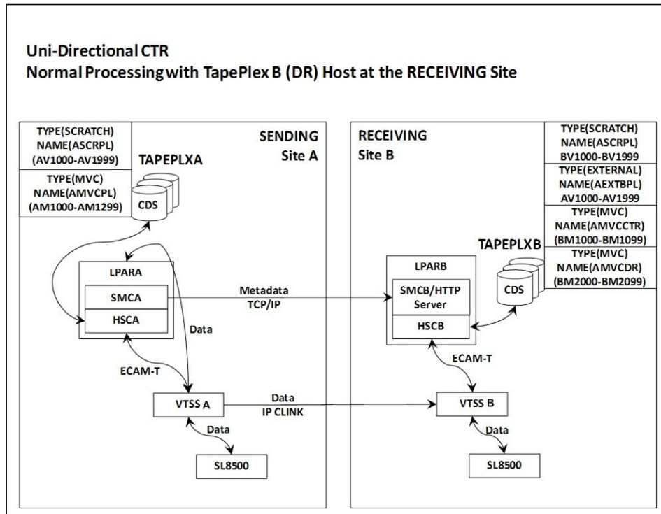
FIGURE 4-3 CTR Configuration
