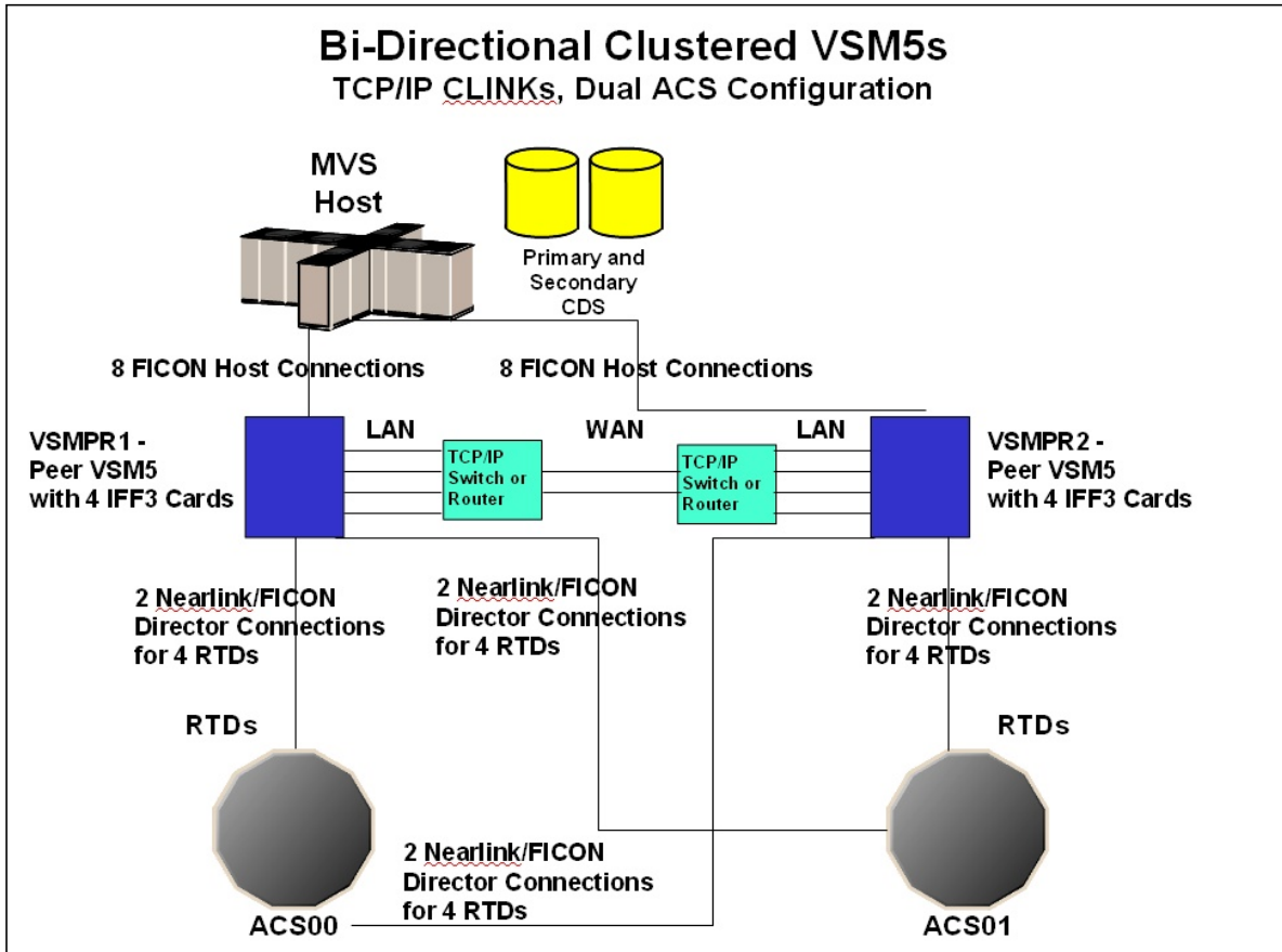
FIGURE A-22 shows an example of a VSM5 to VSM5 Cluster with TCP/IP CLINKs.
