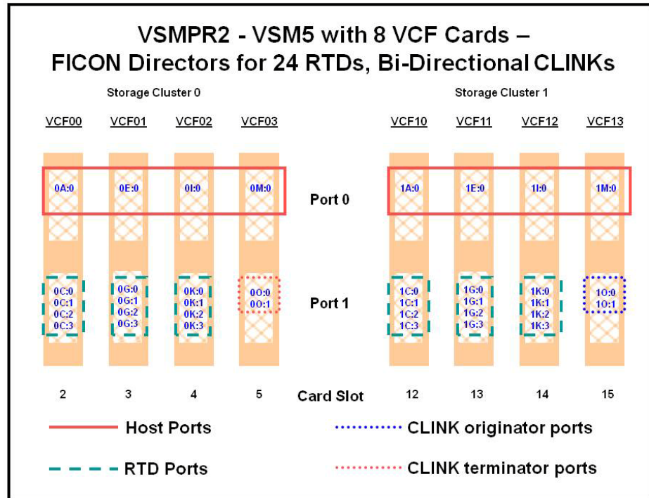
FIGURE A-11 VSMR2 - VSM5 with 8 VCF Cards, 8 Host Ports, FICON Directors for 24 RTDs, 4 CLINKs
