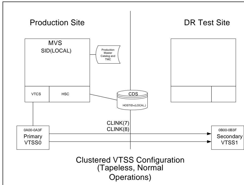
FIGURE 7-13 Primary/Secondary Clustered VTSS Configuration (Tapeless) - Before Running the DRTEST Utility
